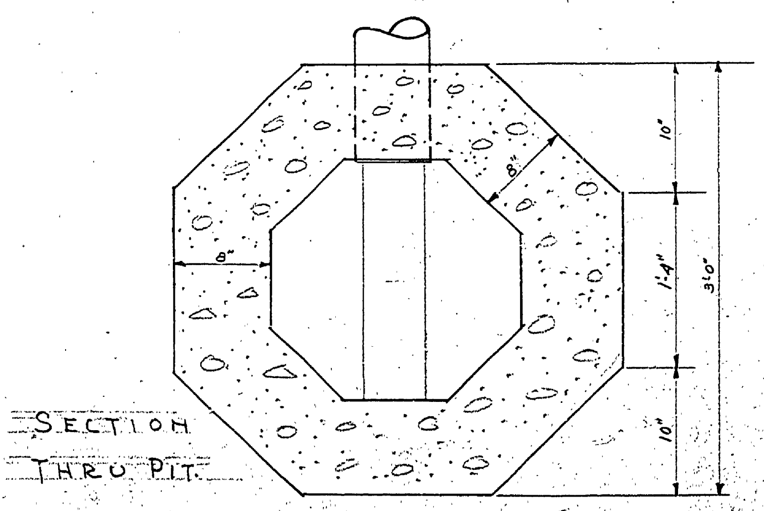
DETAILS OF WASTE WATER SUMP SCALE: 1/2" = 1'-0"
