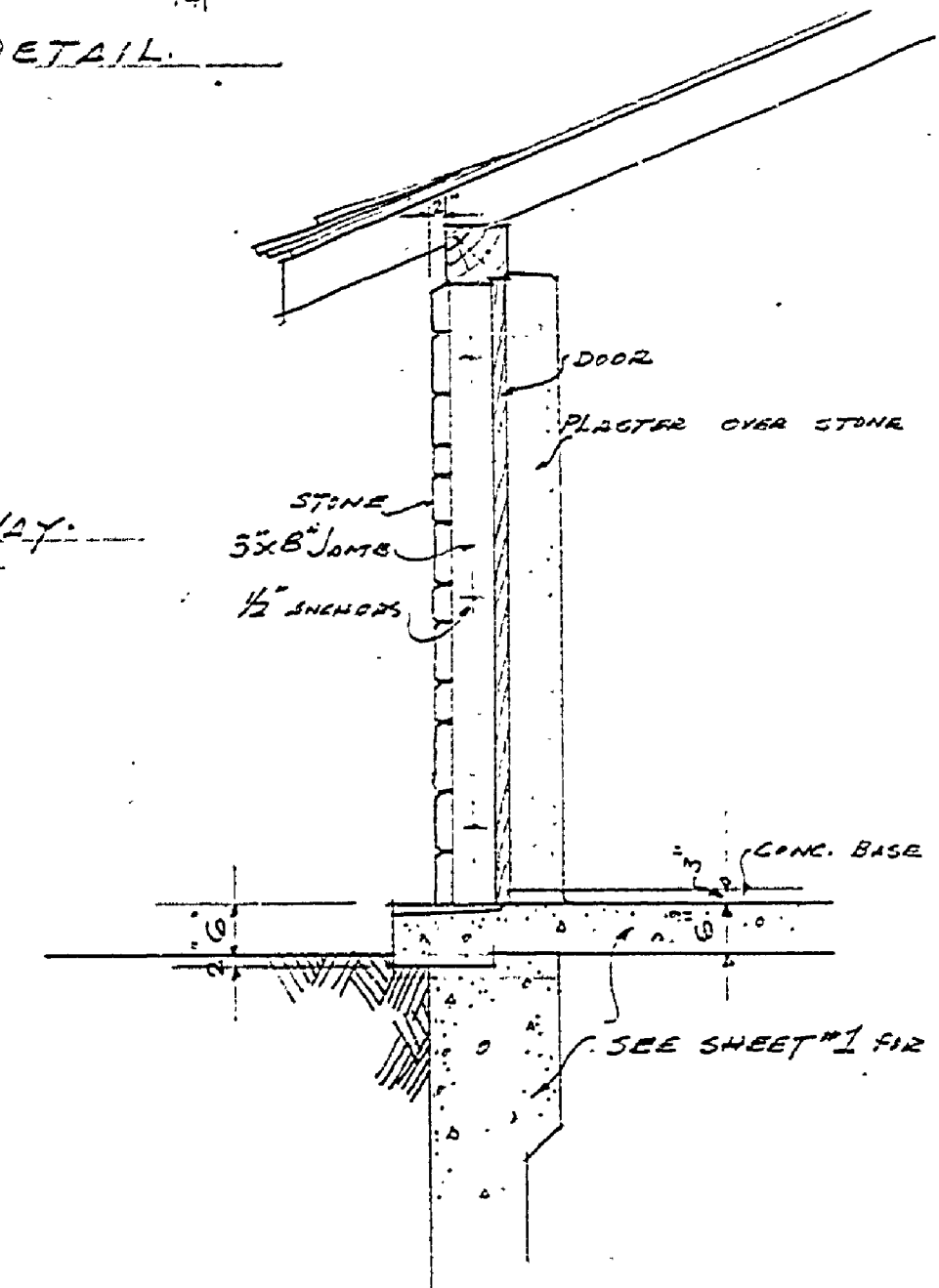
SEC. THRU ENTRANCE SCALE: 1/2" = 1'-0"
