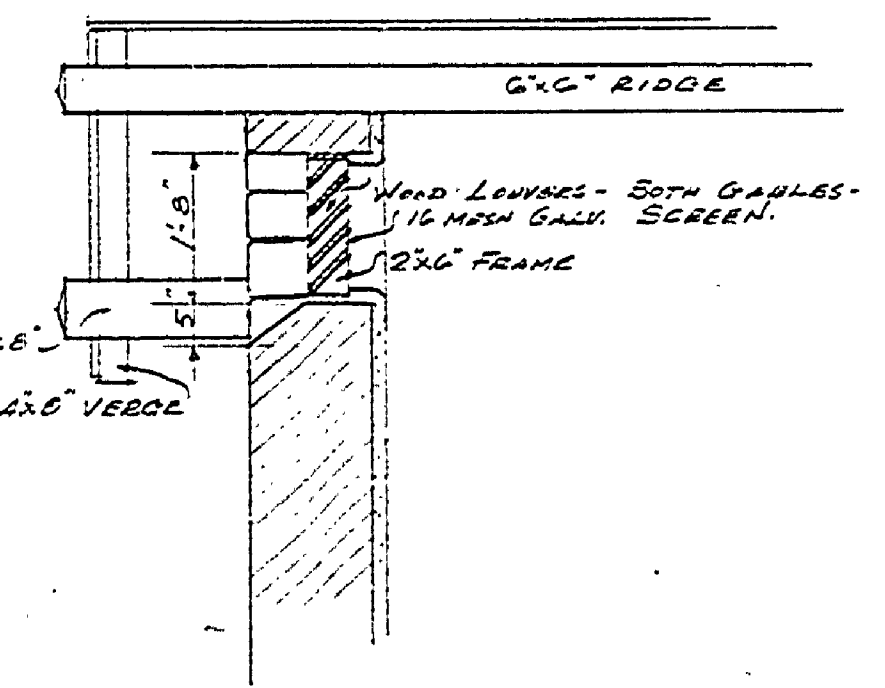
SEC. THRU LOUVERS 1/2" SCALE
