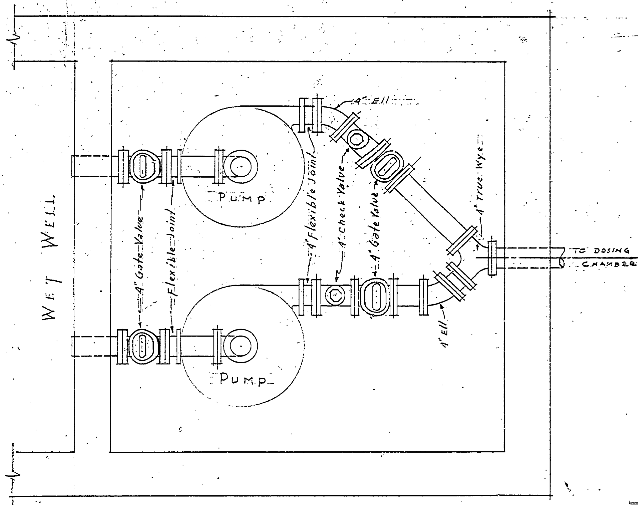
PUMPING STATION-PIPING LAYOUT
