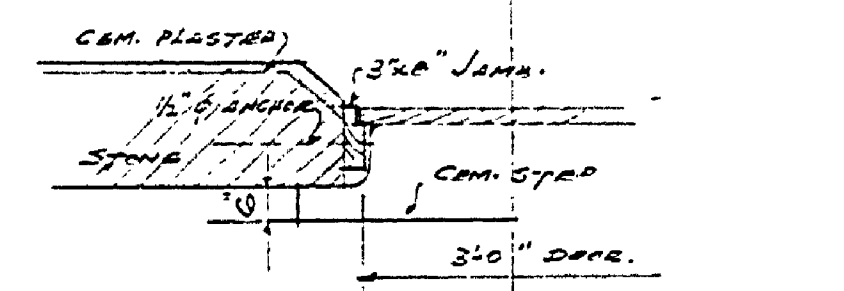
PLAN THRU DOOR WAY SCALE: 1/2" = 1'-0"
