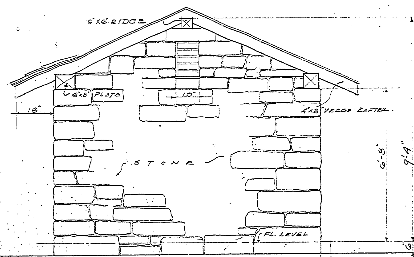
SOUTH ELEVATION SCALE: 1/2" = 1'-0"
