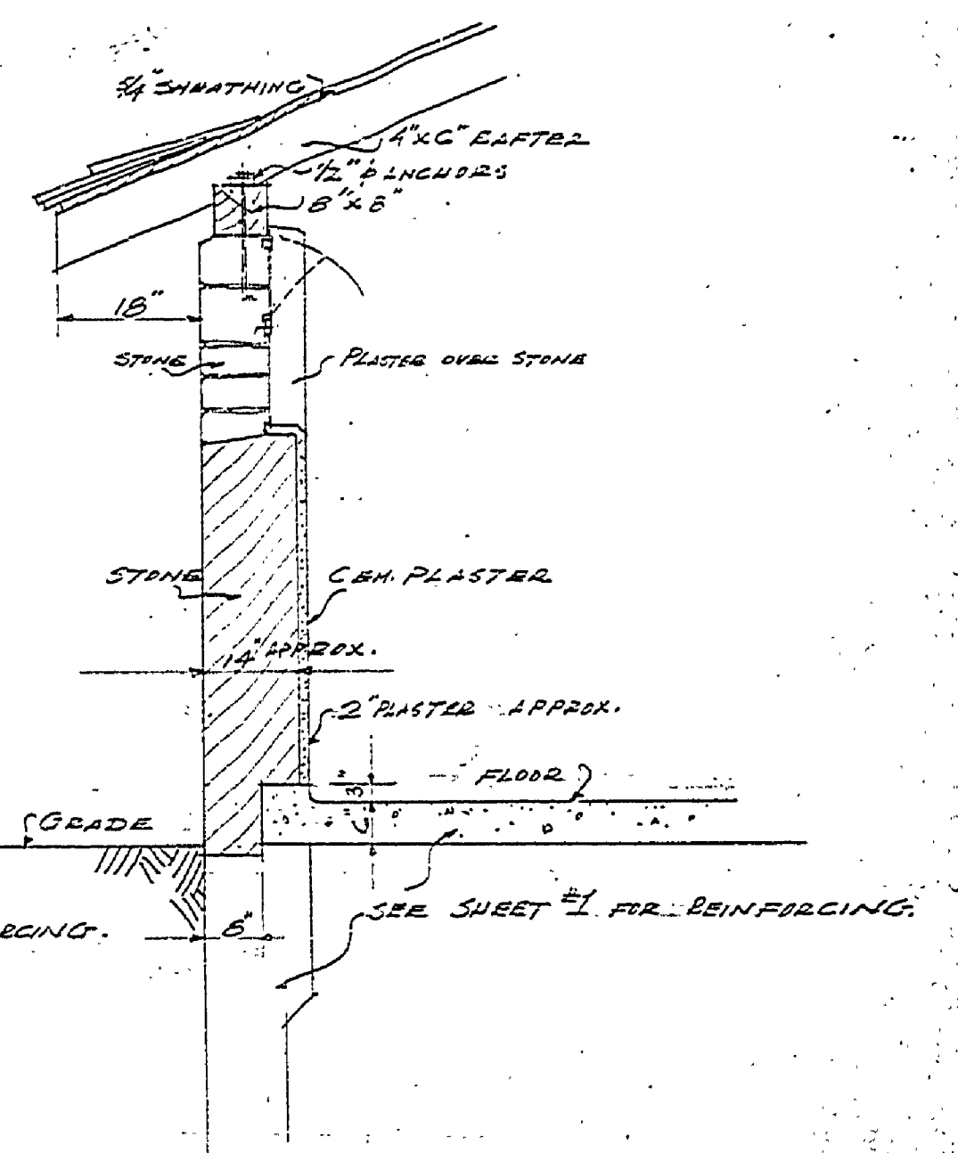
SEC. THRU WINDOW SCALE: 1/2" = 1'-0"
