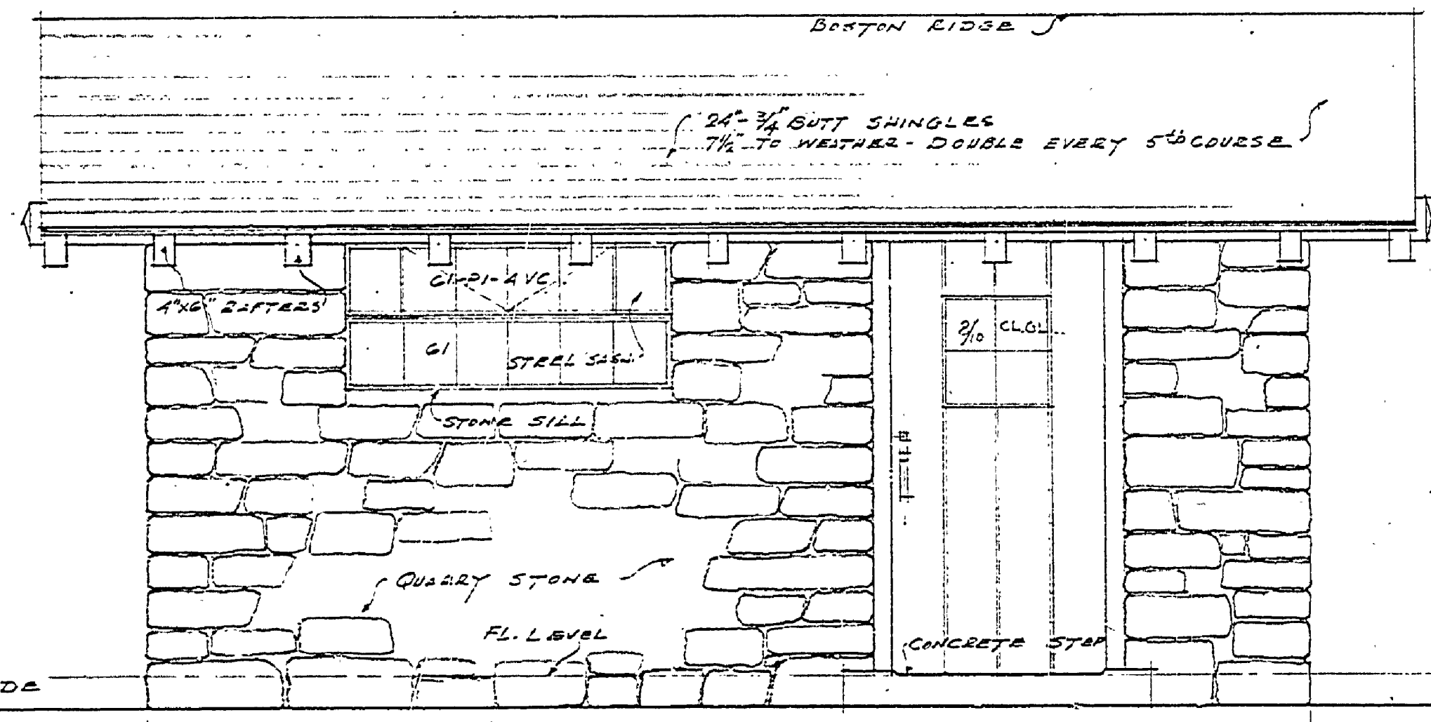
EAST ELEVATION SCALE: 1/2" = 1'-0"
