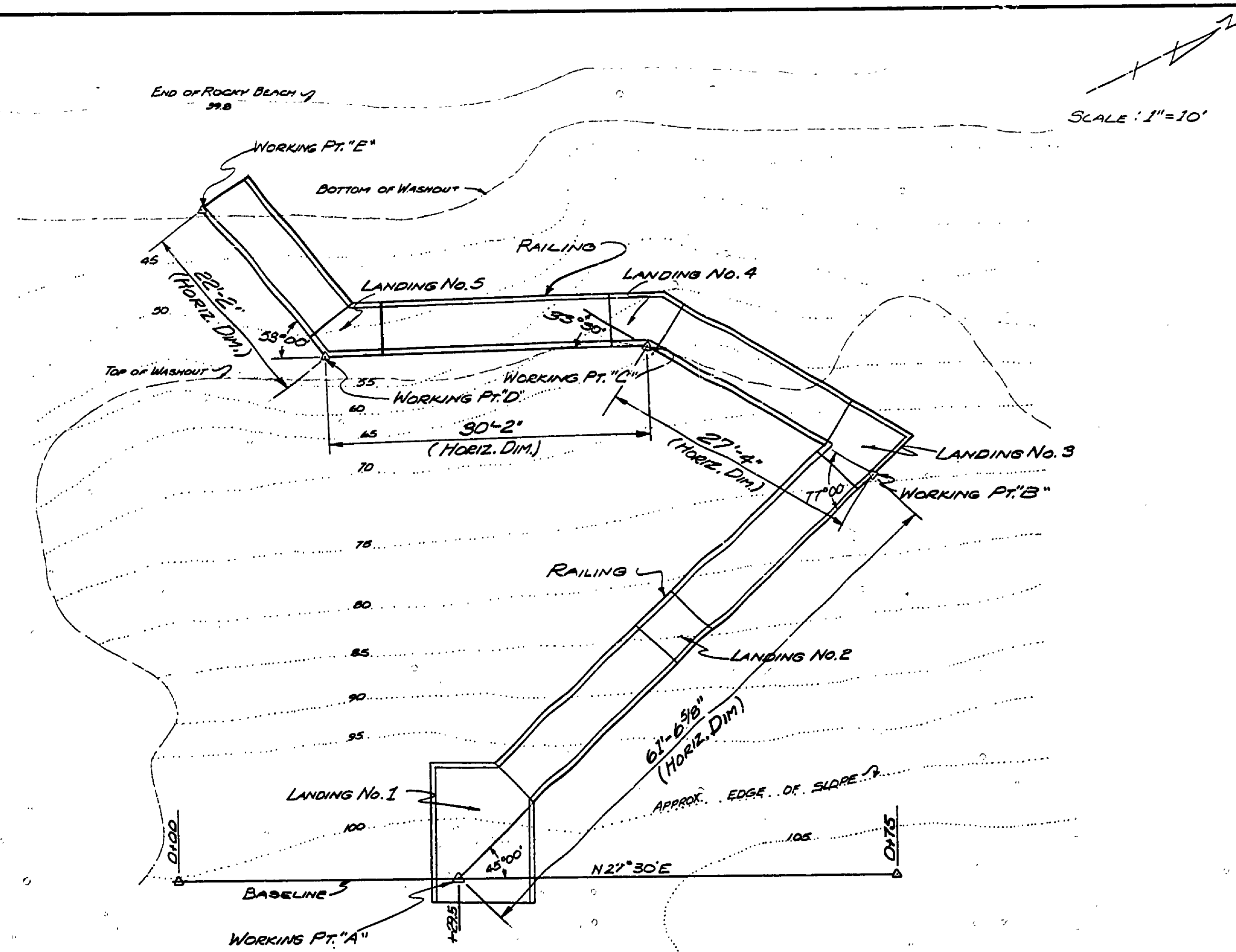
PLAN OF STAIRS 1"=10'
