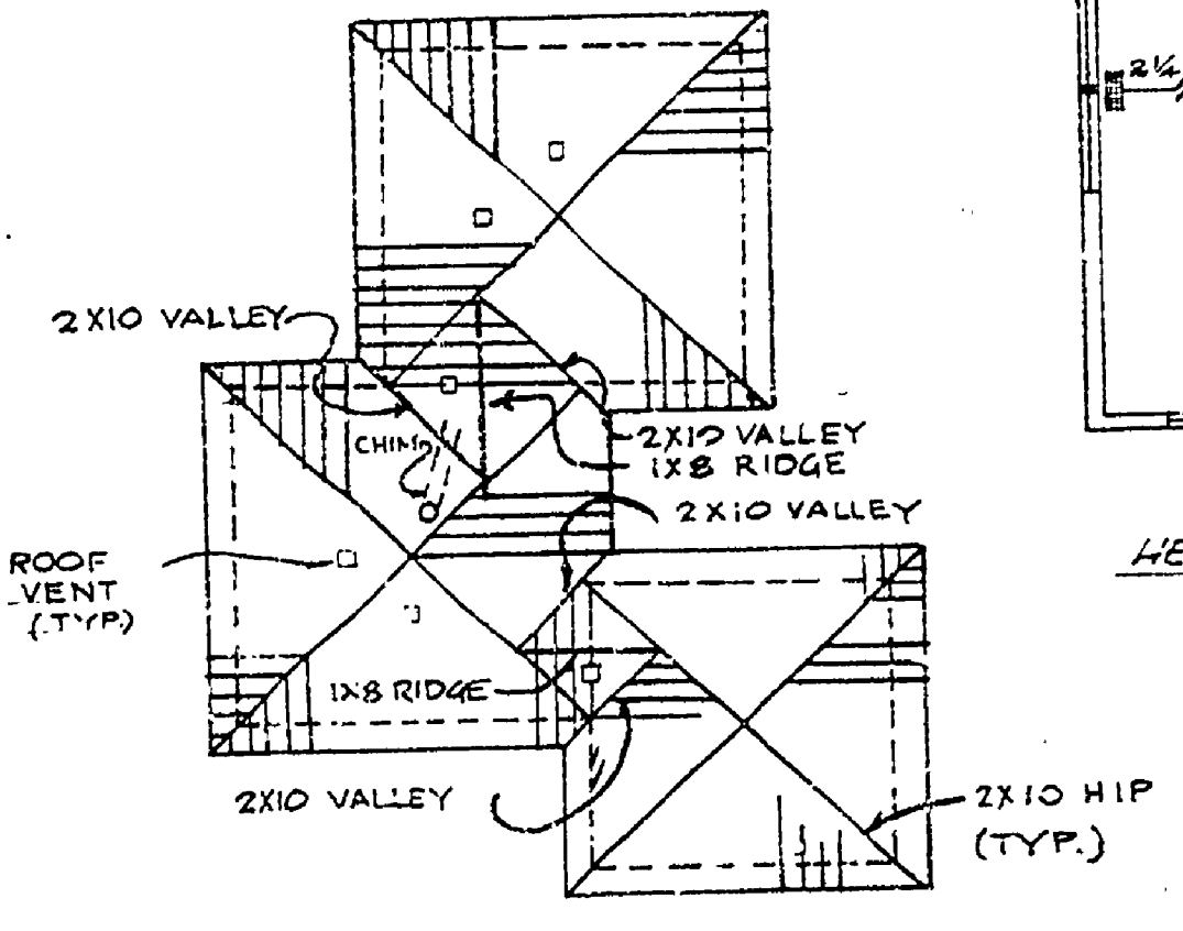
ROOF PLAN NO SCALE NOTE: ALL RAFTERS - 2X8-16\"/>
