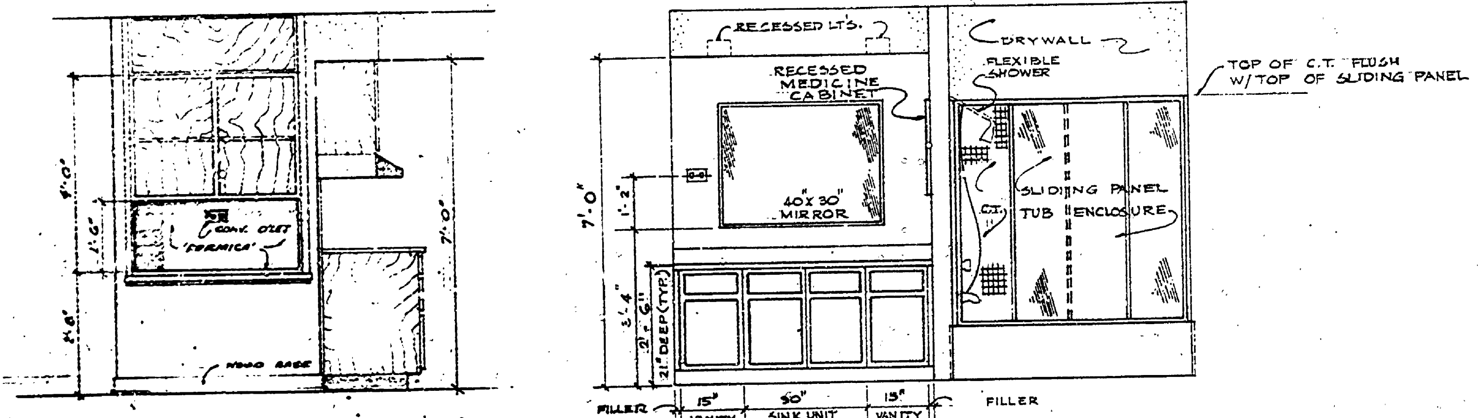
ELEVATION BATHROOM - #7 TUB & SHOWER SIDE SCALE: 1/2" = 1'-0"
