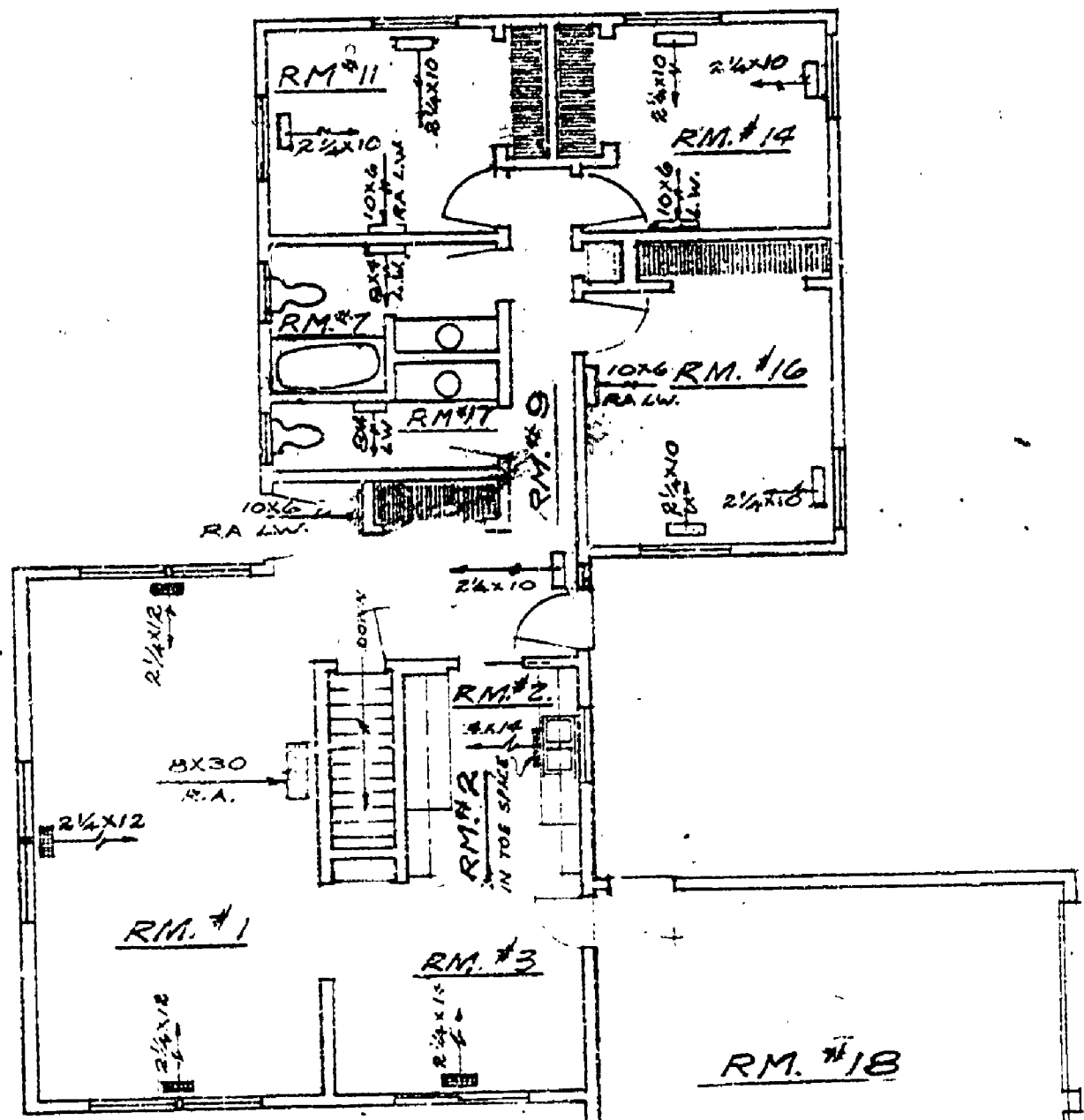
HEATING PLAN - 1ST FL. SCALE: 1/4" = 1'-0"
