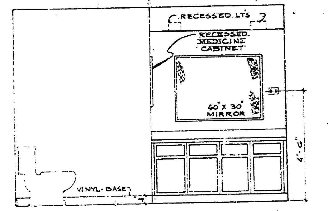
ELEVATION BATHROOM - #17 SCALE: 1/2" = 1'-0"
