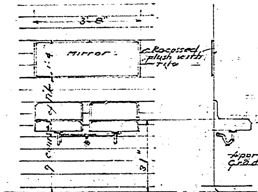
ELEVATION AT LAVATORY
