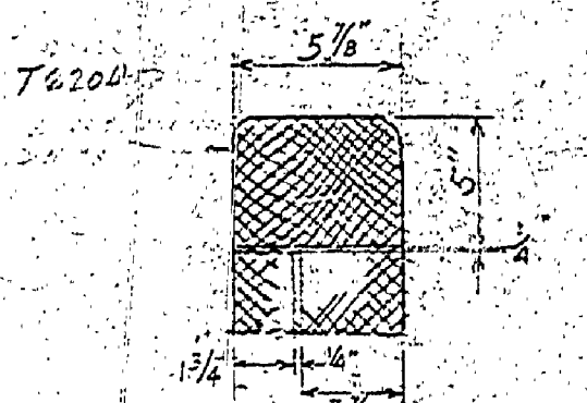
SECTION B-B TILE PARTITION Scale 1/2\"/>
