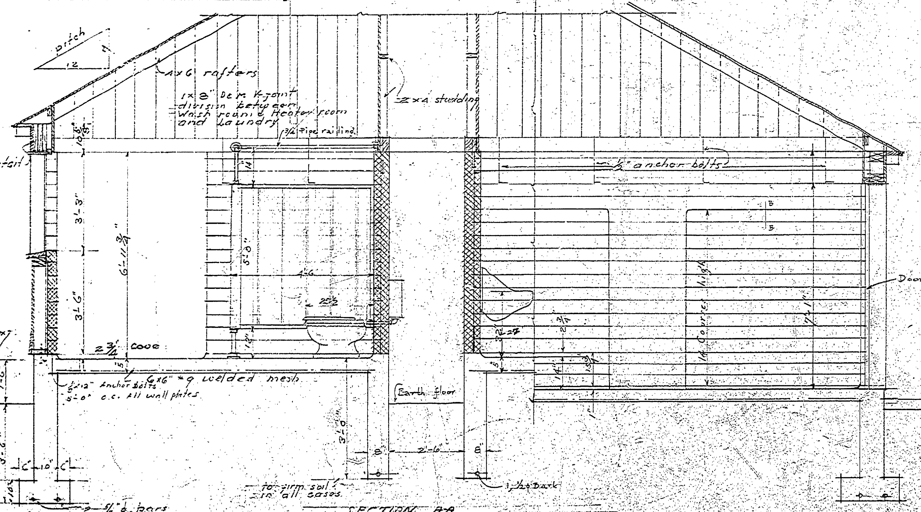
SECTION A-A Scale 1/4\"/>
