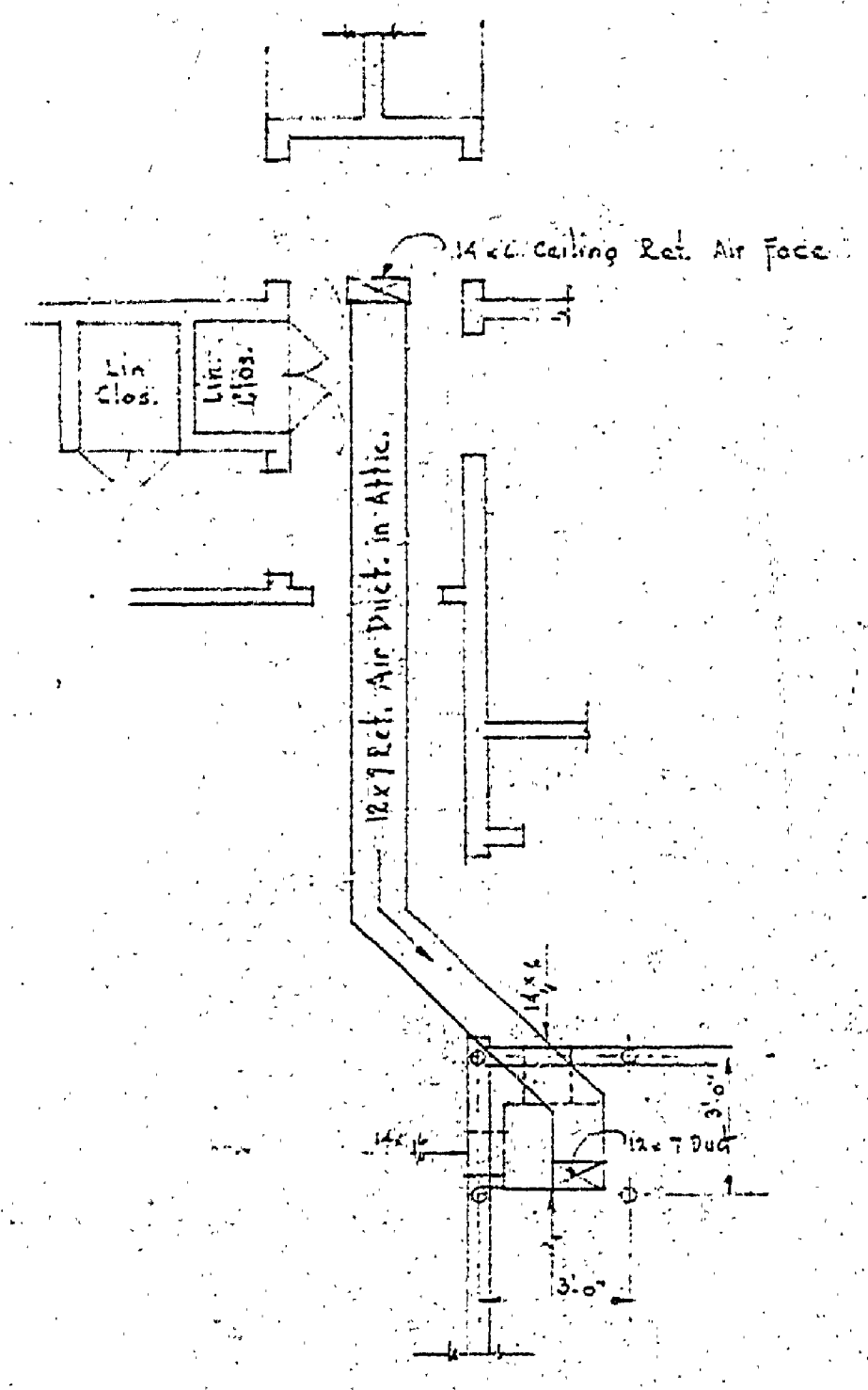
PLAN LAYOUT OF RETURN DUCT Scale: 1/8" = 1'-0"
