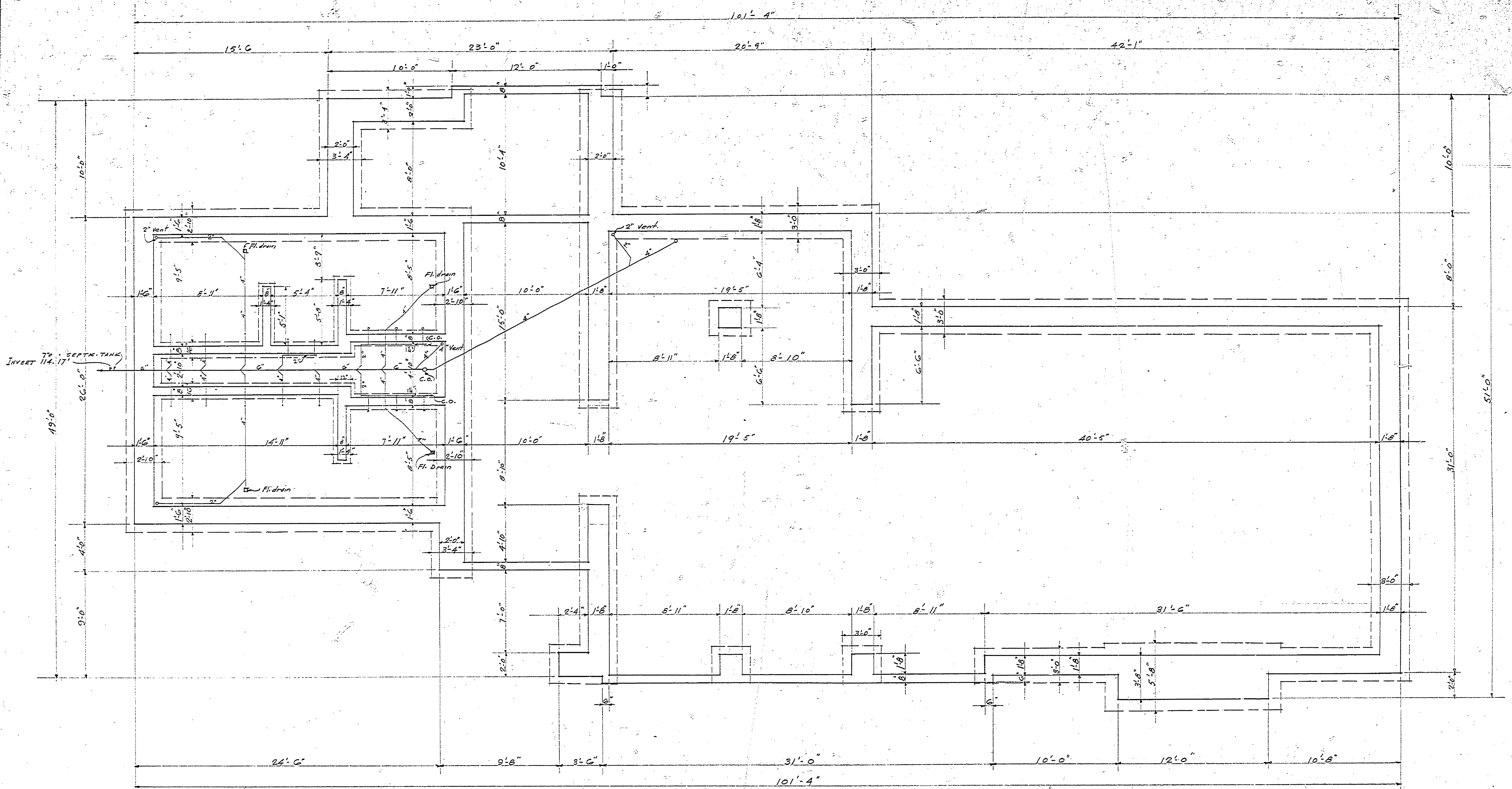
FOUNDATION PLAN SHOWING PLUMBING DIAGRAM SCALE 1/4" = 1'-0"
