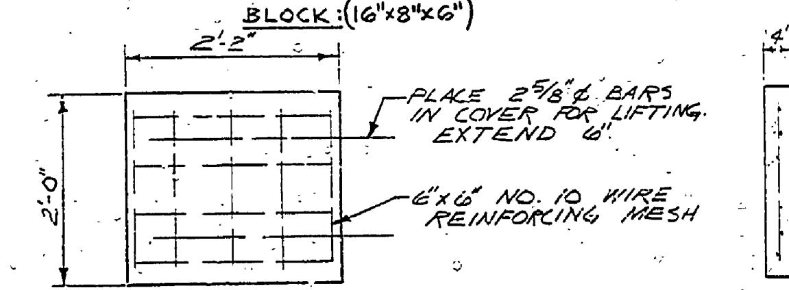
DISTRIBUTION BOX COVER 17 COVERS AT 2'-0" = 34' TOTAL LENGTH OF THE DISTRIBUTION BOX = 34'
