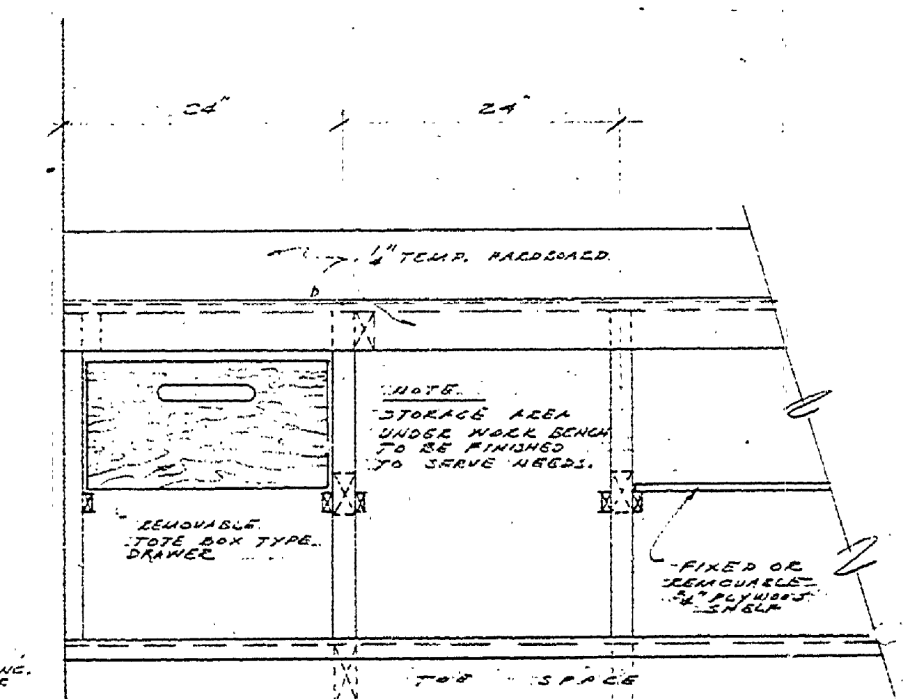
WORK BENCH DETAIL SCALE 1" = 1'-0"
