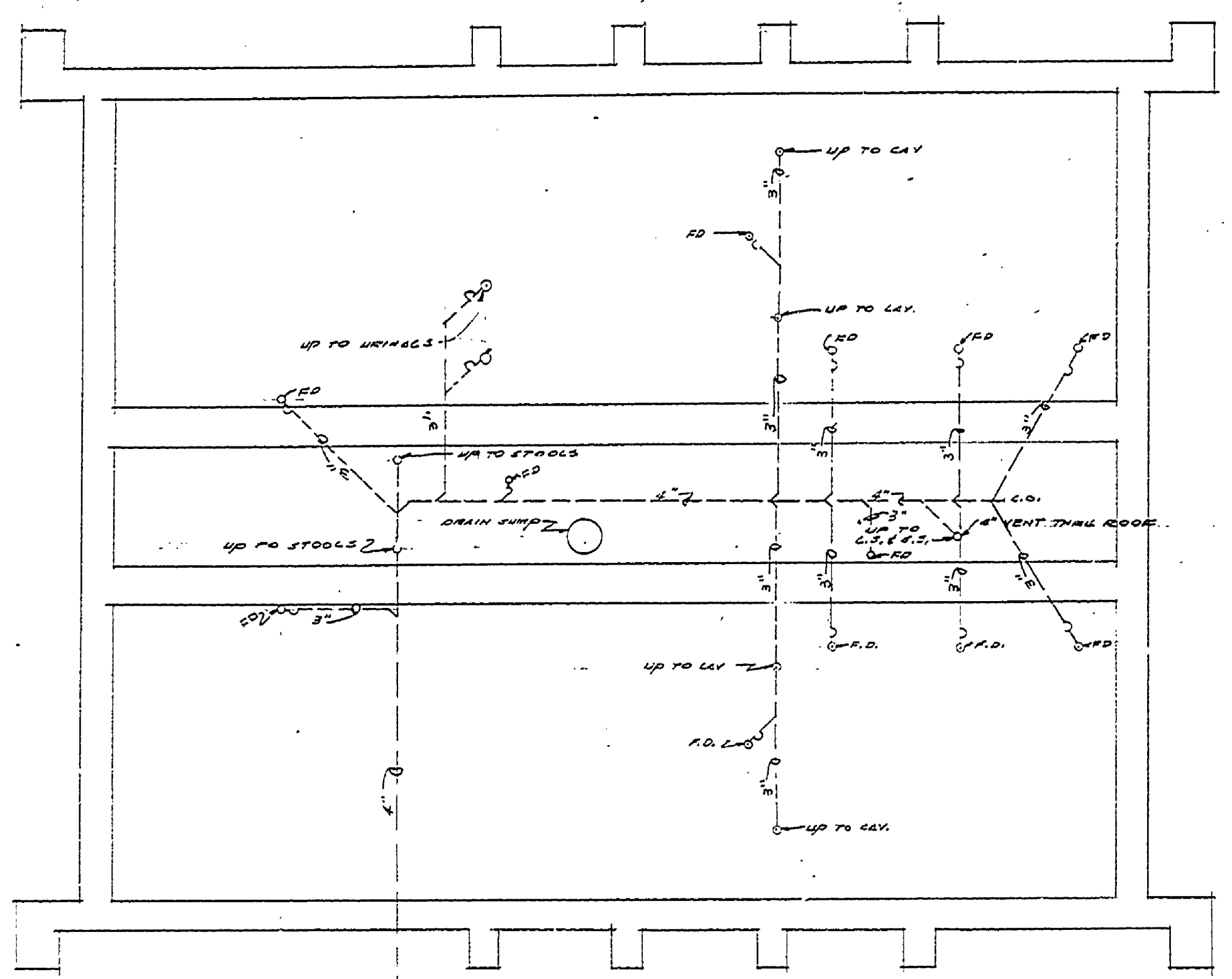
PLUMBING PLAN - UNDERGROUND WASTE
