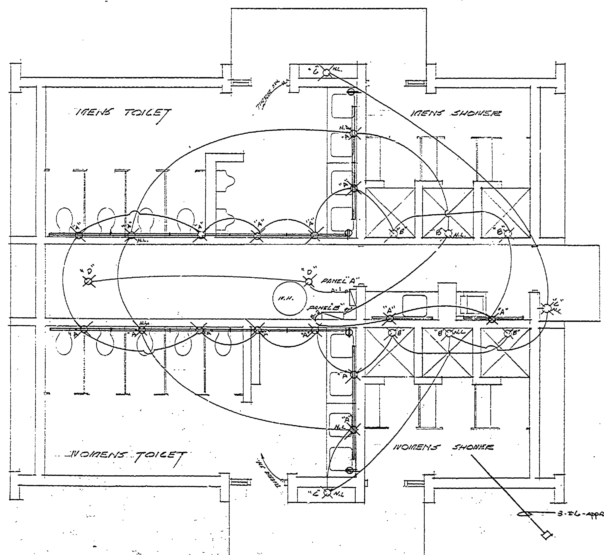
FLOOR PLAN - ELECTRICAL
