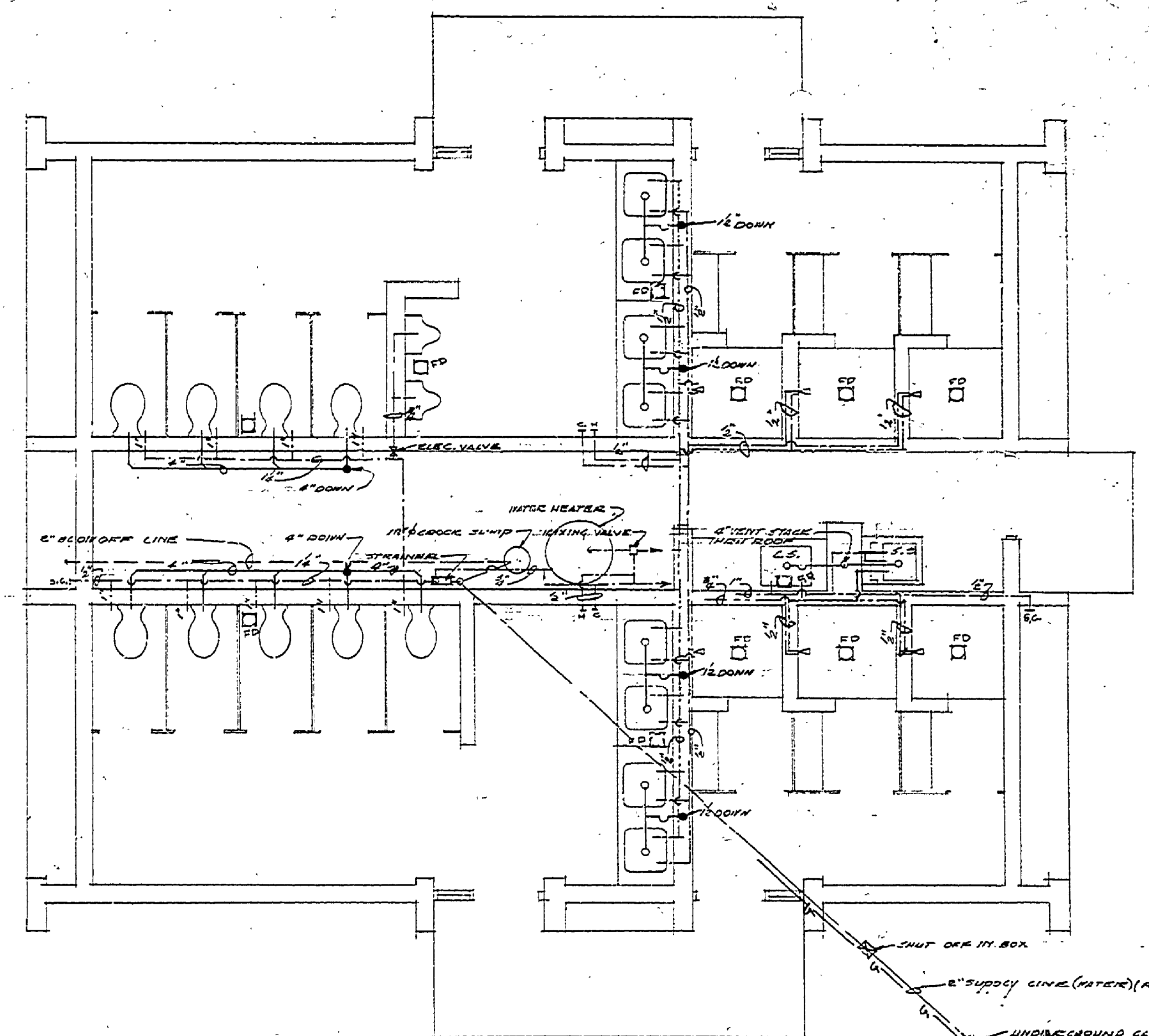
PLUMBING PLAN - ABOVE GROUND - WASTE & WATER
