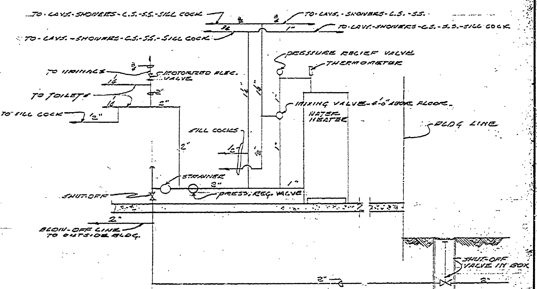
PLUMBING DIAGRAM - WATER
