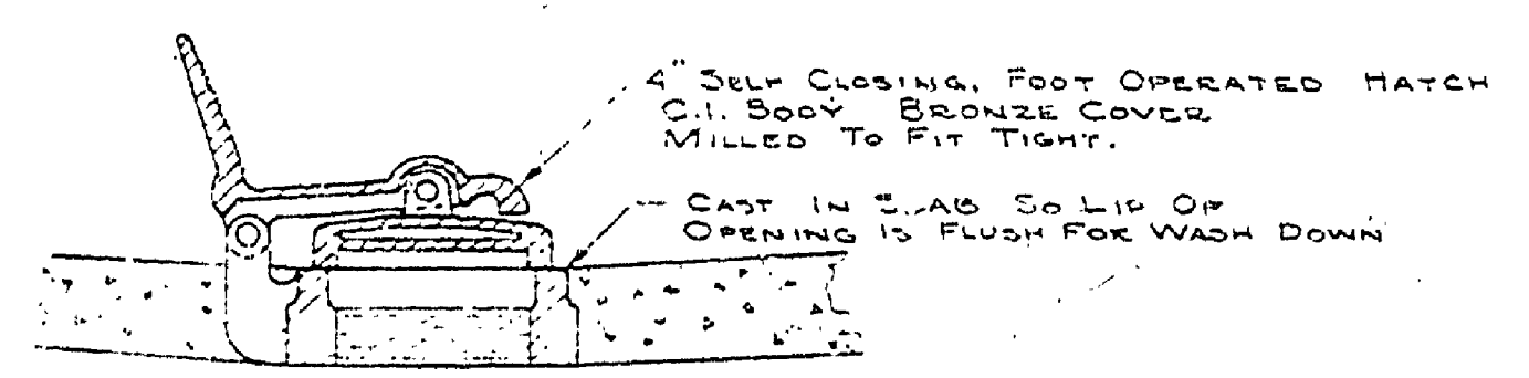
MATCH & COVER SECTION DETAIL VARCO FIG. 42 VARCO ENDOVER SYSTEMS CO. 2820 N. ALAMEDA COMPTON, CALIF.
