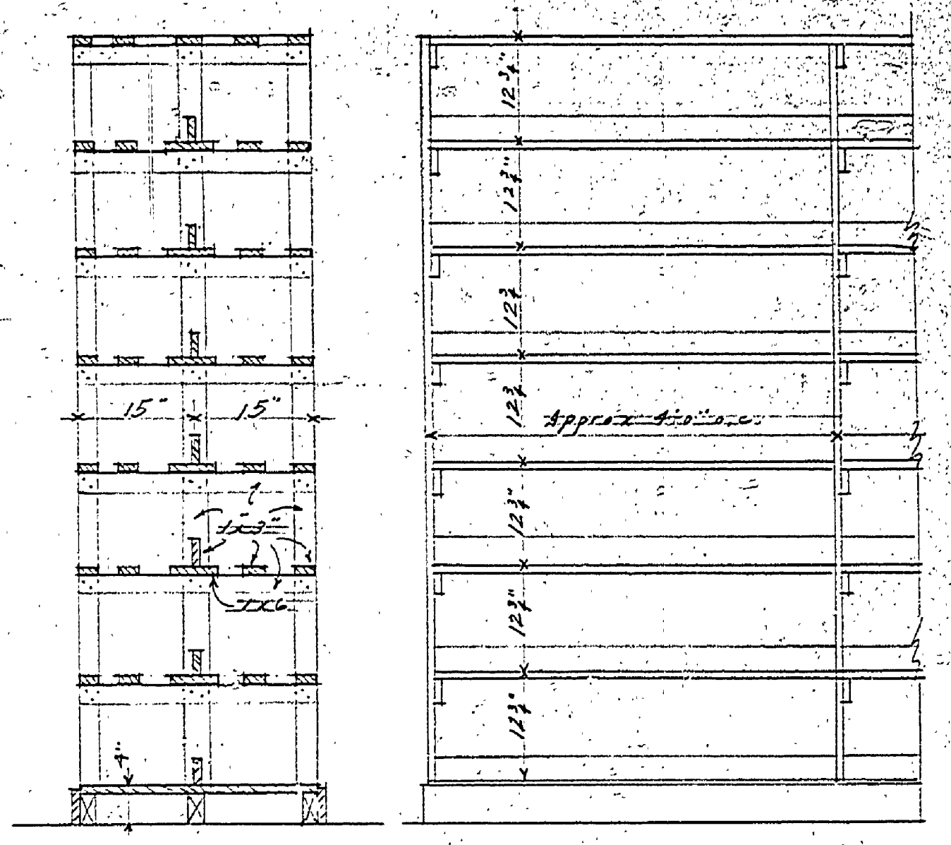
SECTION ELEVATION BASKET RACK DETAIL Scale: 3/4" = 1'-0"
