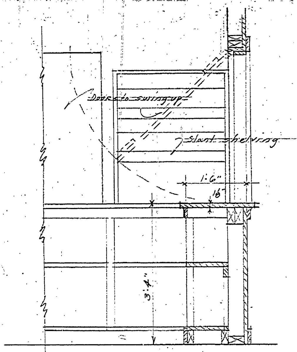
SECTION LOOKING TOWARD ENTRANCE COUNTER DETAIL Scale: 3/4" = 1'-0"
