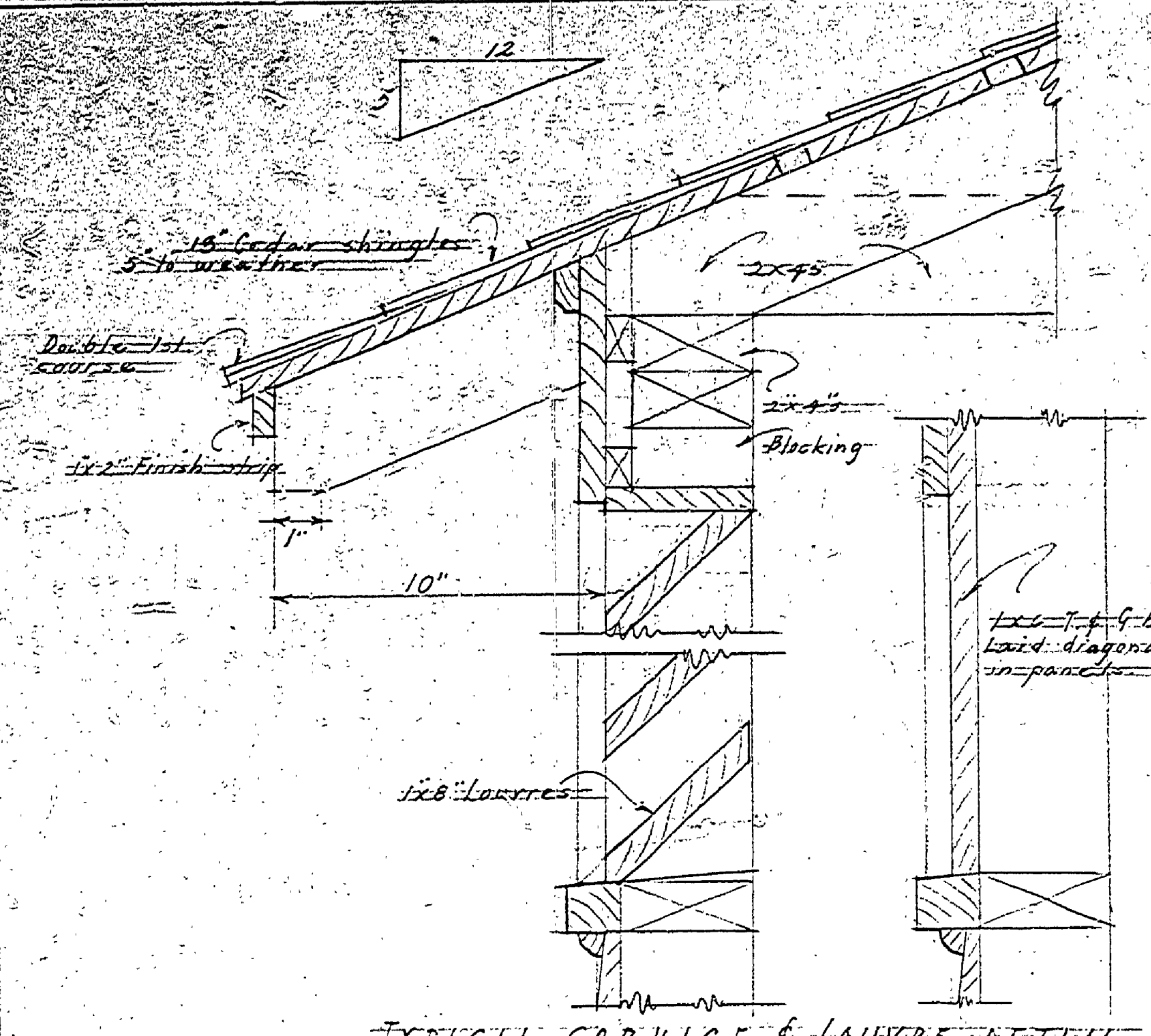
TYPICAL CORNICE & LOUVRE DETAIL Scale: 3/4" = 1'-0"
