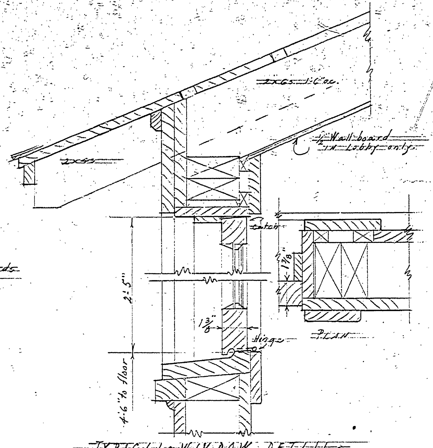
TYPICAL WINDOW DETAIL Scale: 3/4" = 1'-0"
