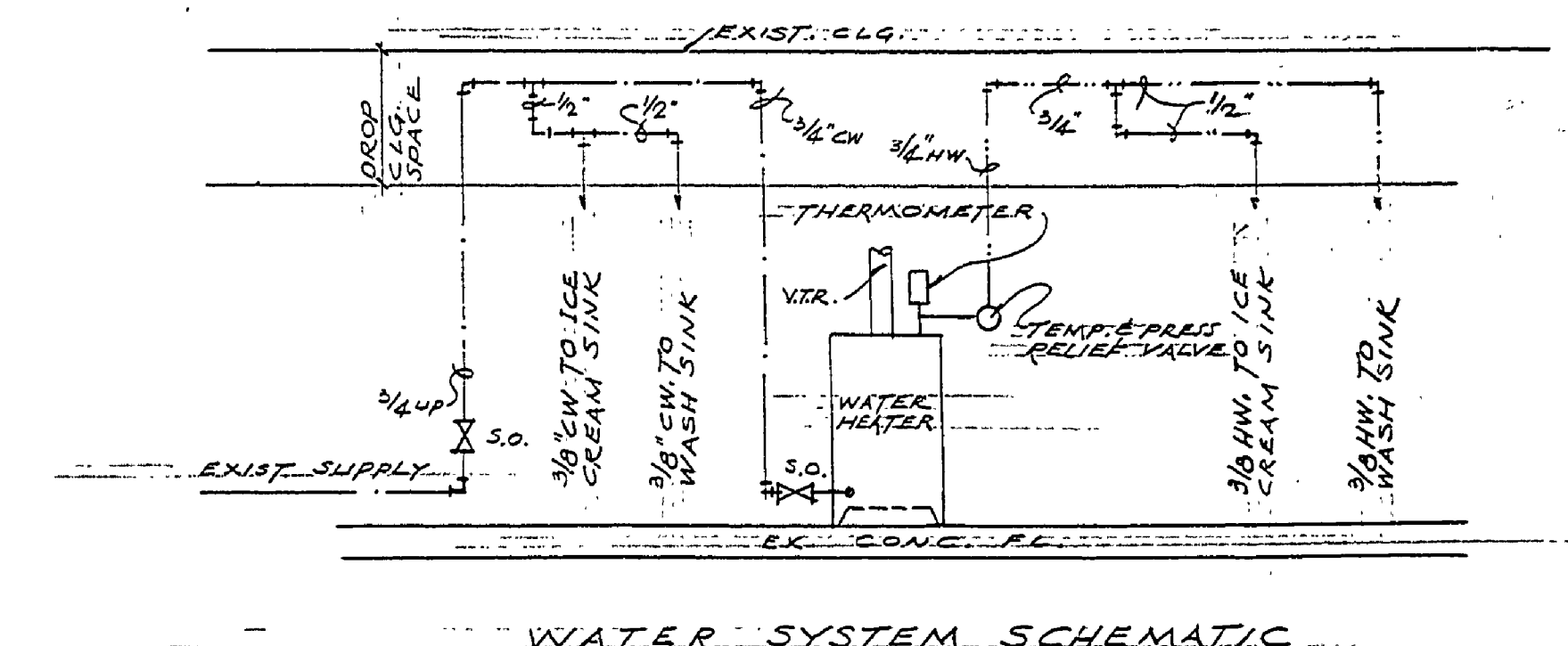
WATER SYSTEM SCHEMATIC
