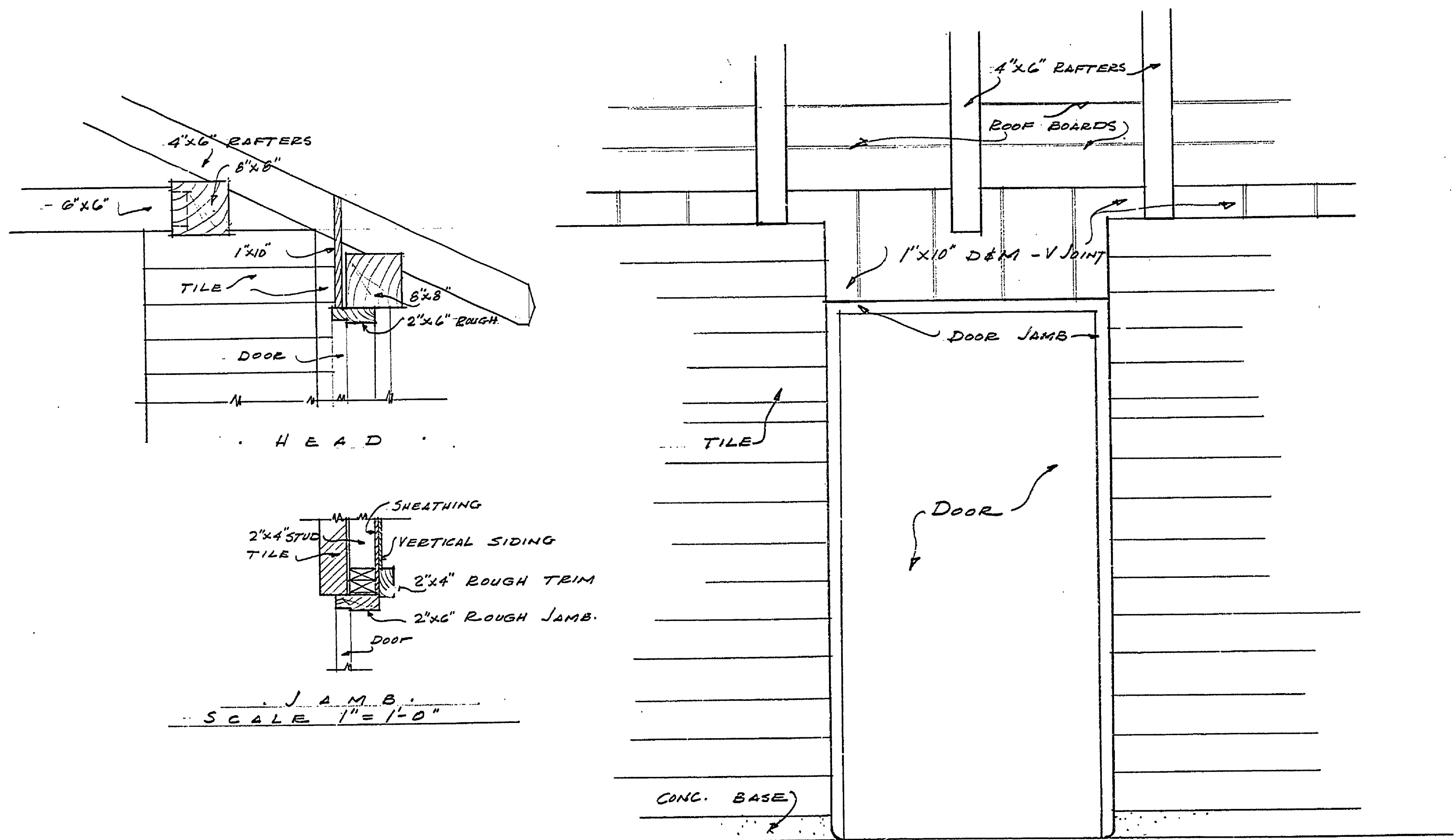
ELEVATION AT DOOR
