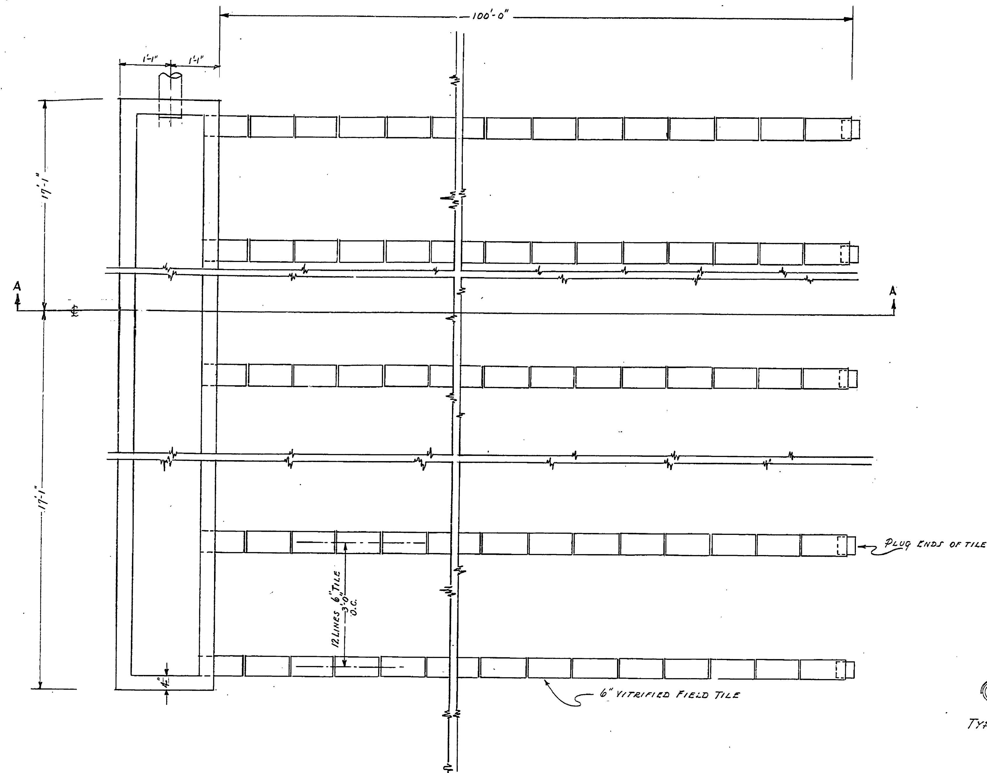
PLAN OF DISPOSAL FIELD Scale 3/4"=1'-0"
