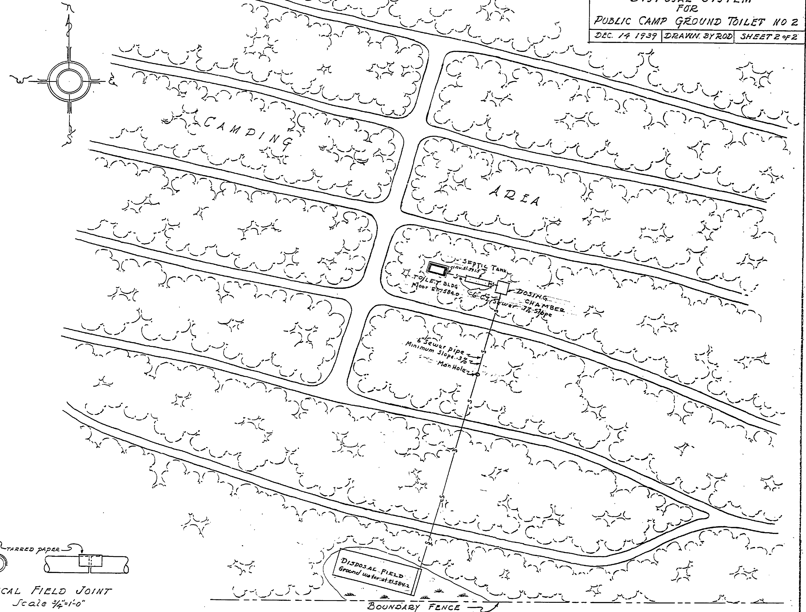
PLOT PLAN TOILET NO. 2 DISPOSAL SYSTEM Scale 1"=60'
