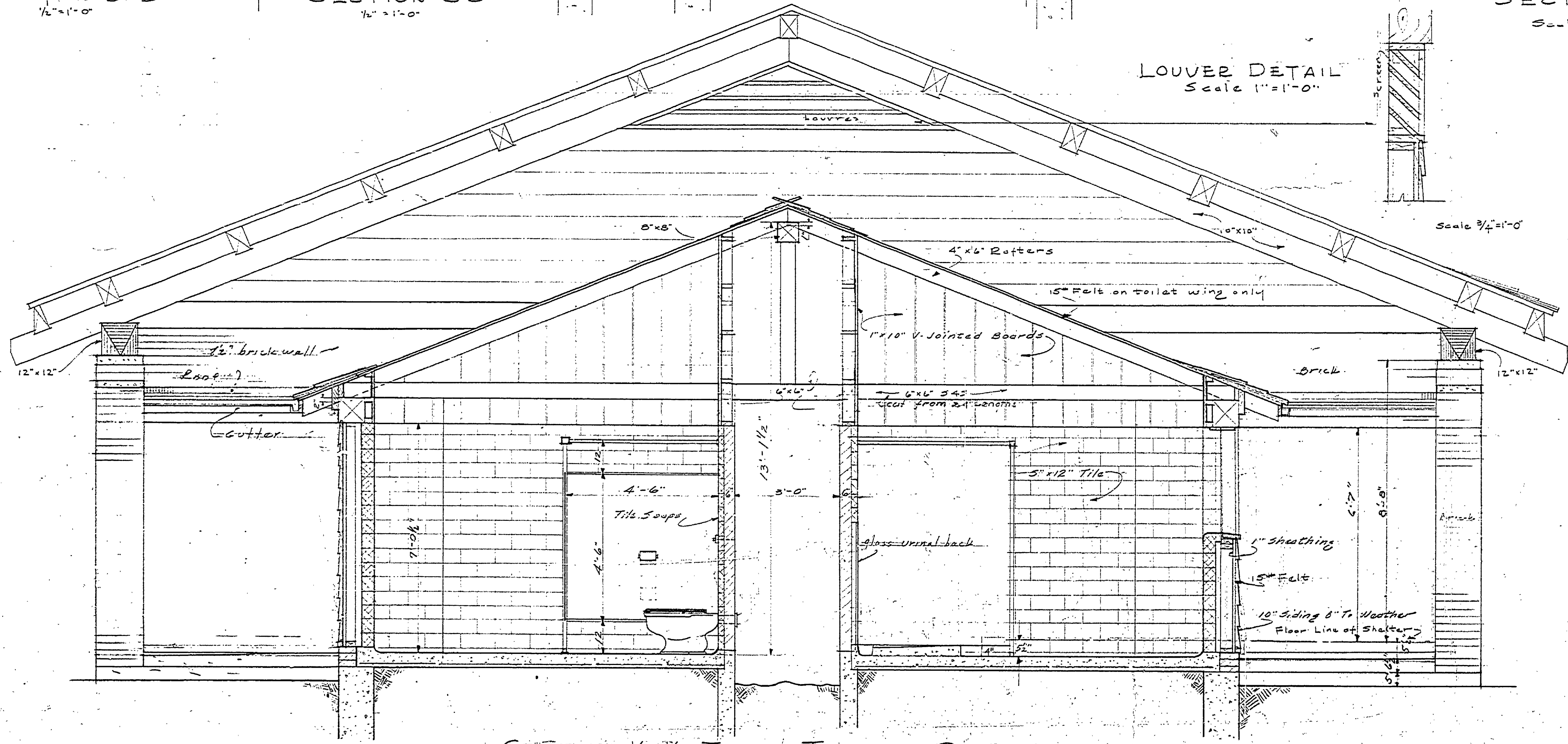
SECTION K-K THRU TOILET ROOM Scale 1/2" = 1'-0"
