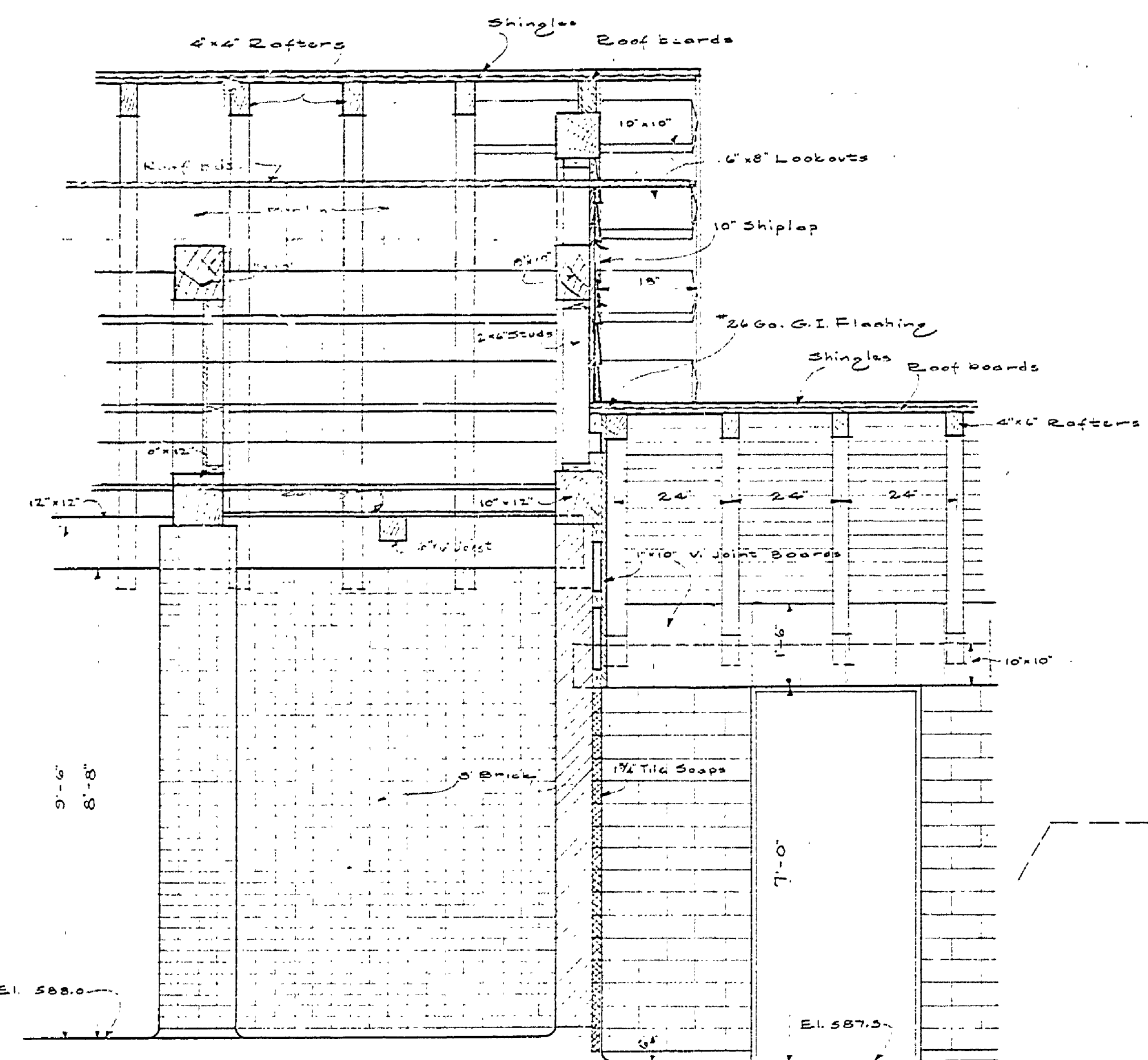
SECTION F-F Scale 1/2" = 1'-0"
