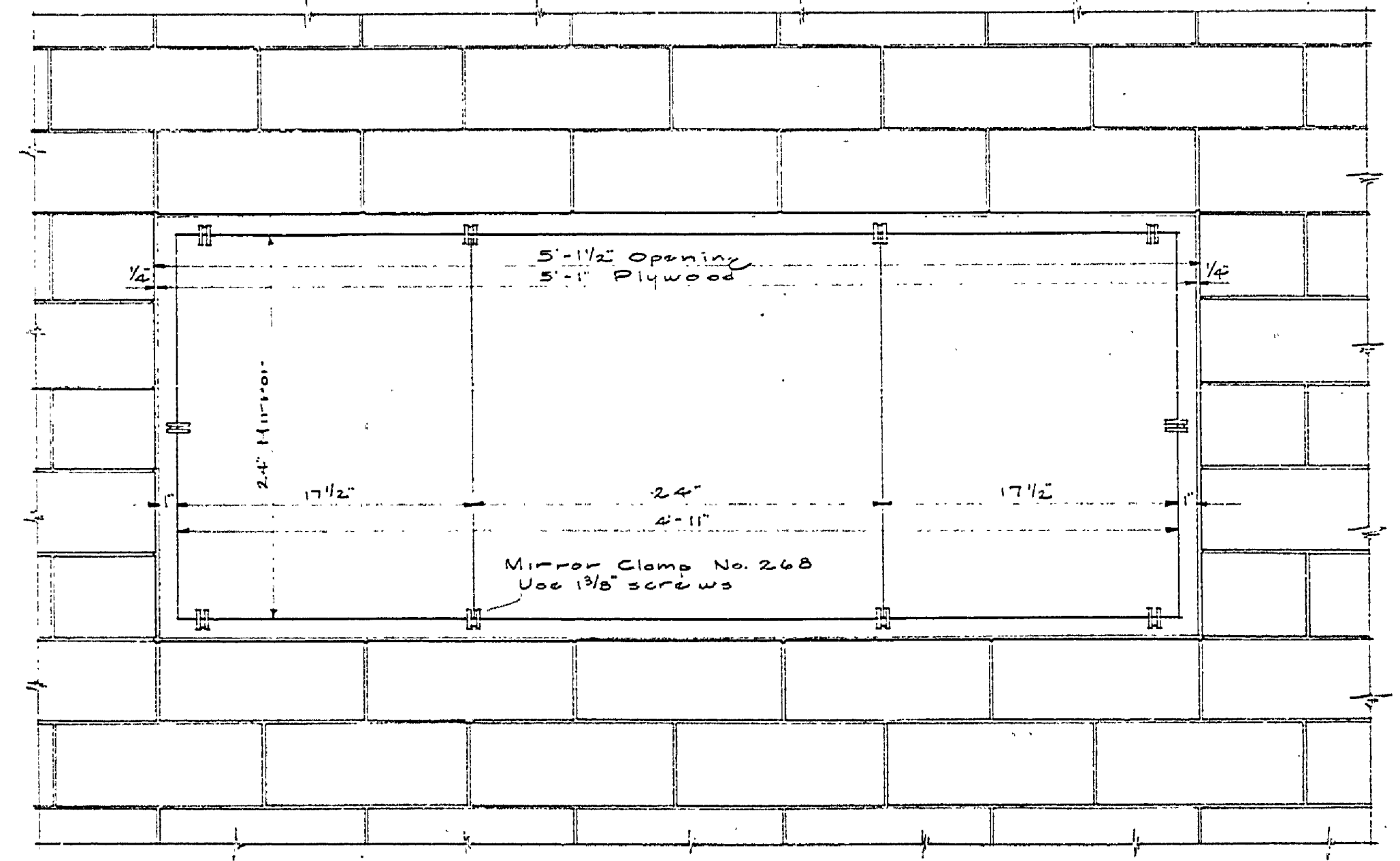
MAIN TOILET ROOM MIRROR DETAIL Scale 1/2" = 1'-0"
