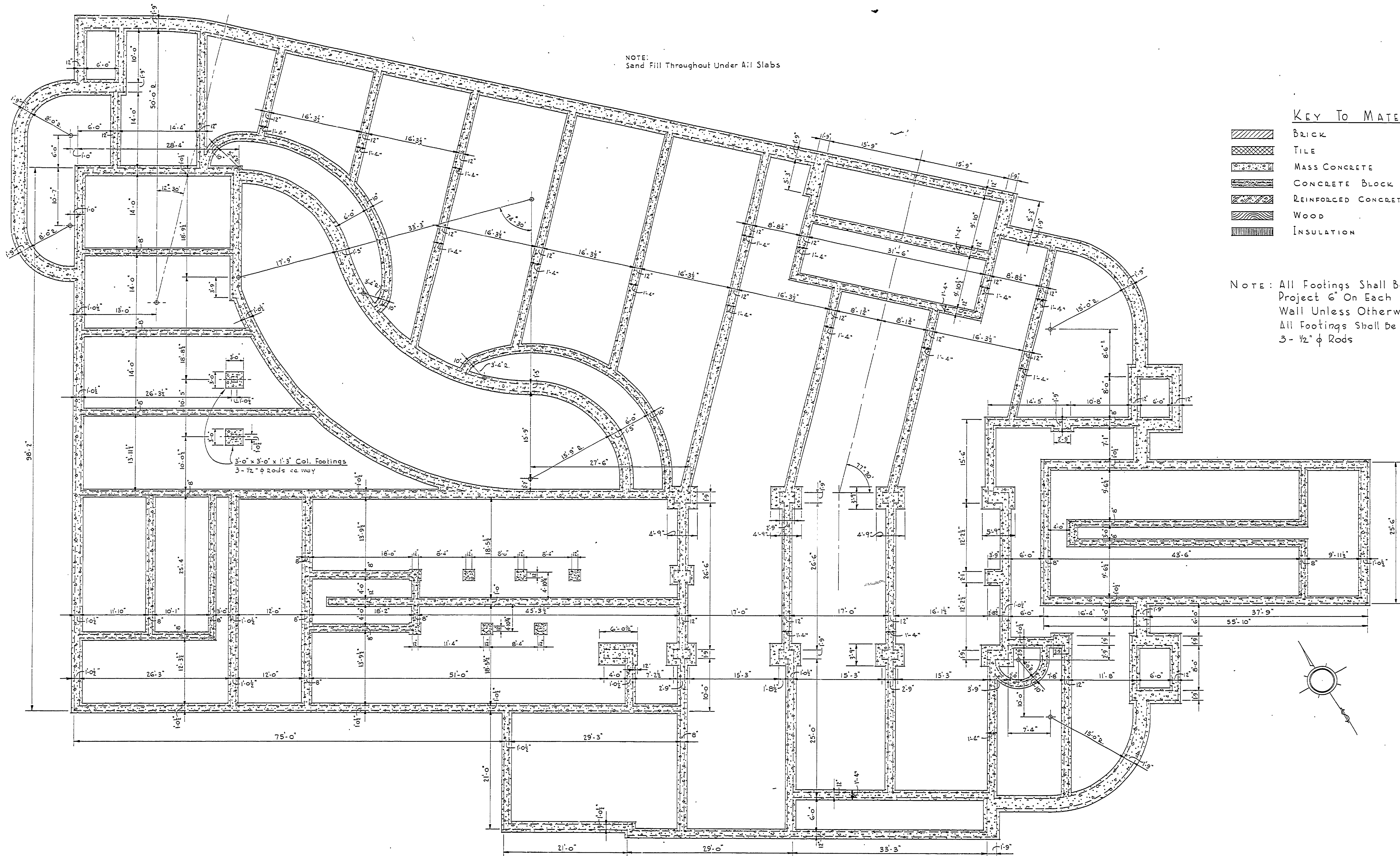
FOUNDATION & FOOTING PLAN Scale 1/8" = 1'-0"
