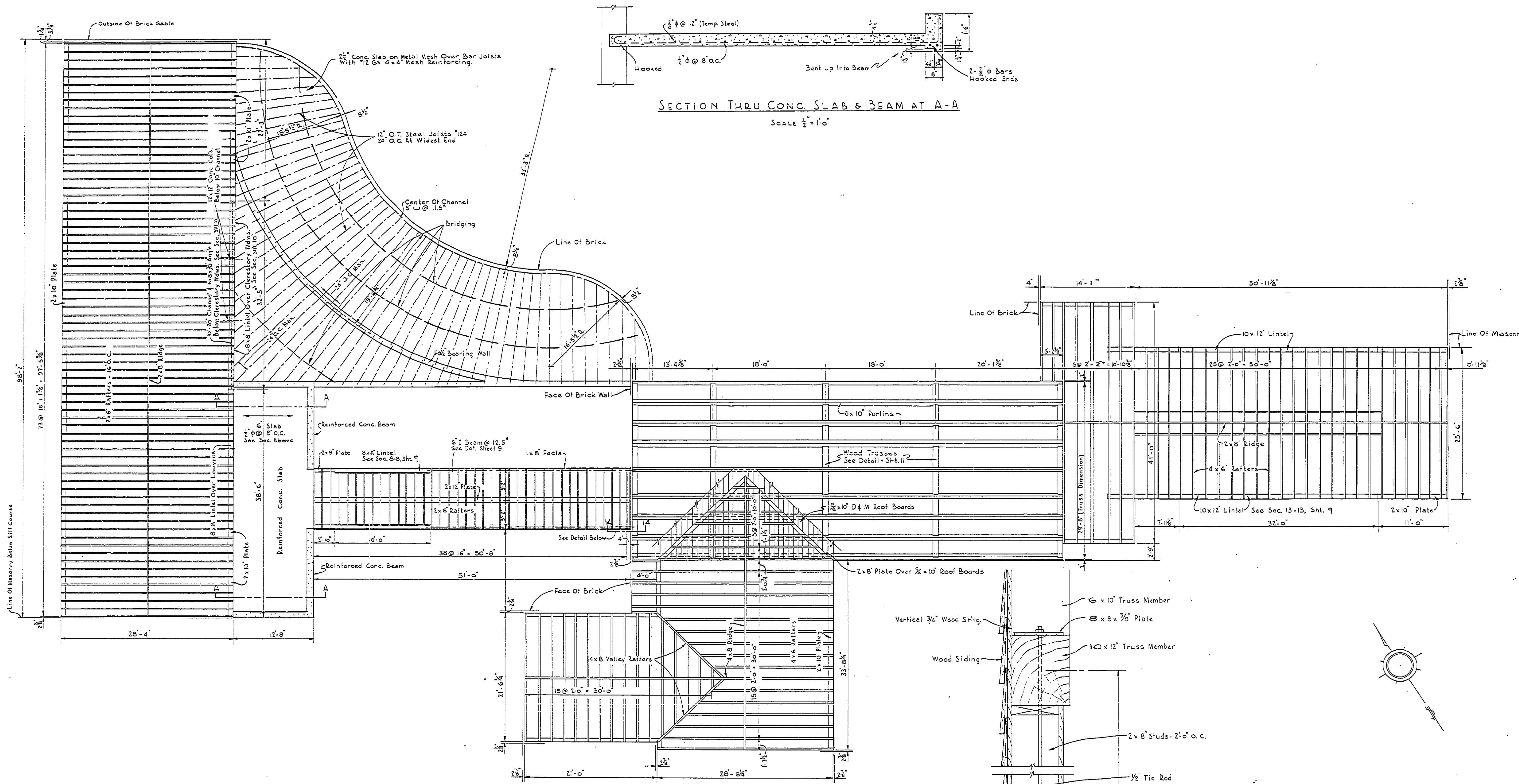
ROOF FRAMING PLAN Scale 1/8" = 1'-0"
