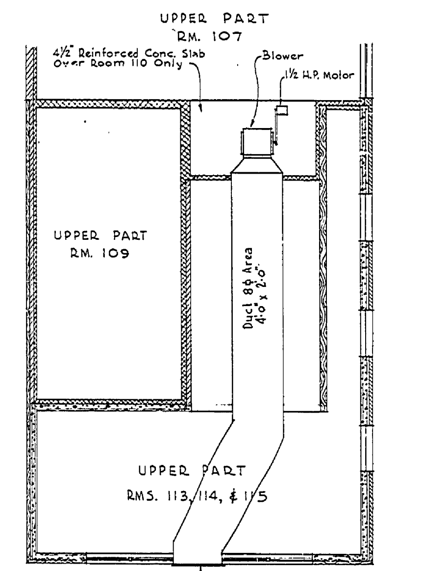
SECTION DETAIL OF KITCHEN FAN INSTALLATION Scale 1/8" = 1'-0"
