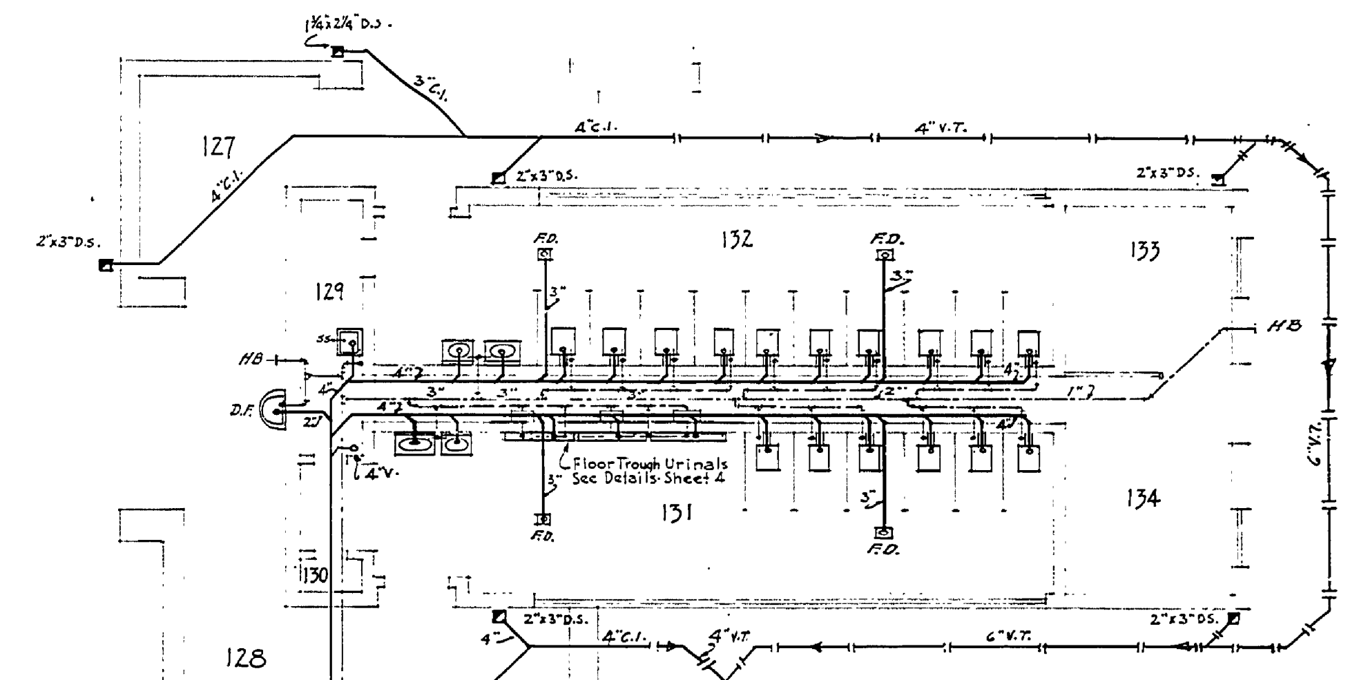
TYPICAL BRANCH MAIN TO W.C. FLUSH VALVES.
