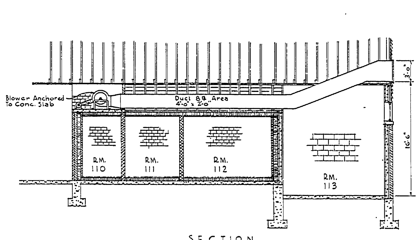
SECTION DETAIL OF KITCHEN FAN INSTALLATION Scale 1/8" = 1'-0"
