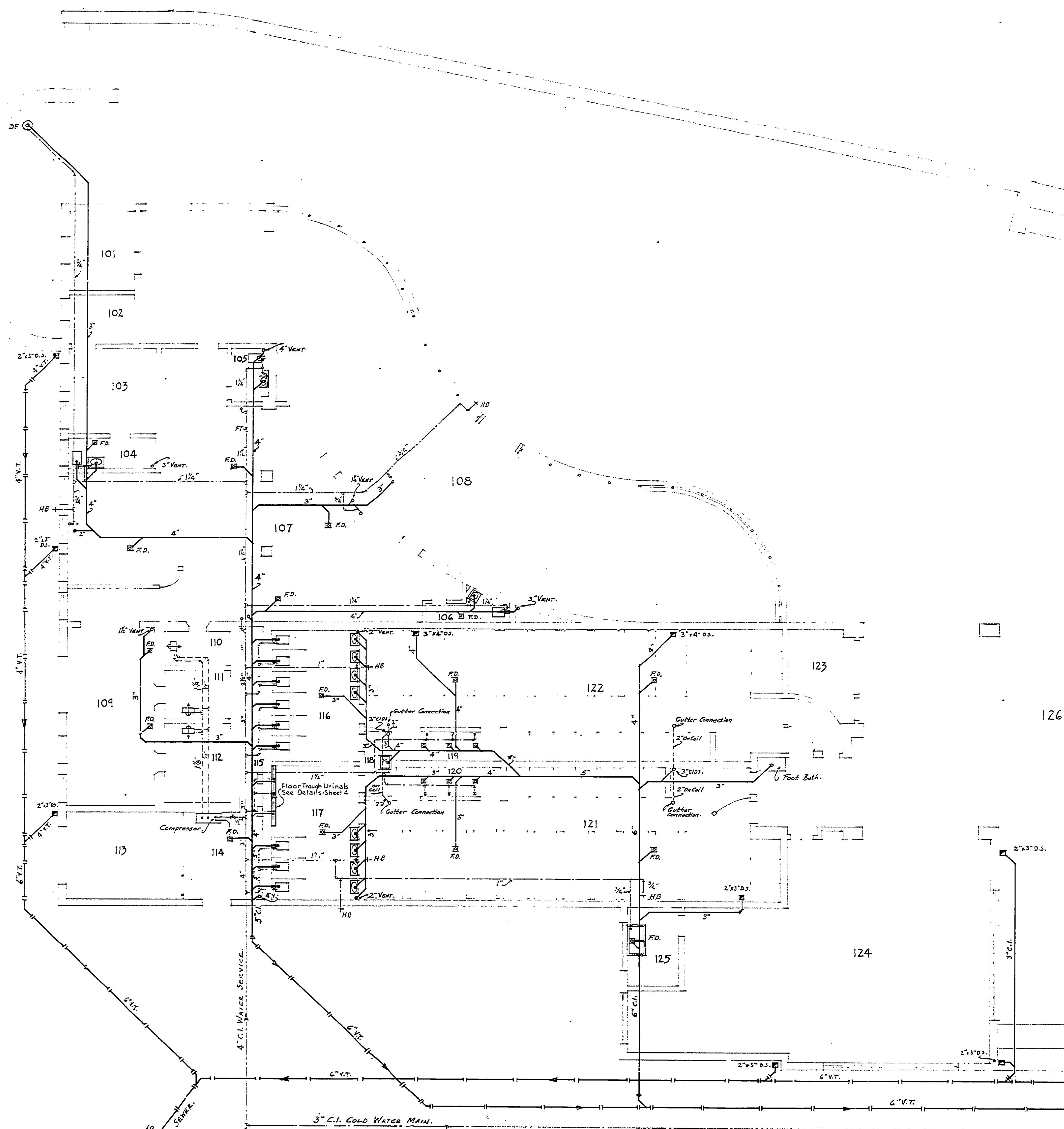
PLUMBING PLAN Scale 1/8" = 1'-0"
