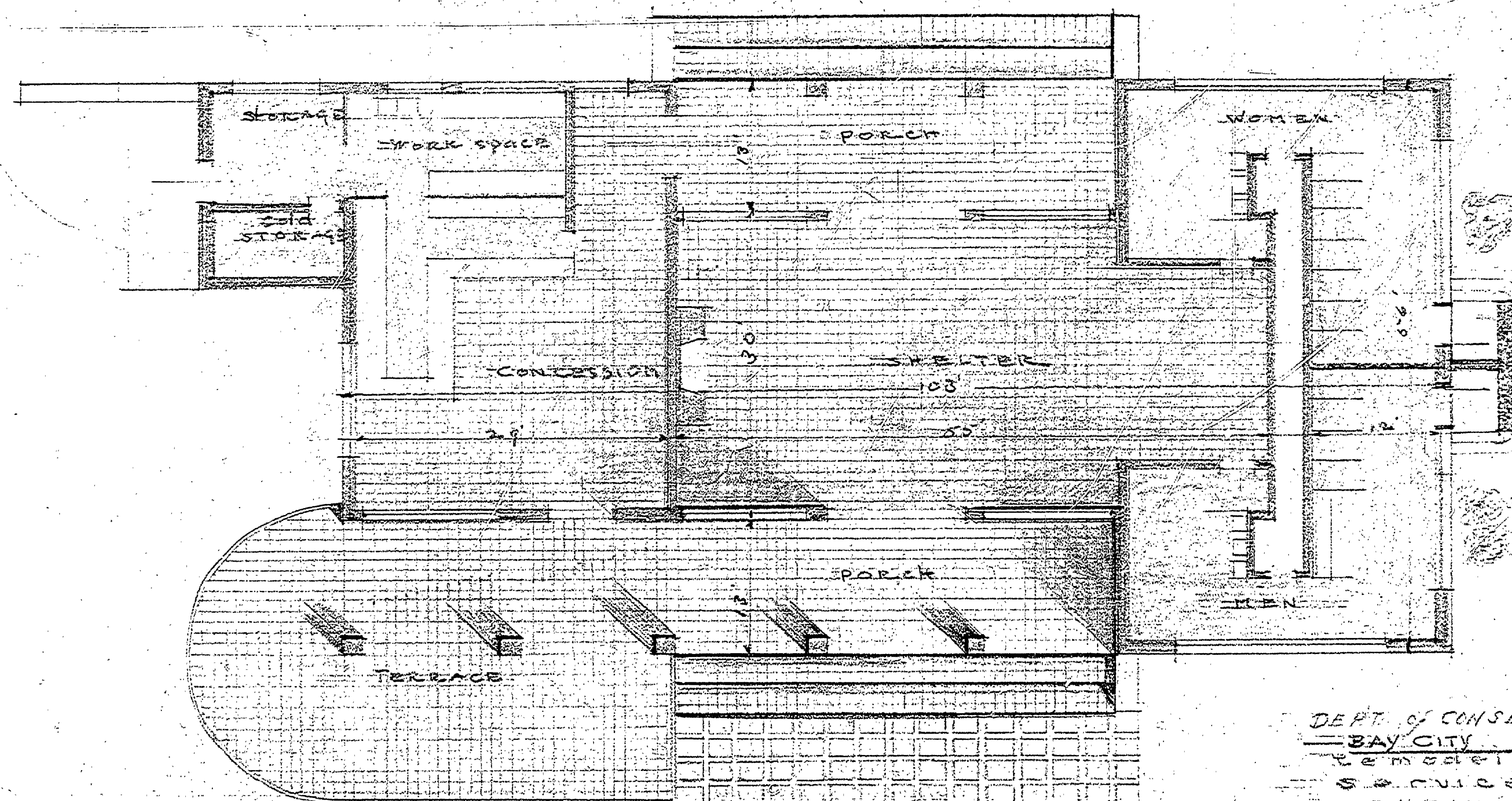
FLOOR PLAN
