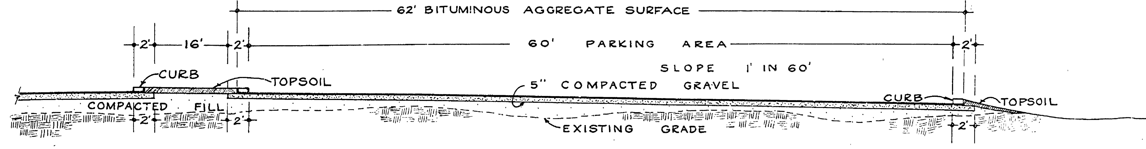
PARKING AREA SECTION
