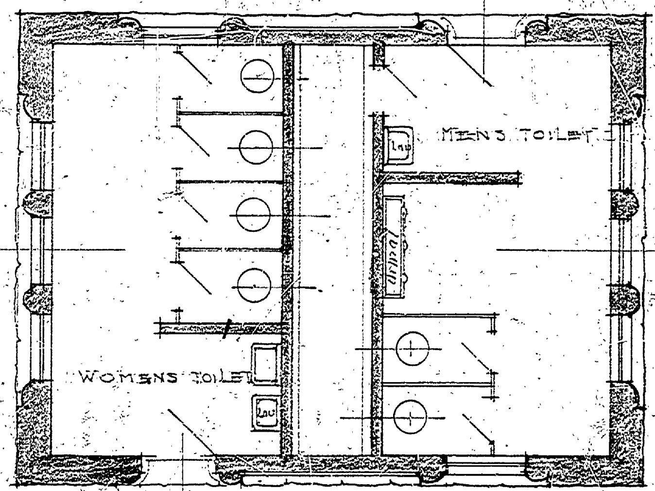
FLOOR PLAN SCALE 1/2" = 1'-0" OUTSIDE DIMENSIONS 20'-0" x 26'-0"
