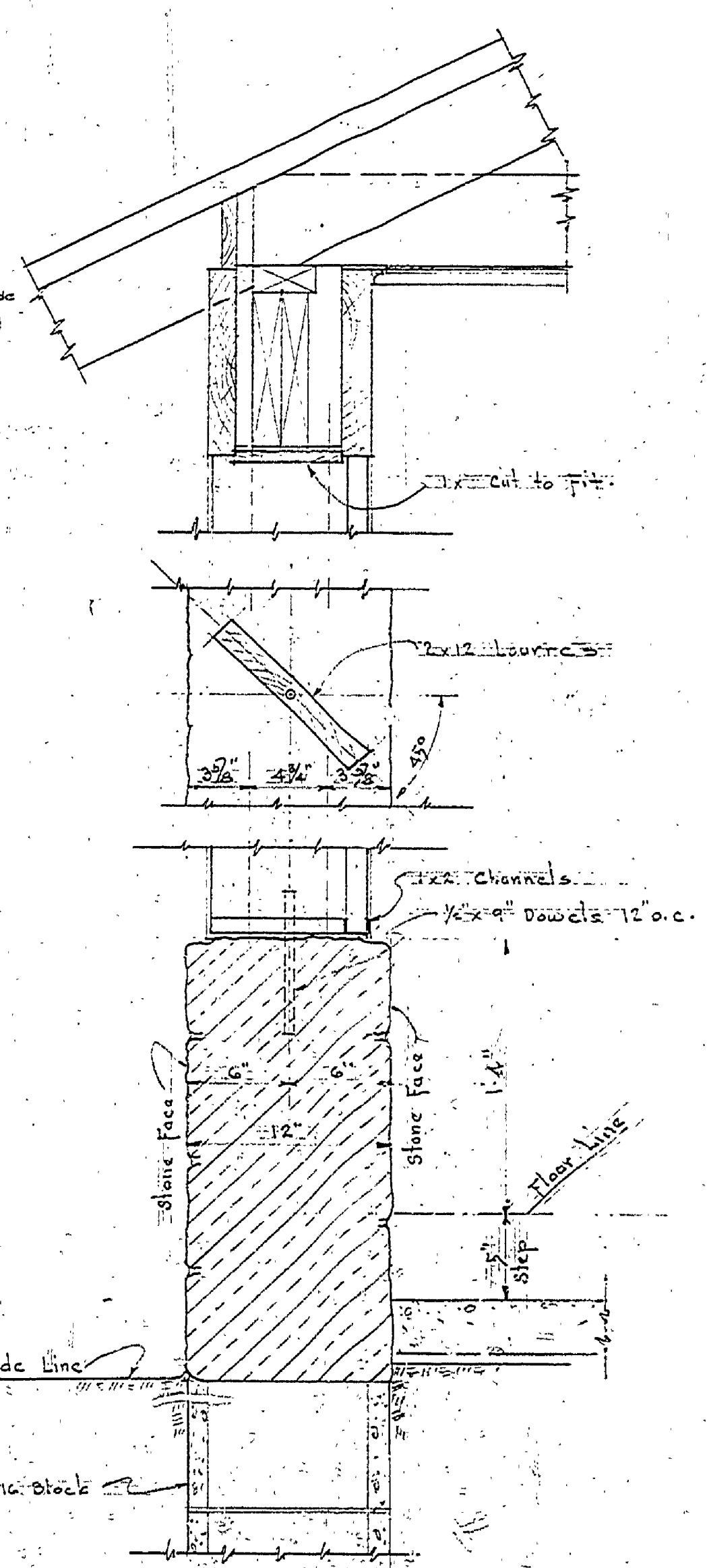
DETAIL Scale 1/2" = 1'-0"
