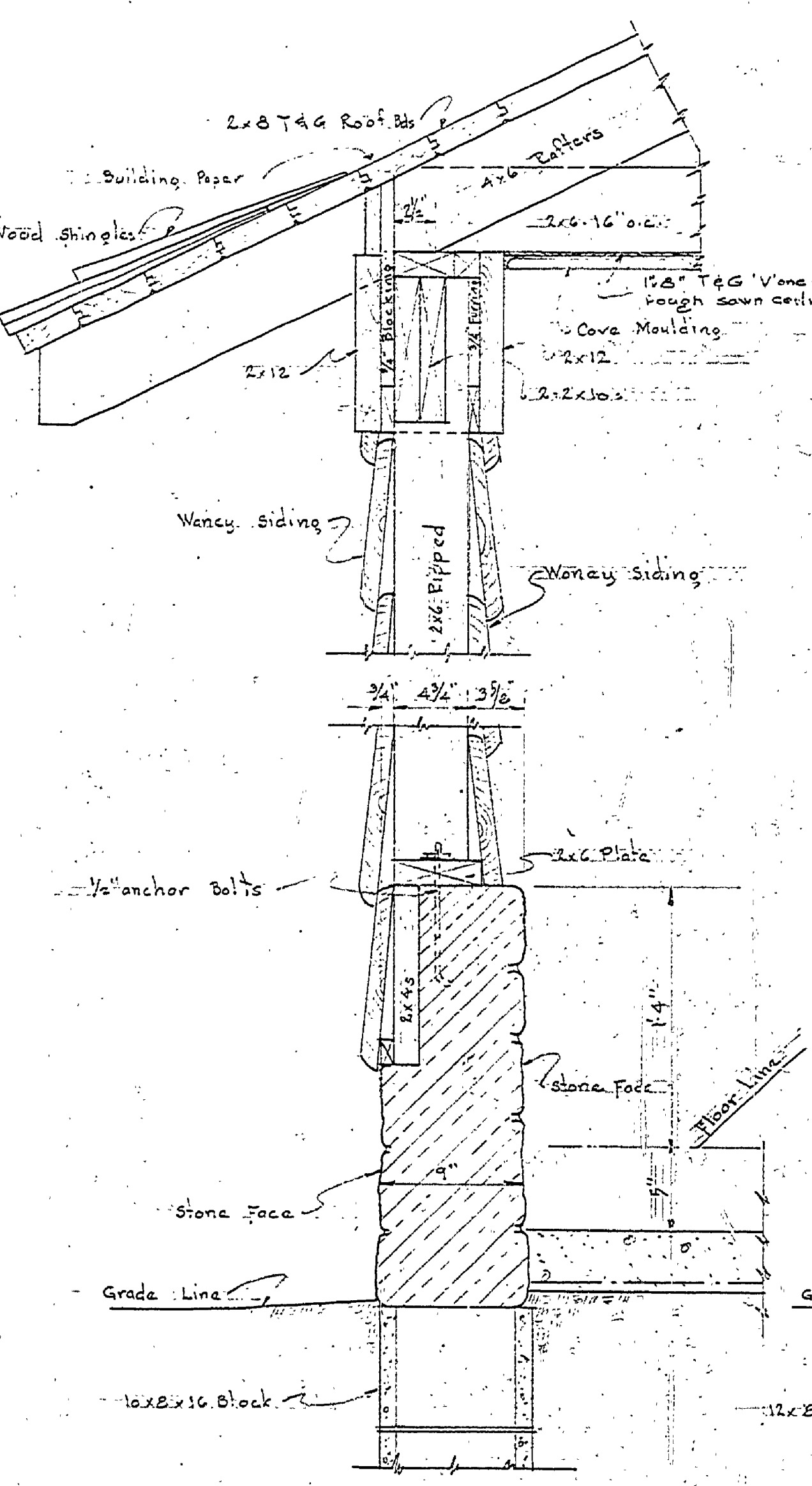
DETAIL Scale 1/2" = 1'-0"
