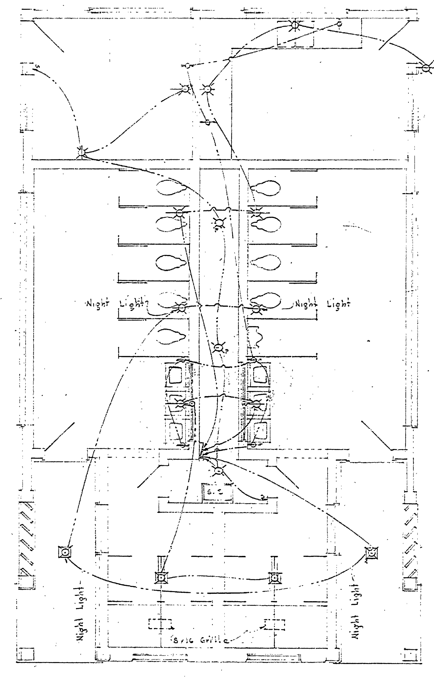
ELECTRICAL LAYOUT Scale 1/2" = 1'-0"
