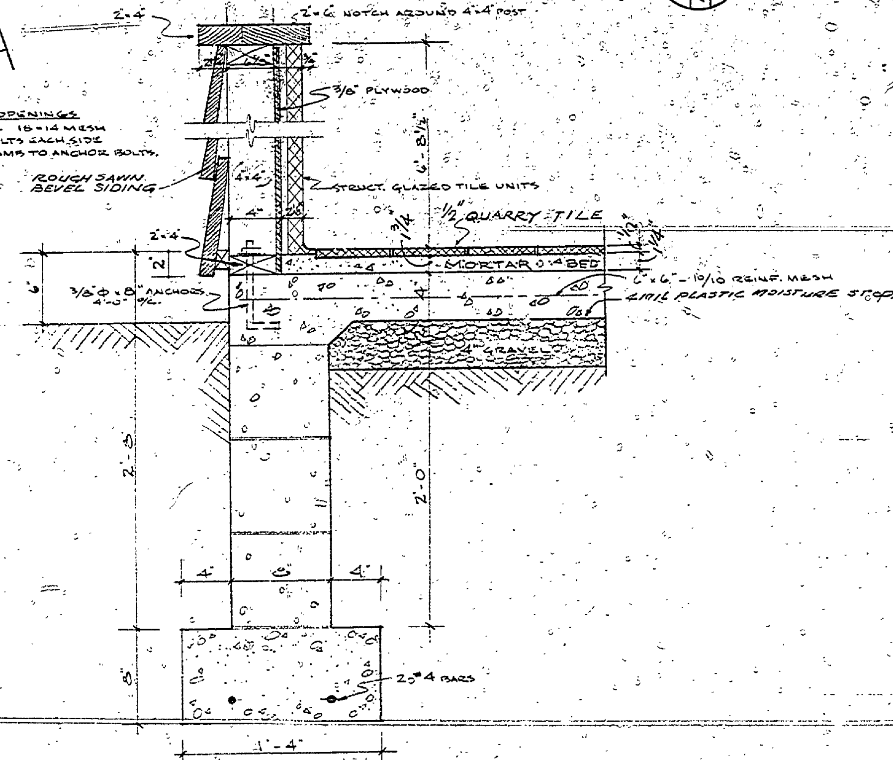
FOUNDATION SECTION 1/2" = 1'-0"
