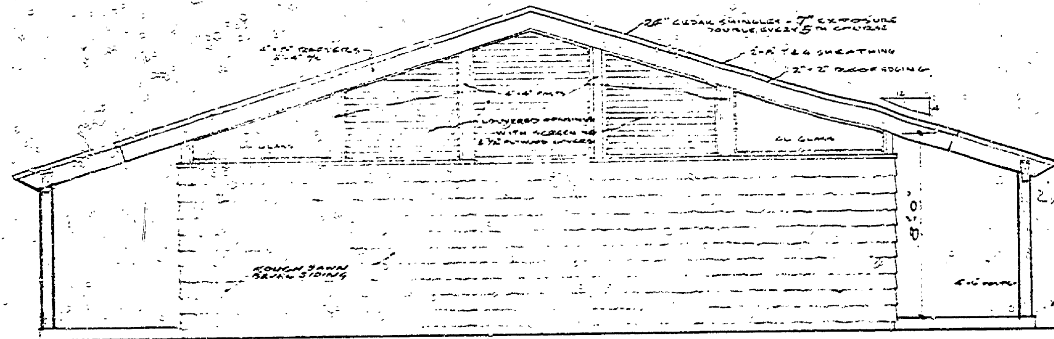
EAST ELEVATION 1/2" = 1'-0"
