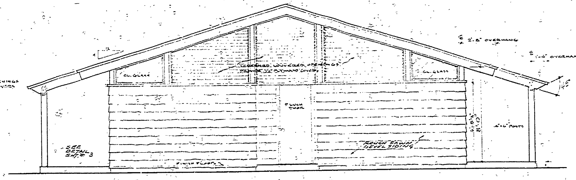
WEST ELEVATION 1/2" = 1'-0"
