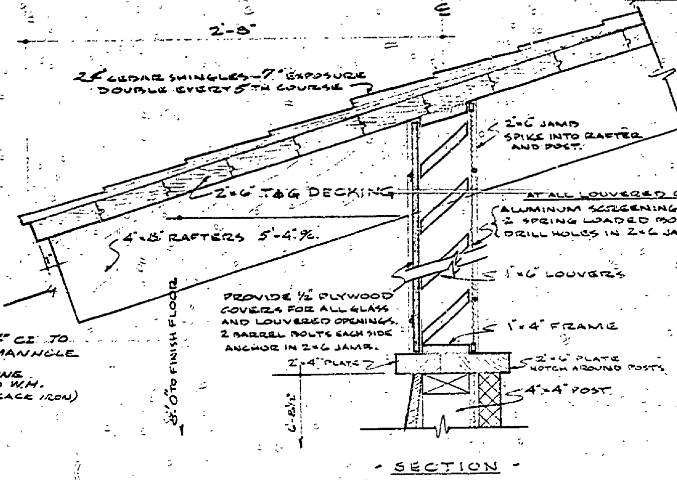
SECTION 1/2" = 1'-0"
