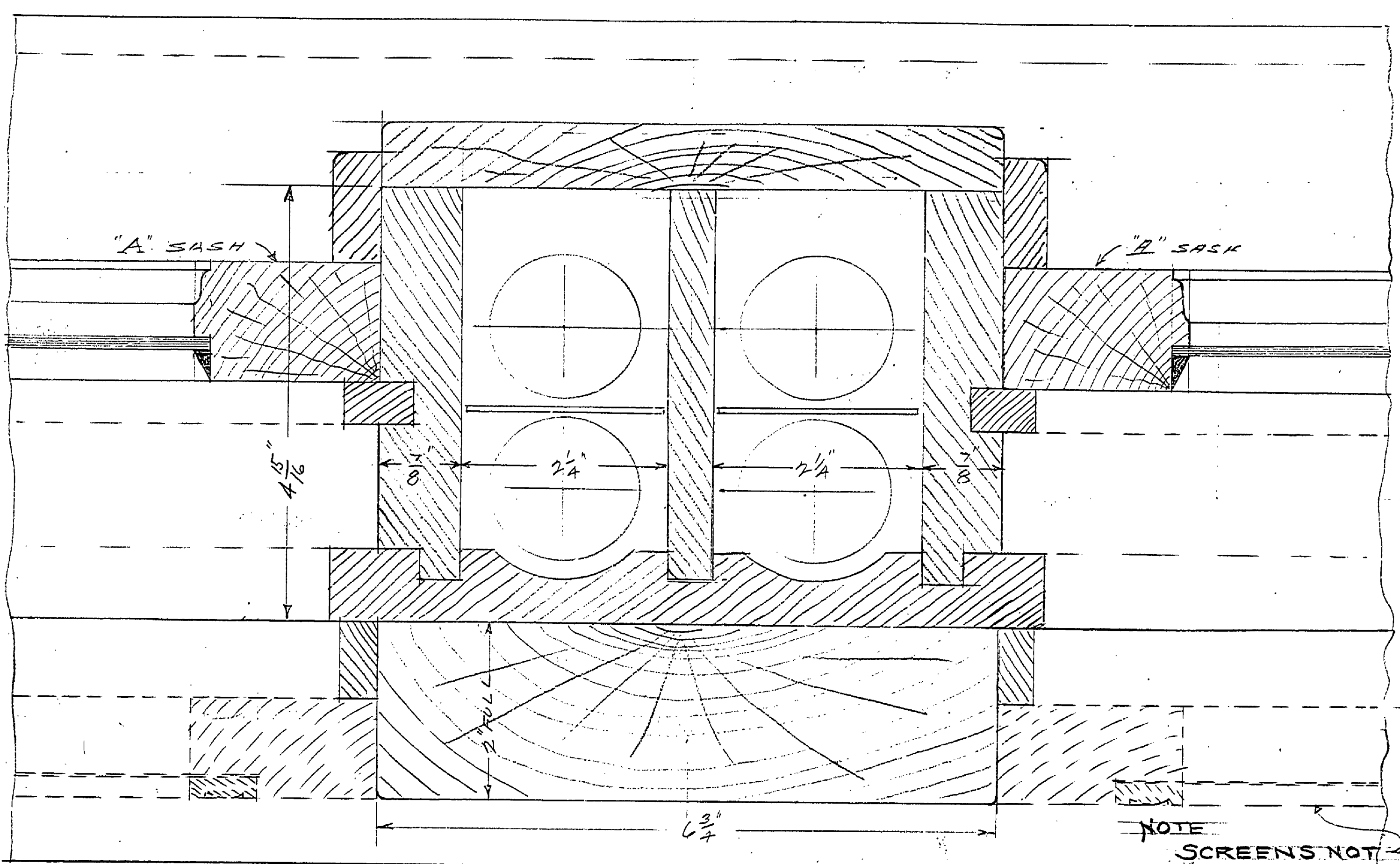
MULLION FOR DOUBLE FRAME - FULL SIZE.
