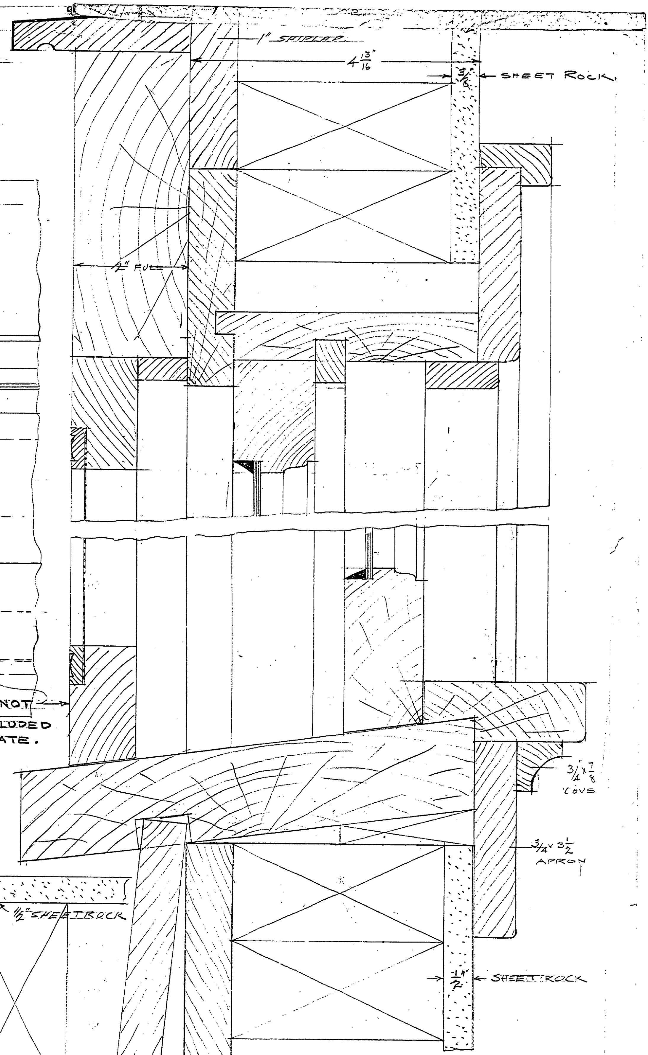
TYPICAL SECTION - FULL SIZE.
