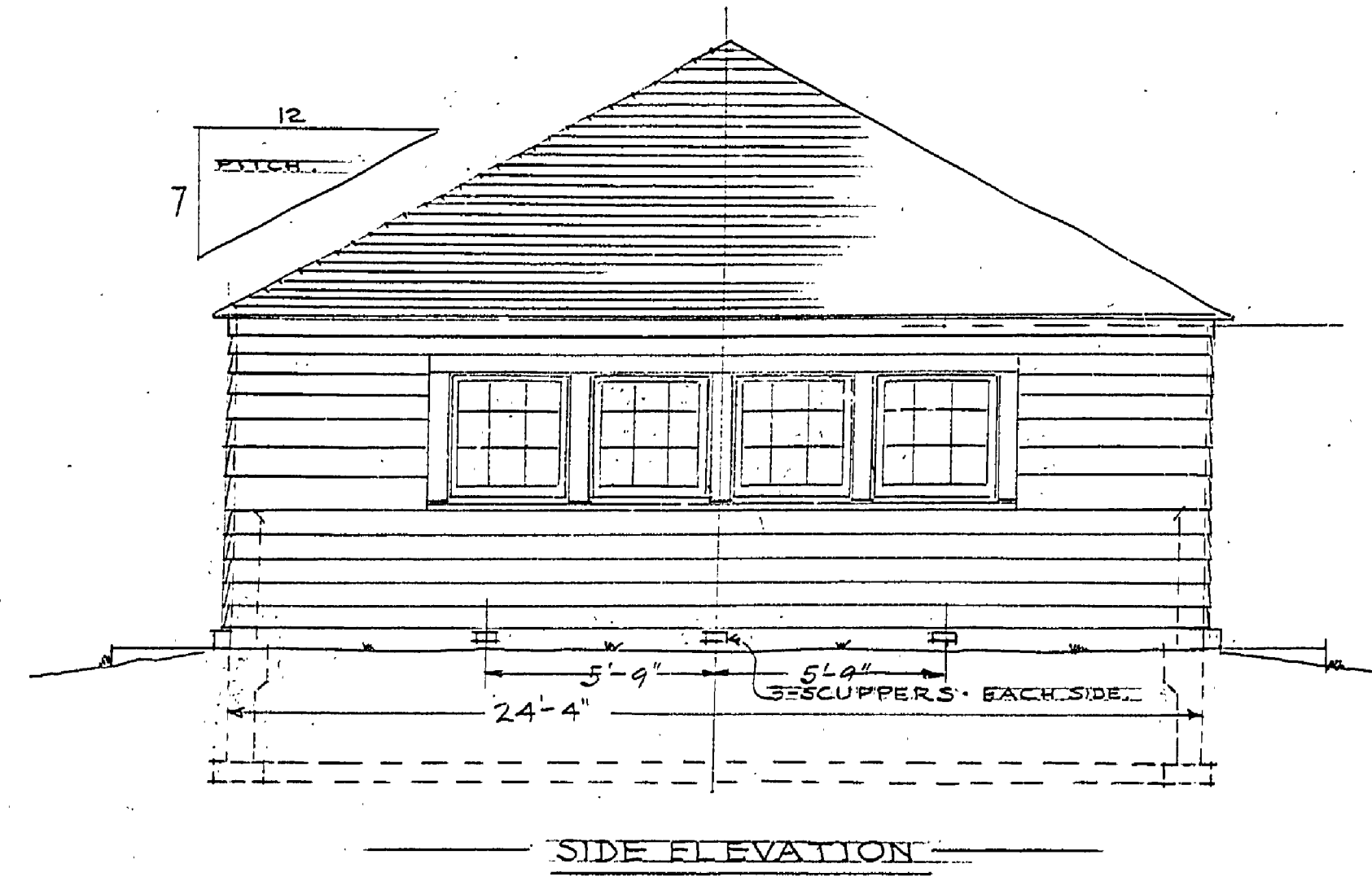
SIDE ELEVATION
