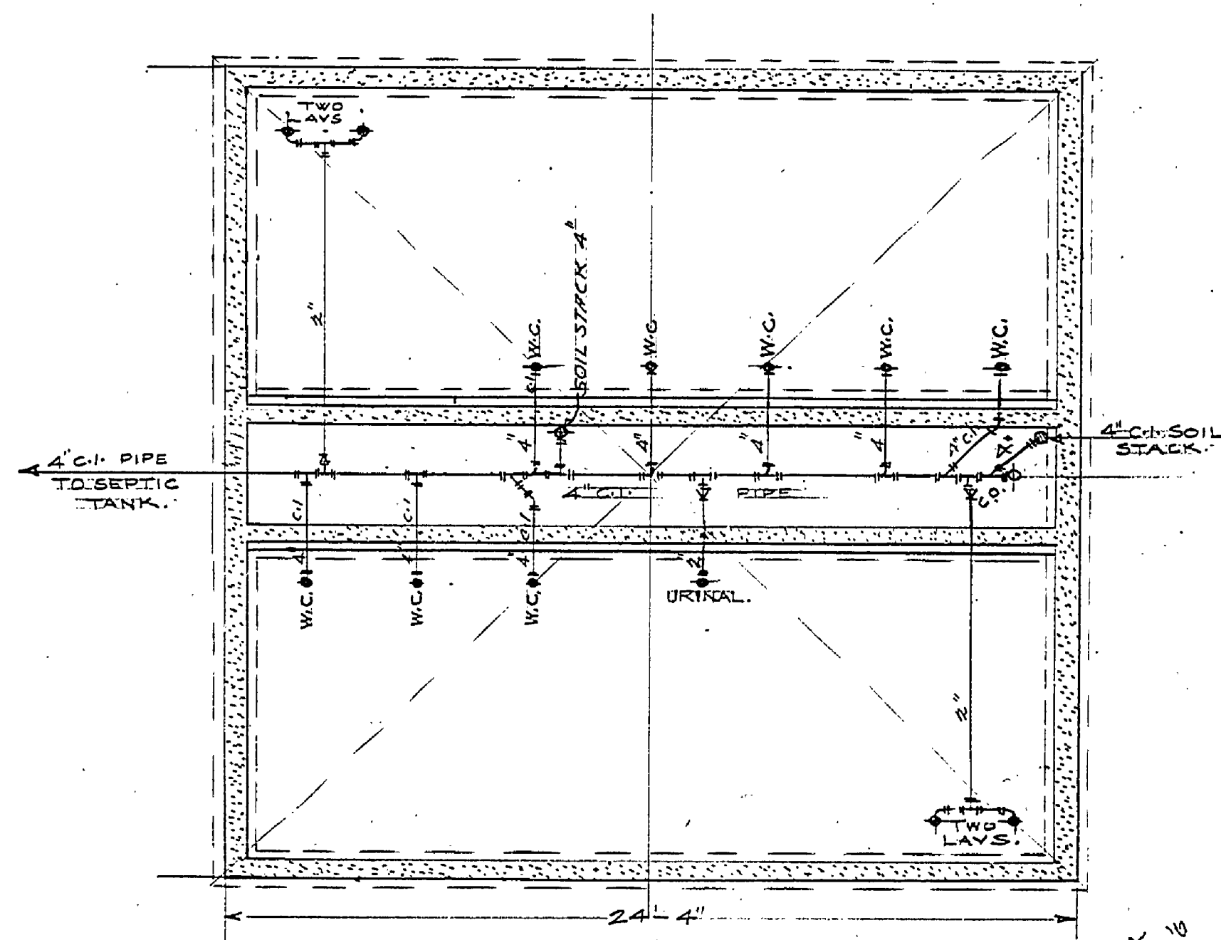
PIPING PLAN
