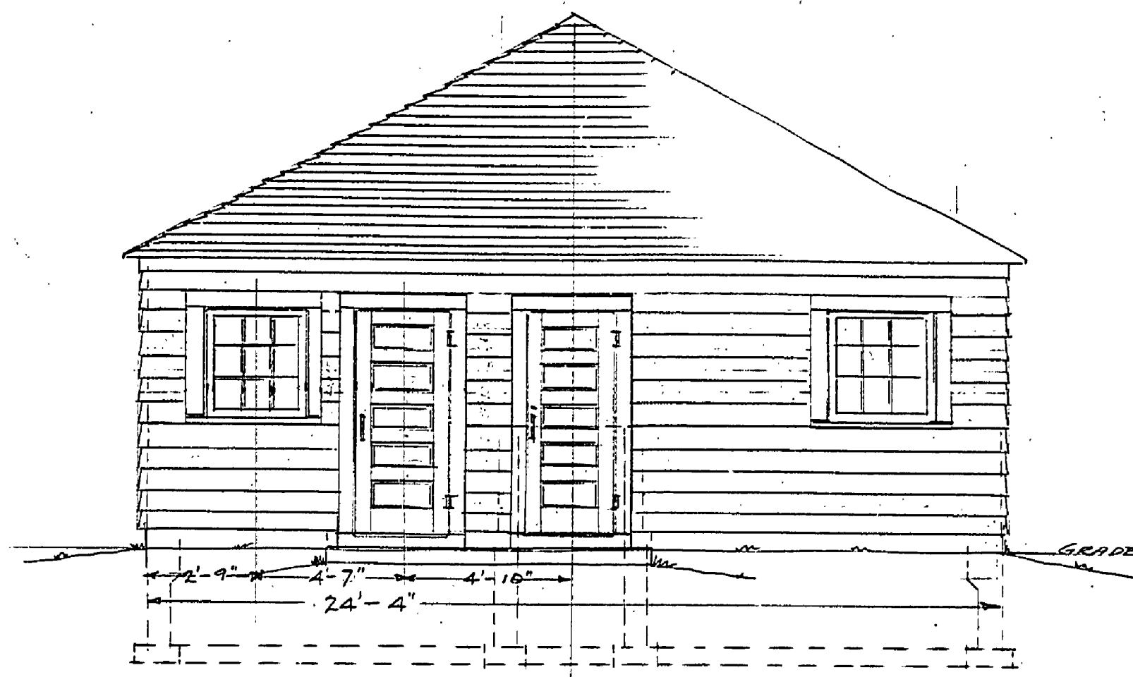
END ELEVATION SHOWING ENTRANCE TO PIPE PASSAGE
