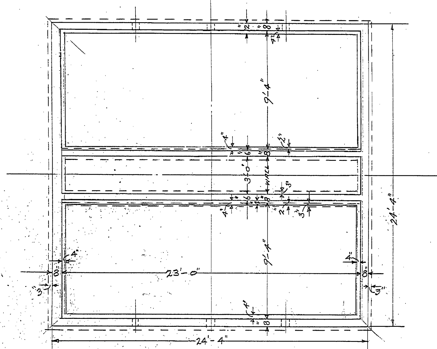
FOUNDATION PLAN
