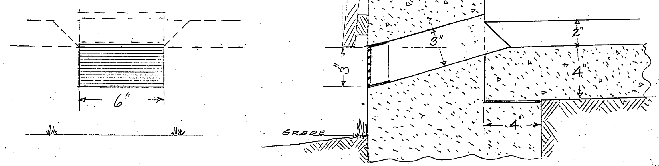
DETAIL OF SCUPPERS
