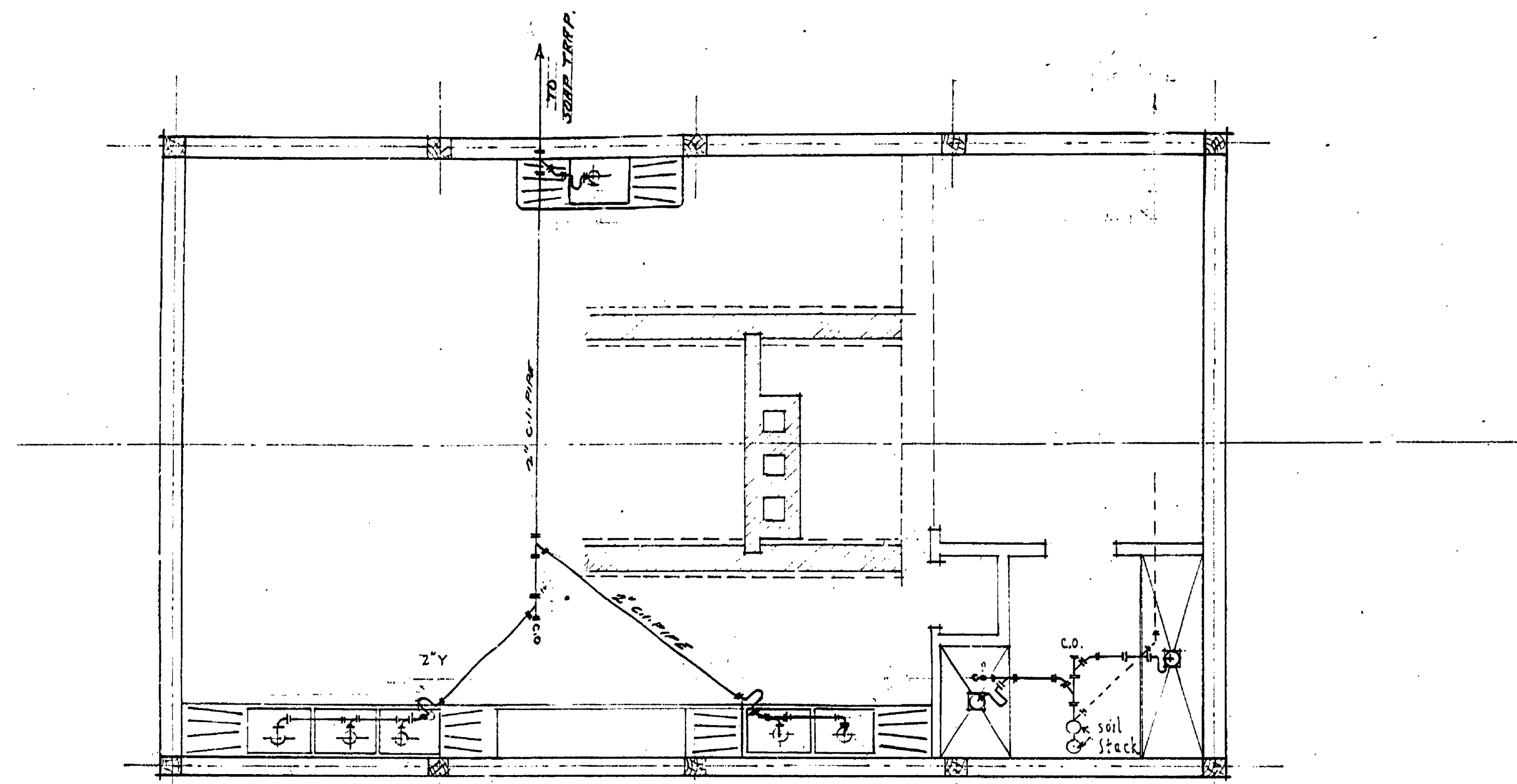
FIRST FLOOR PLUMBING PLAN
