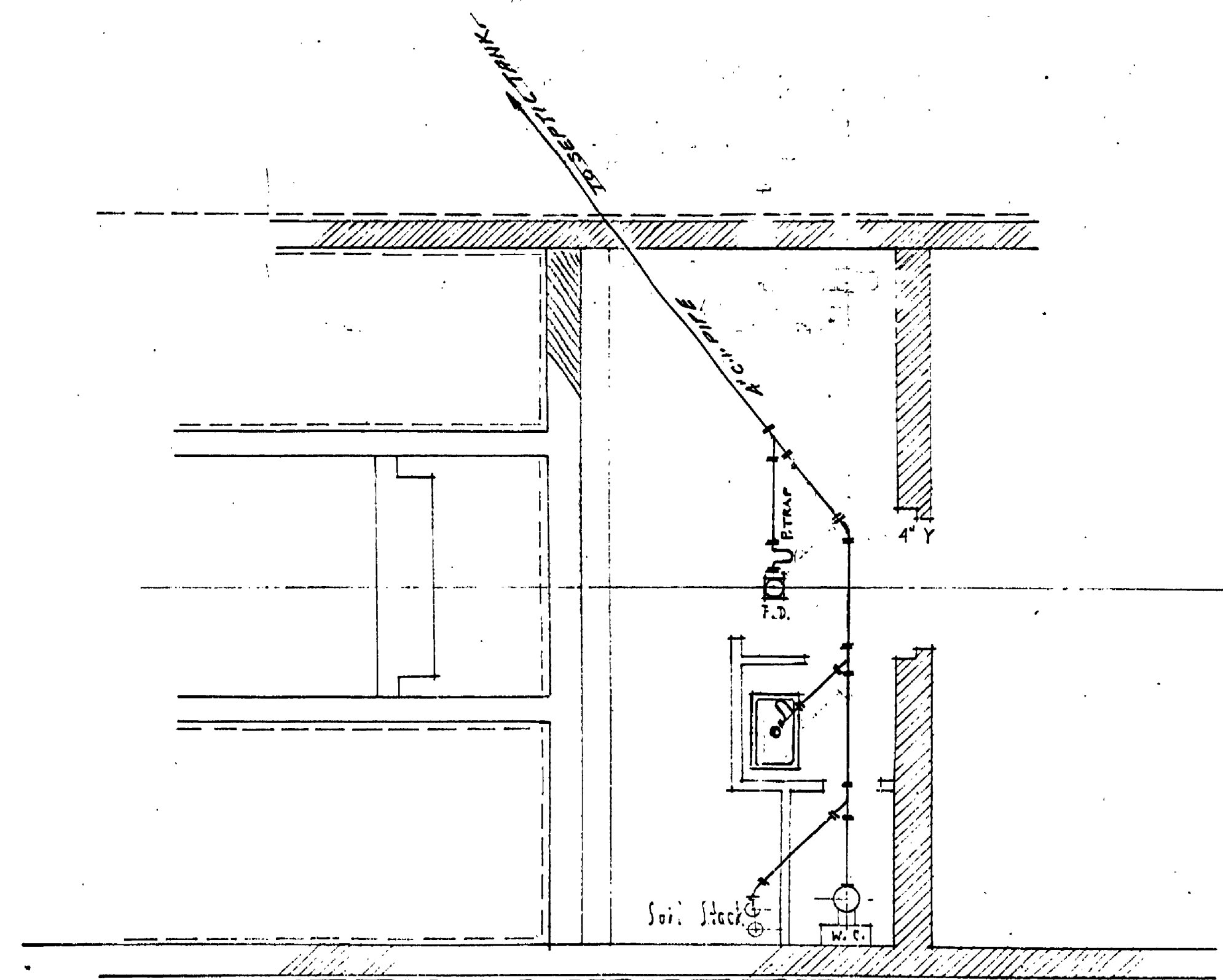
BASEMENT PLUMBING PLAN
