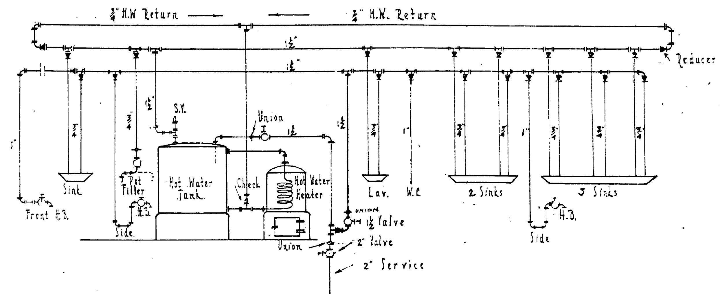
HOT AND COLD WATER DIAGRAM
