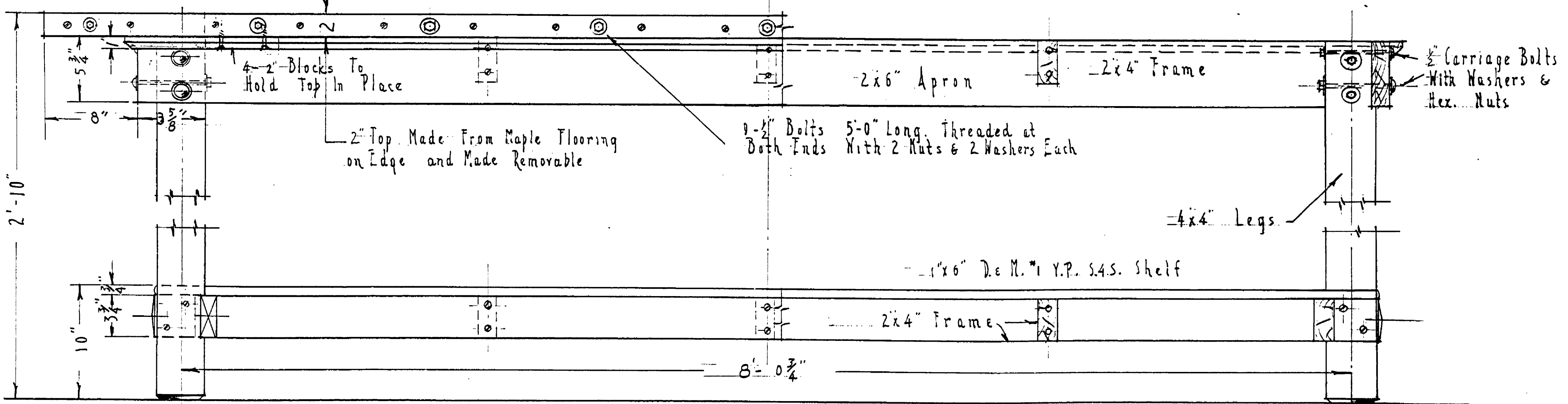
SIDE ELEVATION and SECTION A-A Scale 2" = 1'-0"
