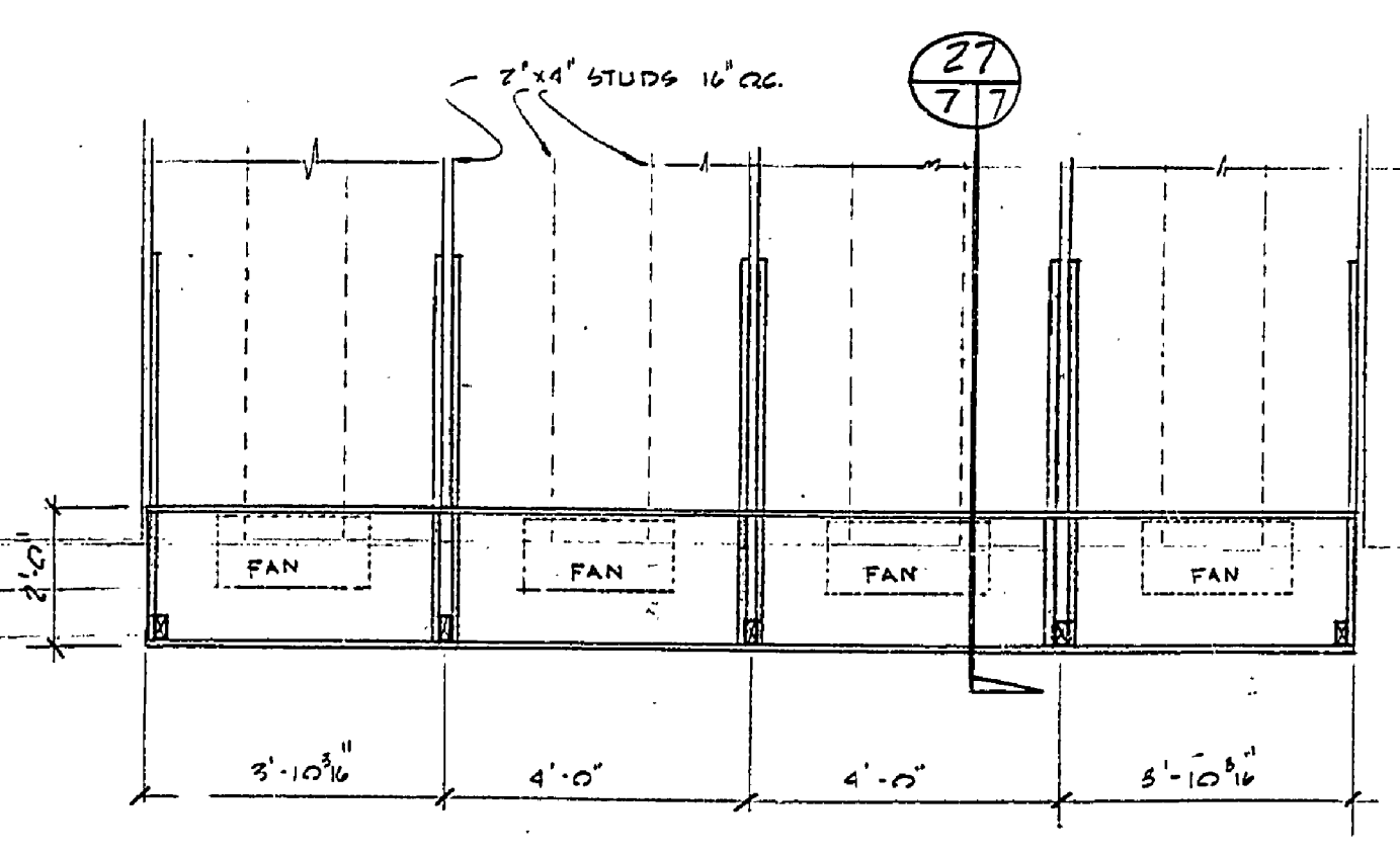
HOOD FRAMING DETAIL SCALE 3/8"=1'-0"
