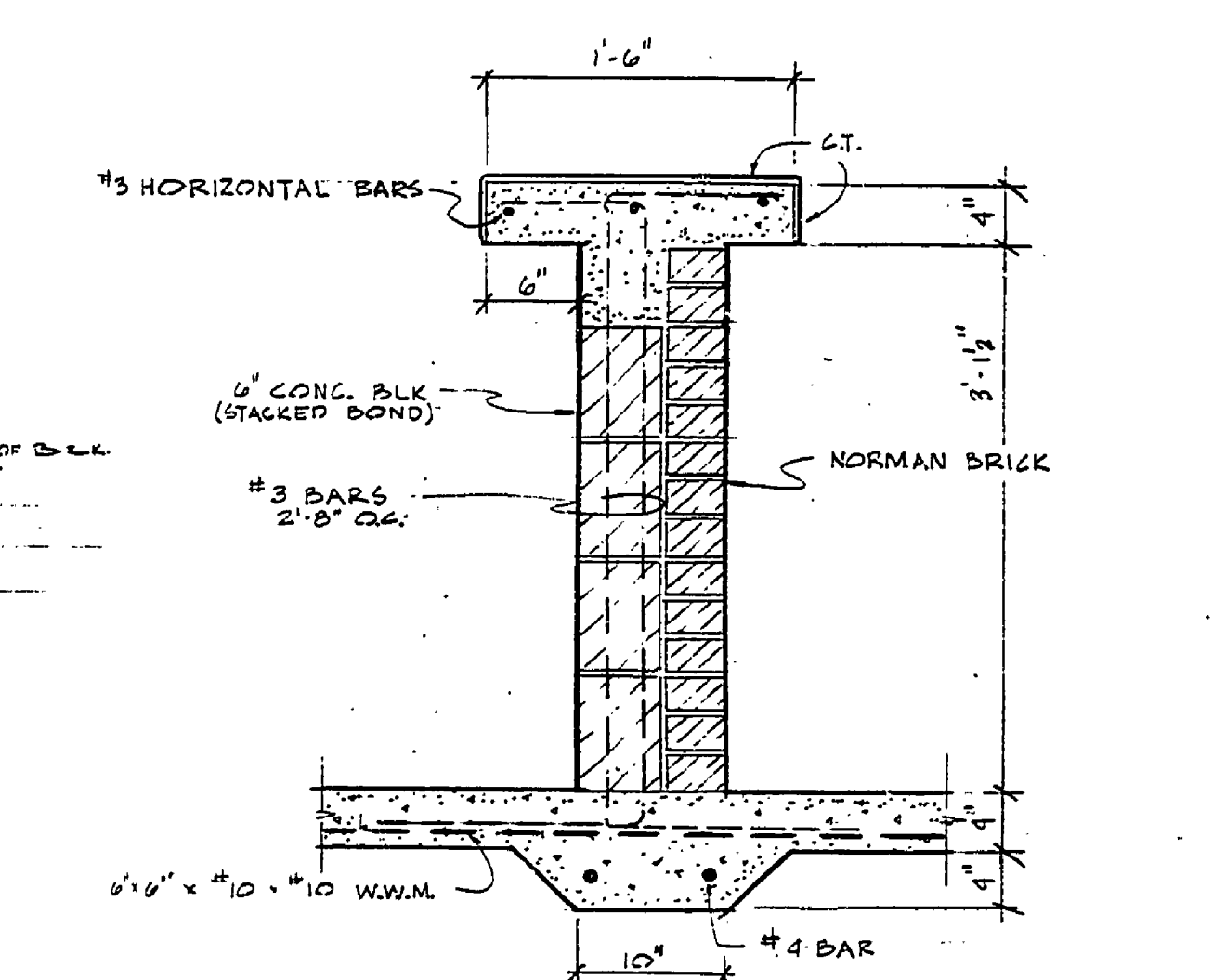
COUNTER SECTION SCALE 1"=1'-0"
