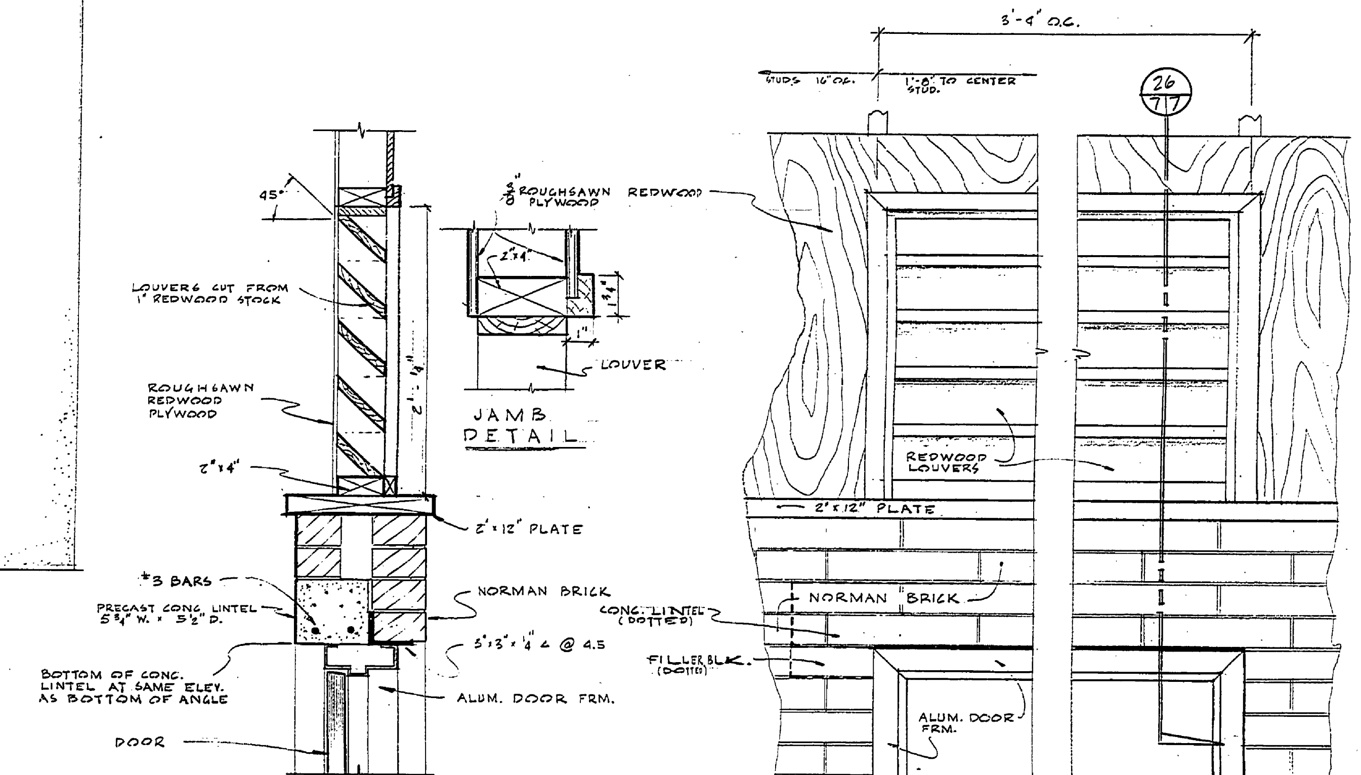
SECTION 20 SCALE 1/2"=1'-0"
