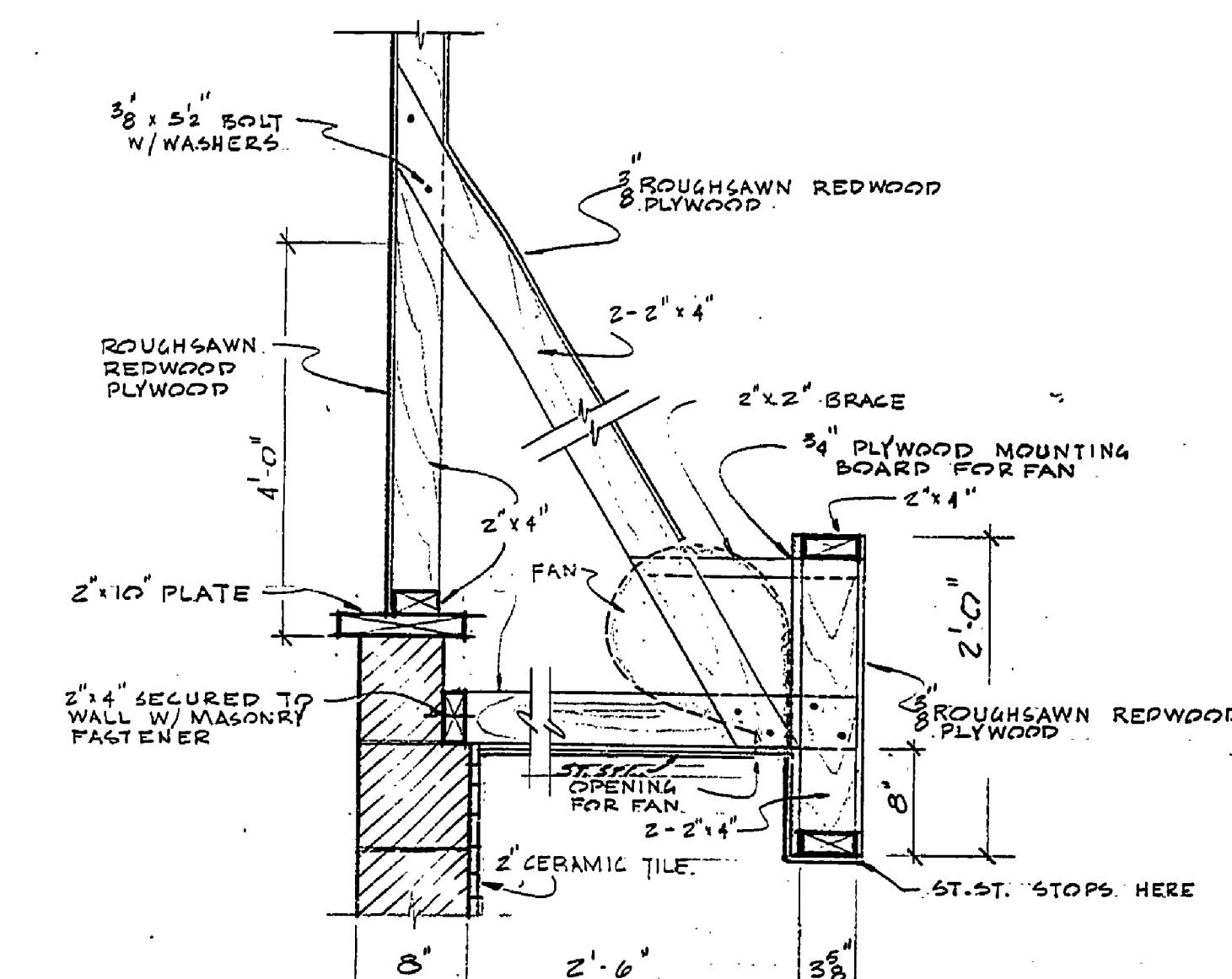
SECTION 27 SCALE 1"=1'-0"
