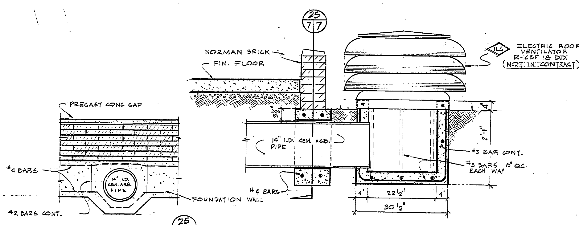
EXHAUST FAN INSTALLATION DETAIL SCALE 3/4"=1'-0"
