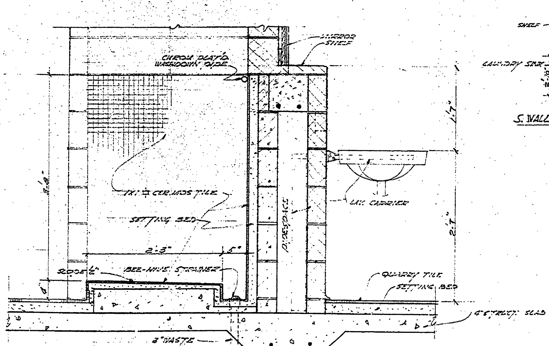
DET. 9/25 SCALE 1/4" = 1'-0"
