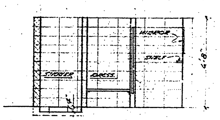
SMALL ELEV. WOMEN'S SHOWER SCALE 1/4" = 1'-0"
