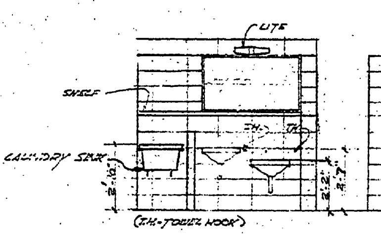
SMALL ELEV. WOMEN'S TOILET SCALE 1/4" = 1'-0"
