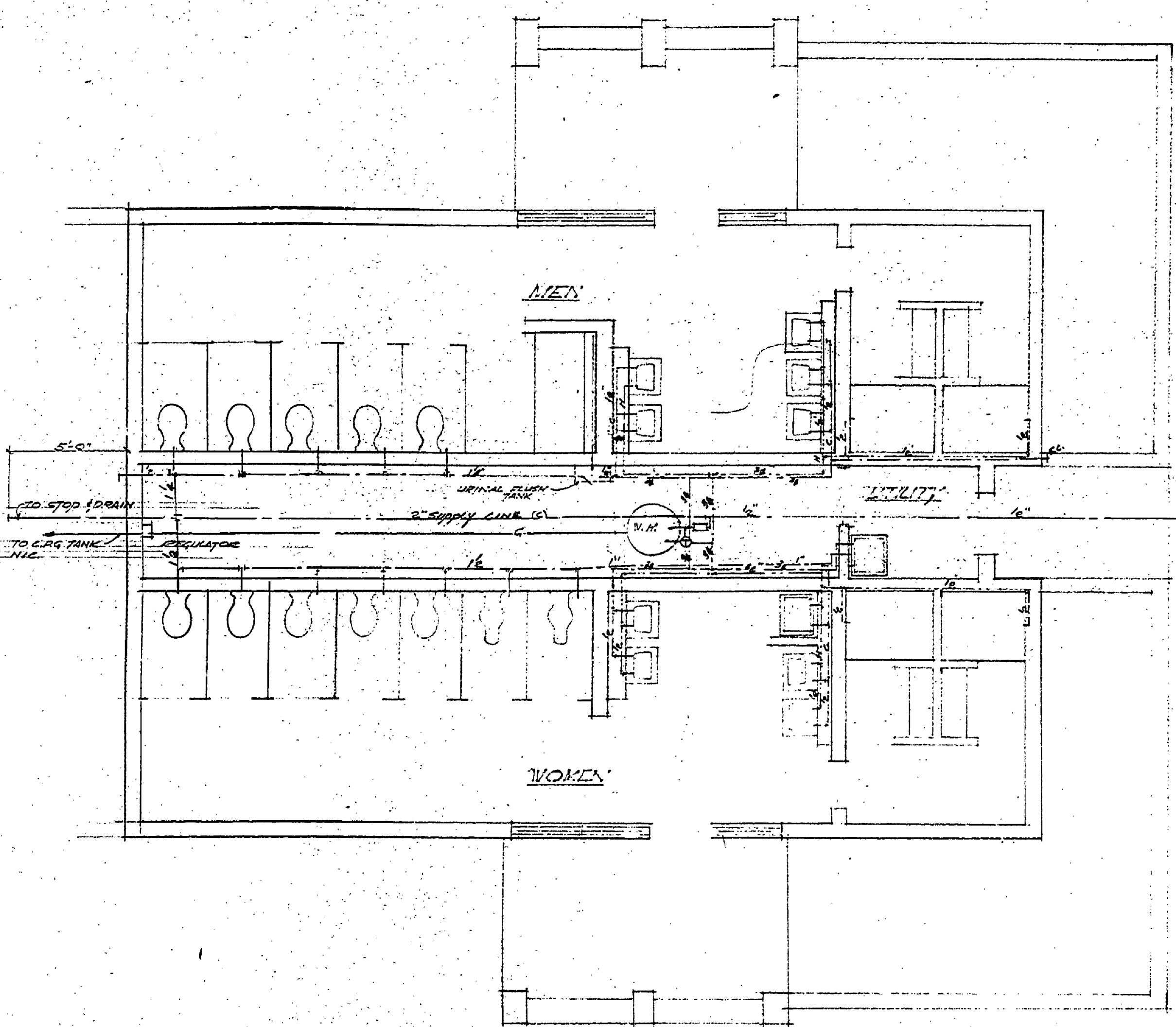
PLUMBING PLAN SCALE 1/4" = 1'-0"
