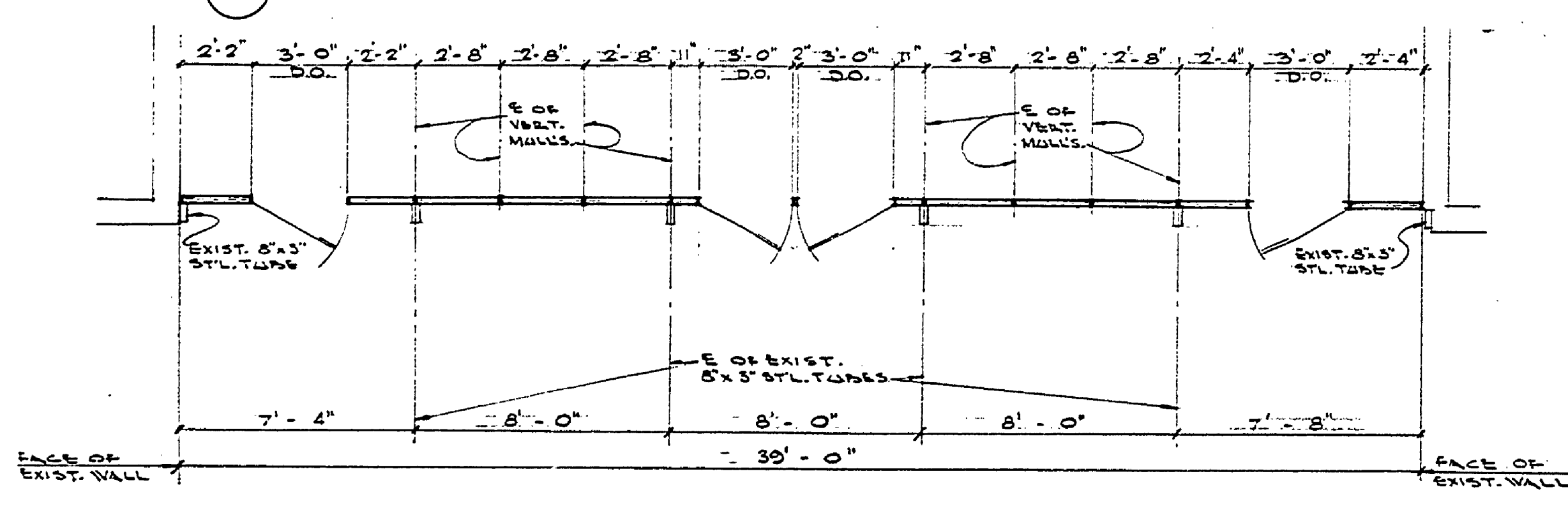
PLAN - CONCESSION INSECT SCREENING 1/4\"/>
