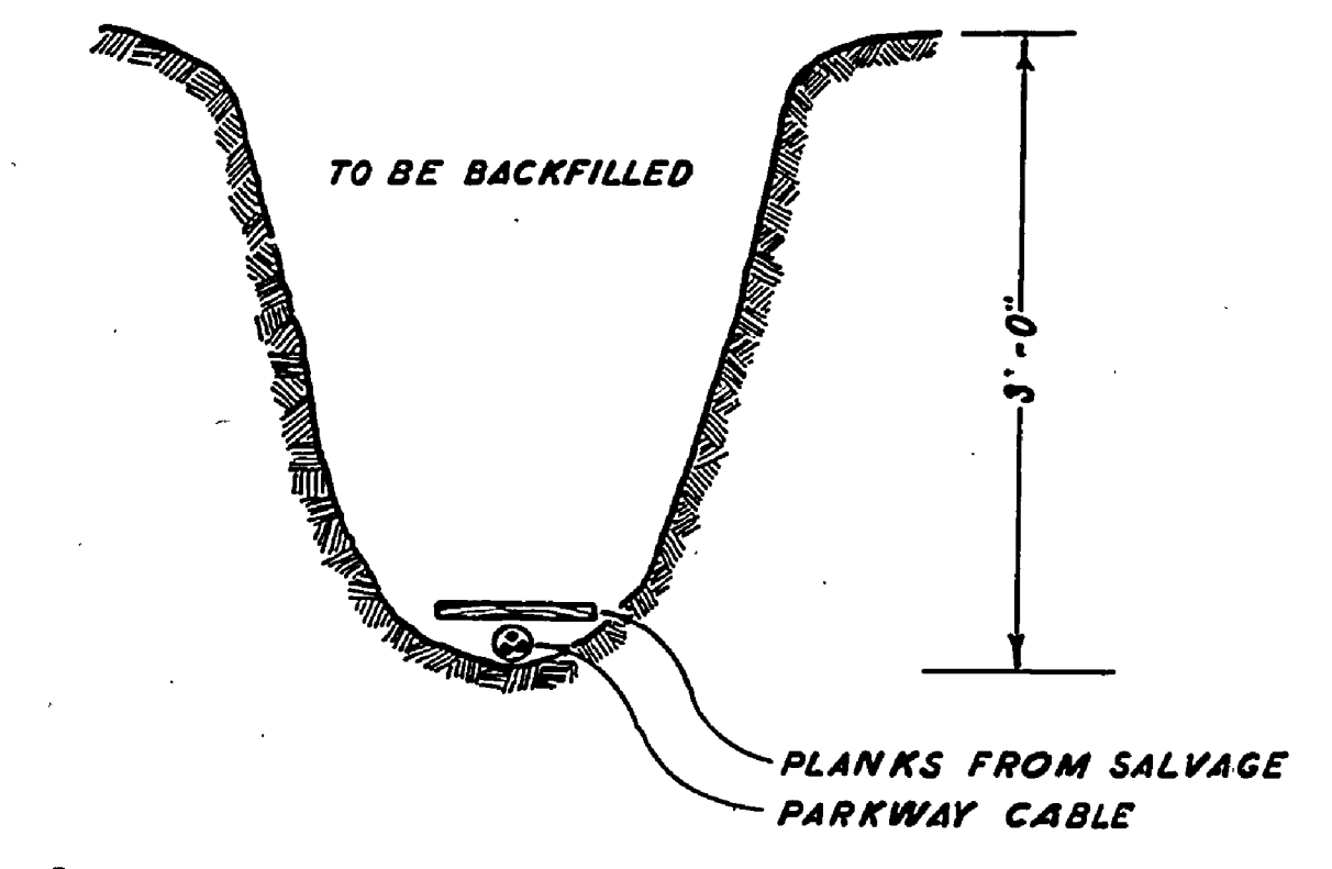
CROSS SECTION OF CONDUIT TRENCH
