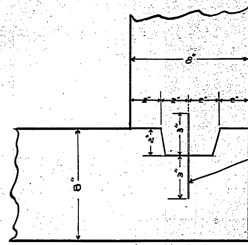
CONSTRUCTION JOINT
