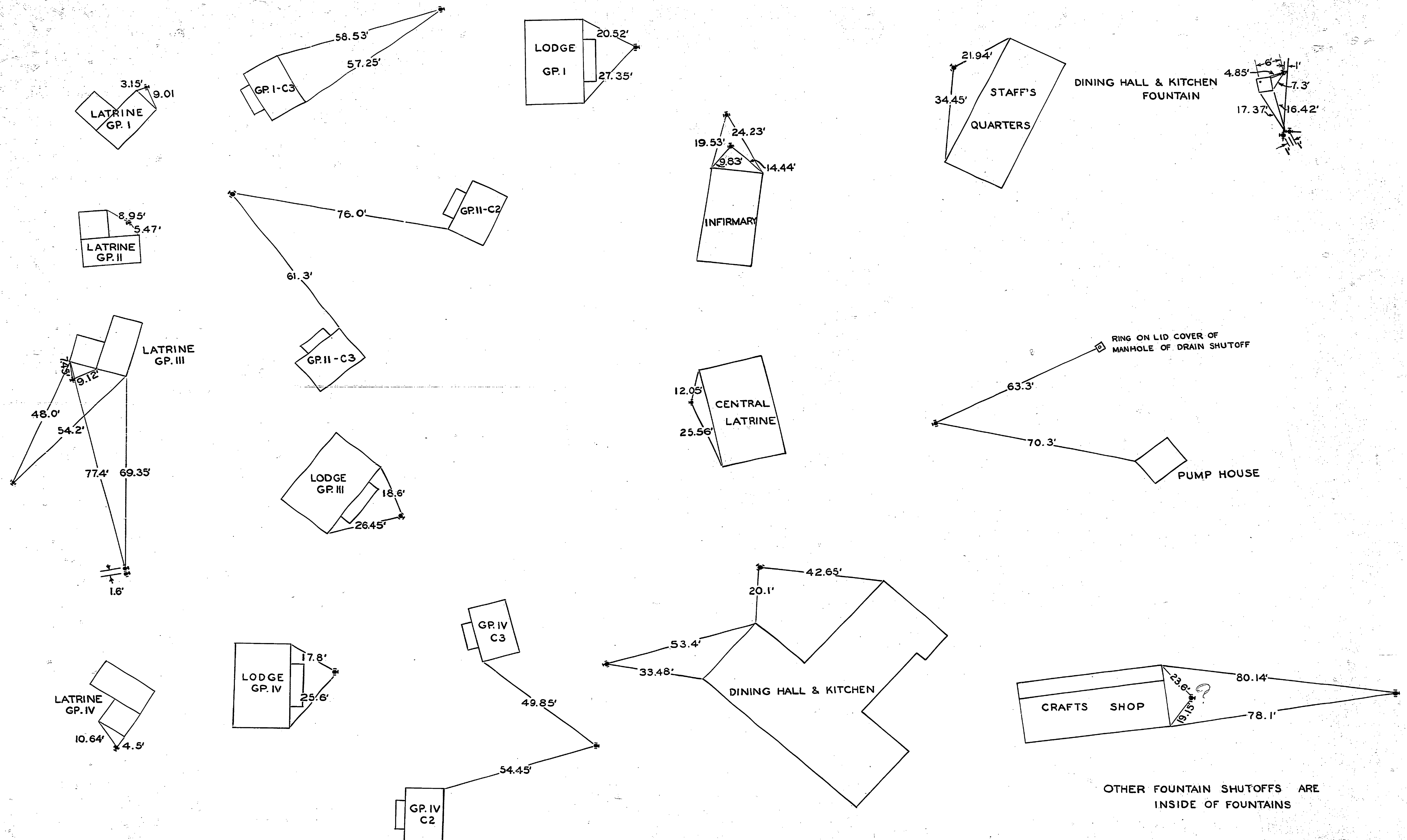
TIES FOR LOCATION OF VALVES IN WATERLINES - C-1 NOONDAY LAKE
