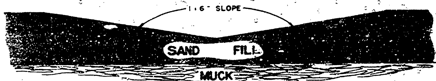
TYPICAL DITCH SECTION SECTION B-B
