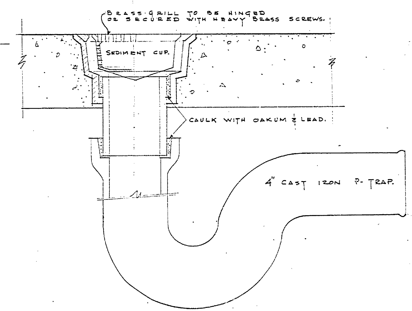
DETAIL OF FLOOR DRAINS
