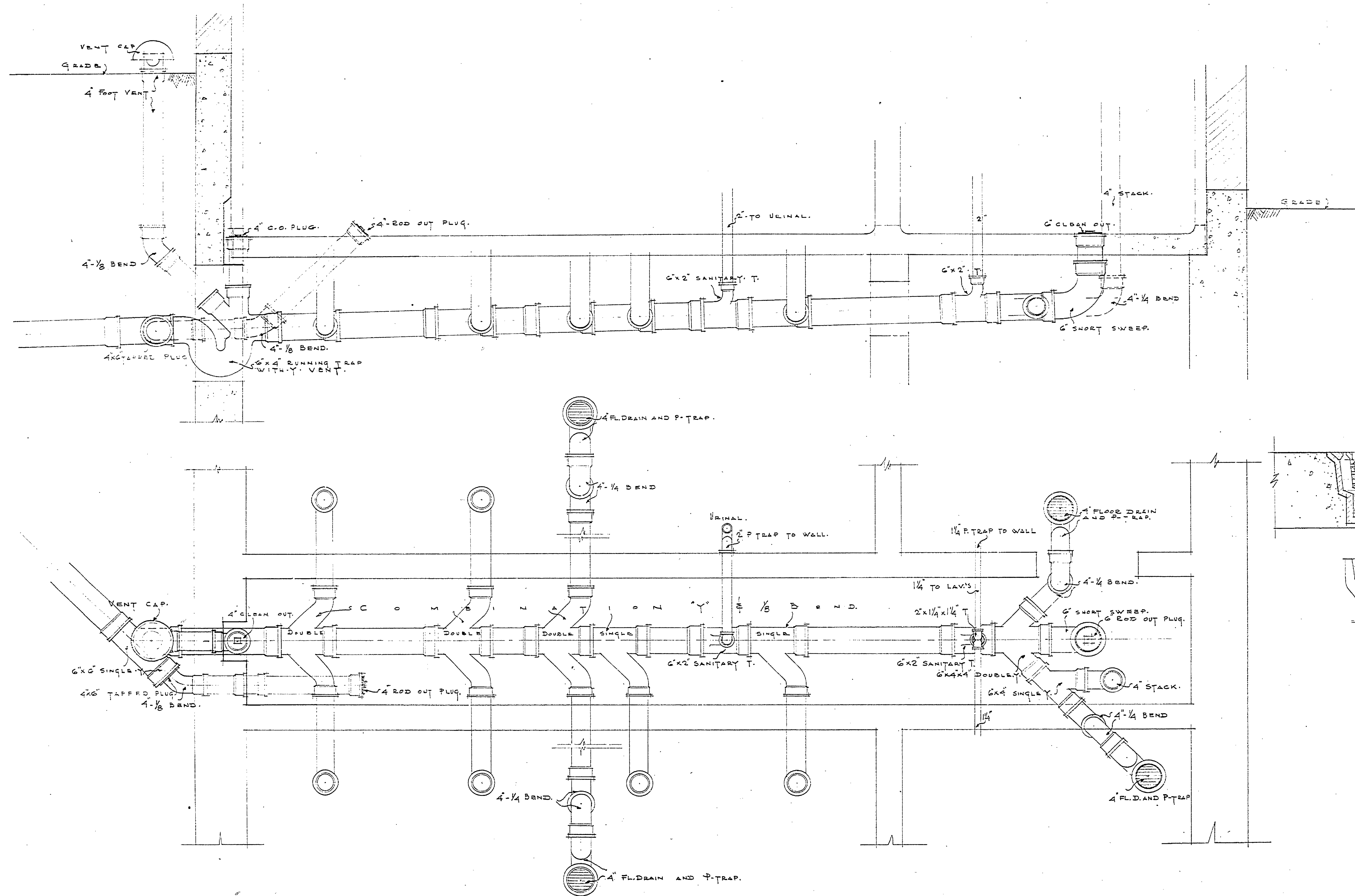
DRAINAGE LAYOUT SCALE 1" = 1'-0"
