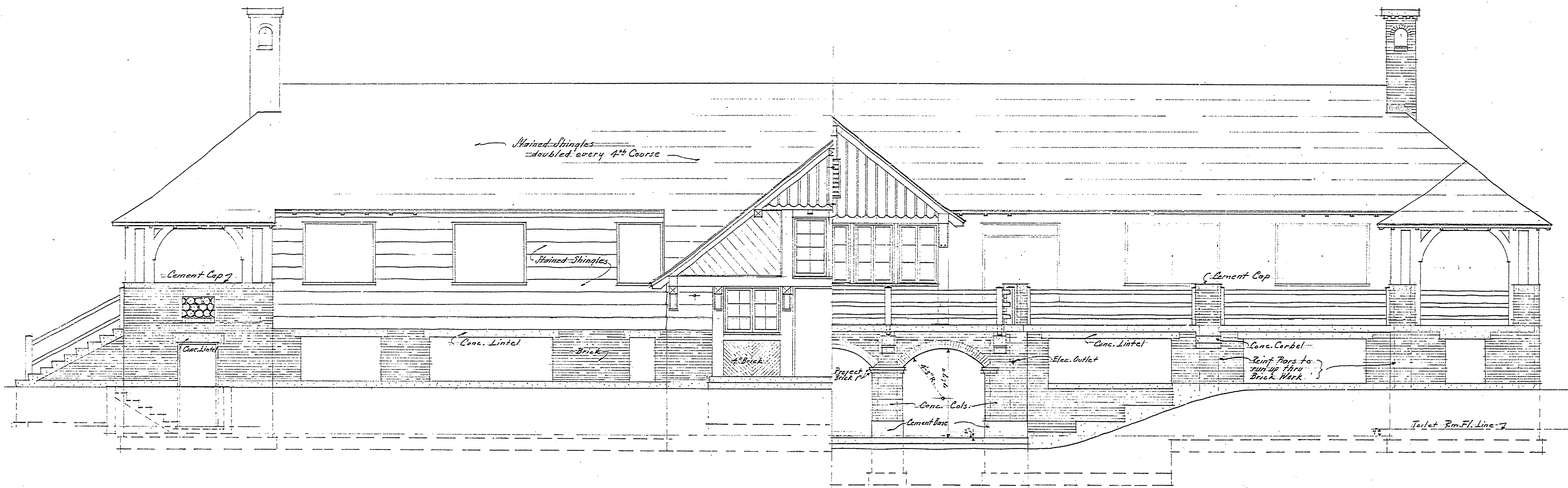
ONE-HALF OF ENTRANCE ELEVATION
