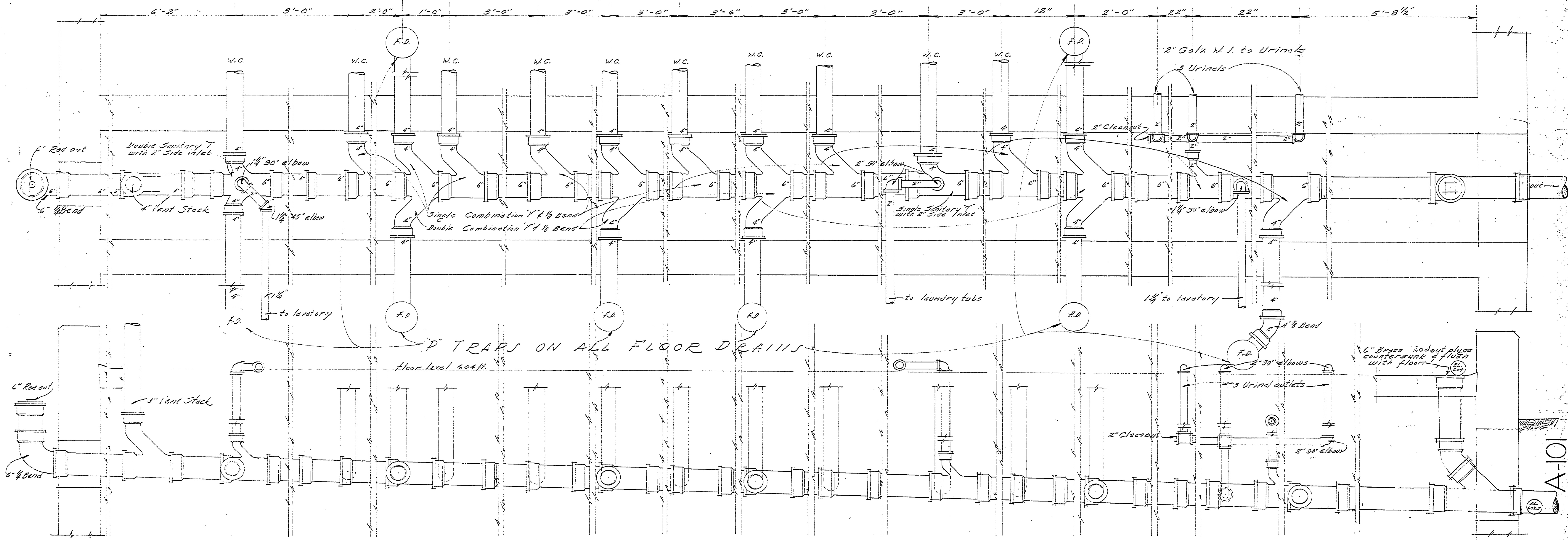
DETAILED LAYOUT OF DRAINAGE SYSTEM SCALE 1"=1'-0"
