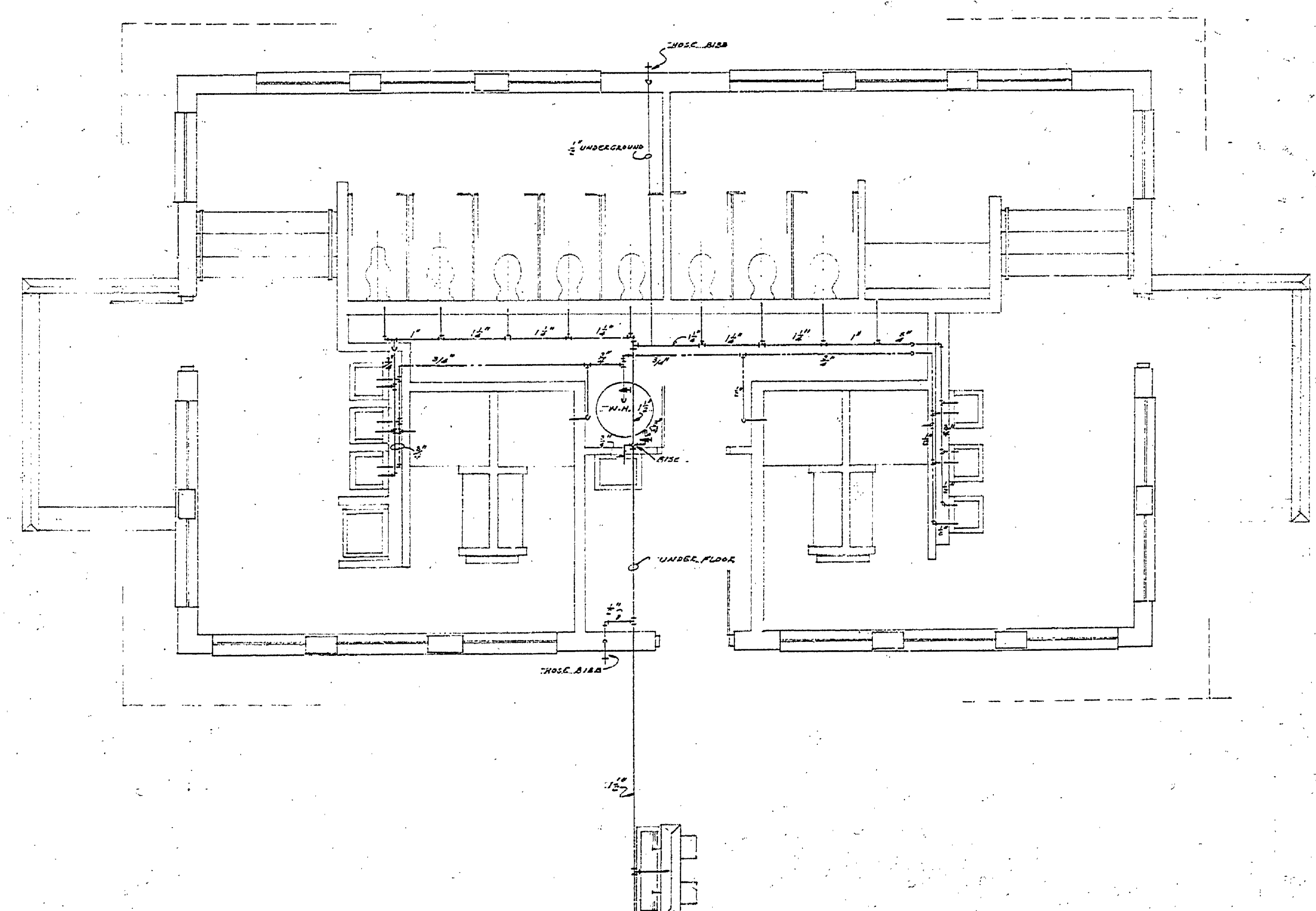
PLUMBING PLAN SCALE 1/4" = 1'-0"
