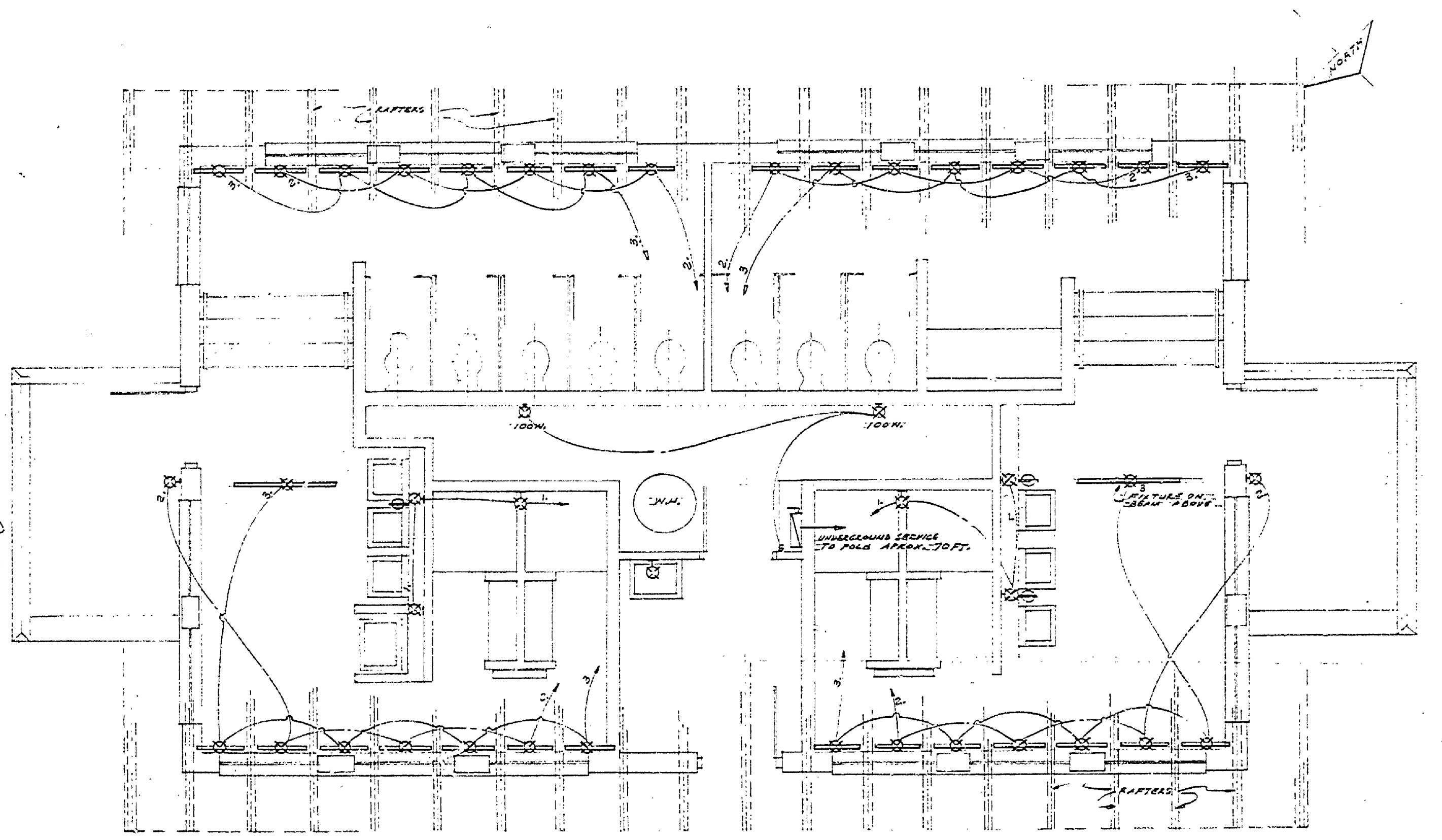
ELECTRICAL PLAN SCALE 1/4" = 1'-0"
