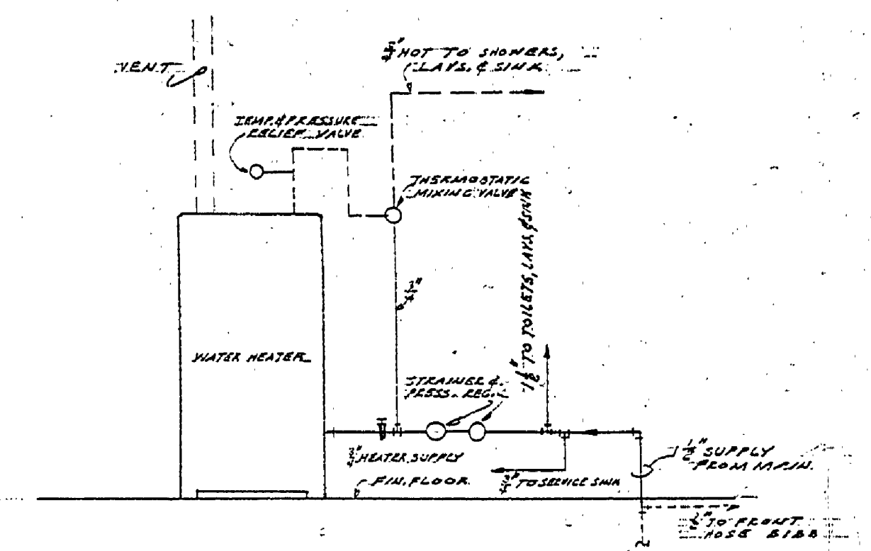
WATER HEATER PIPING NO SCALE
