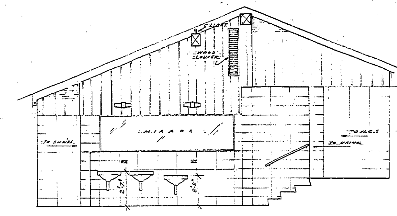
S.E. WALL - MENS TOILET SCALE 1/4" = 1'-0"
