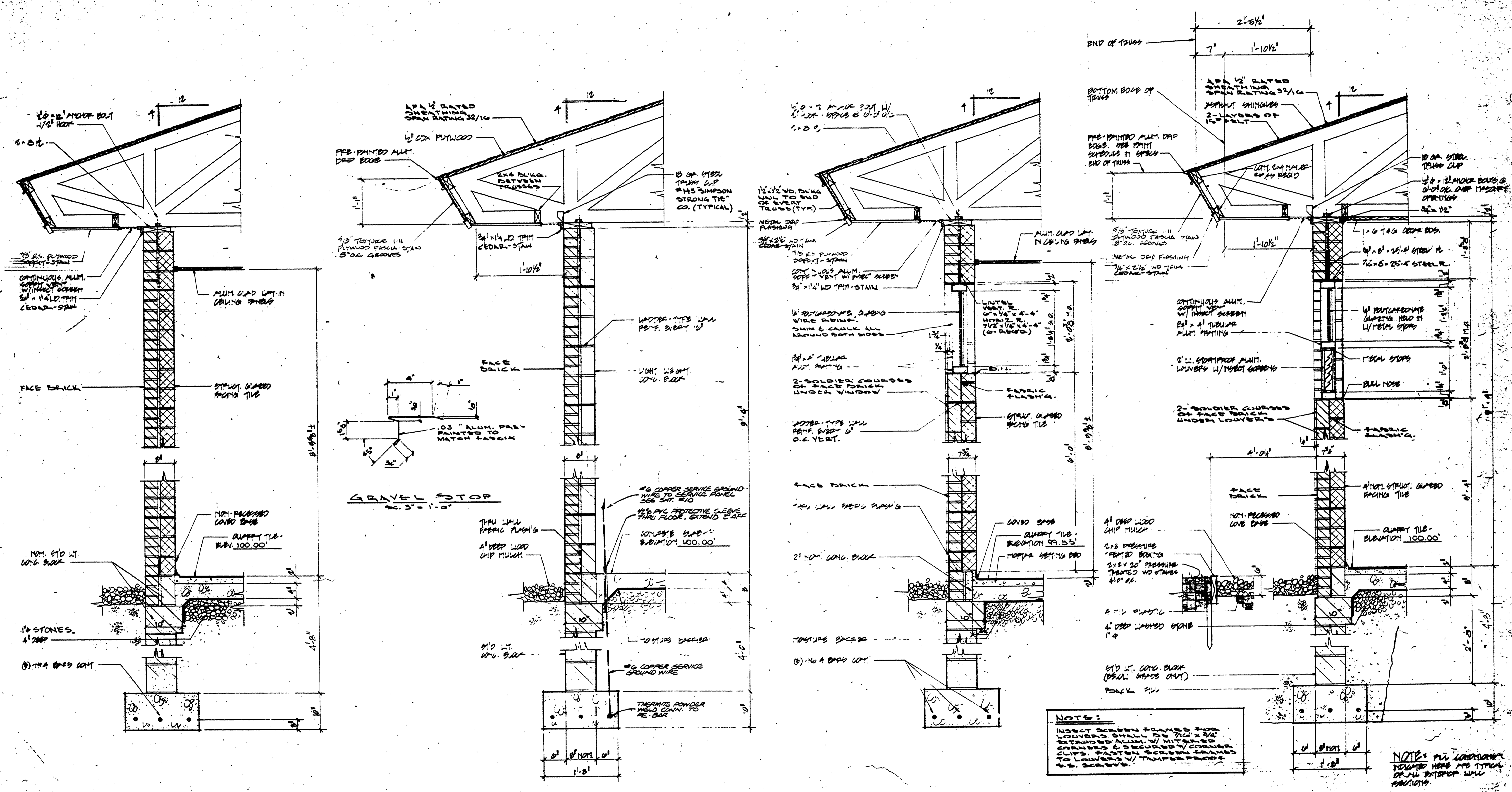
WALL SECTION 1
