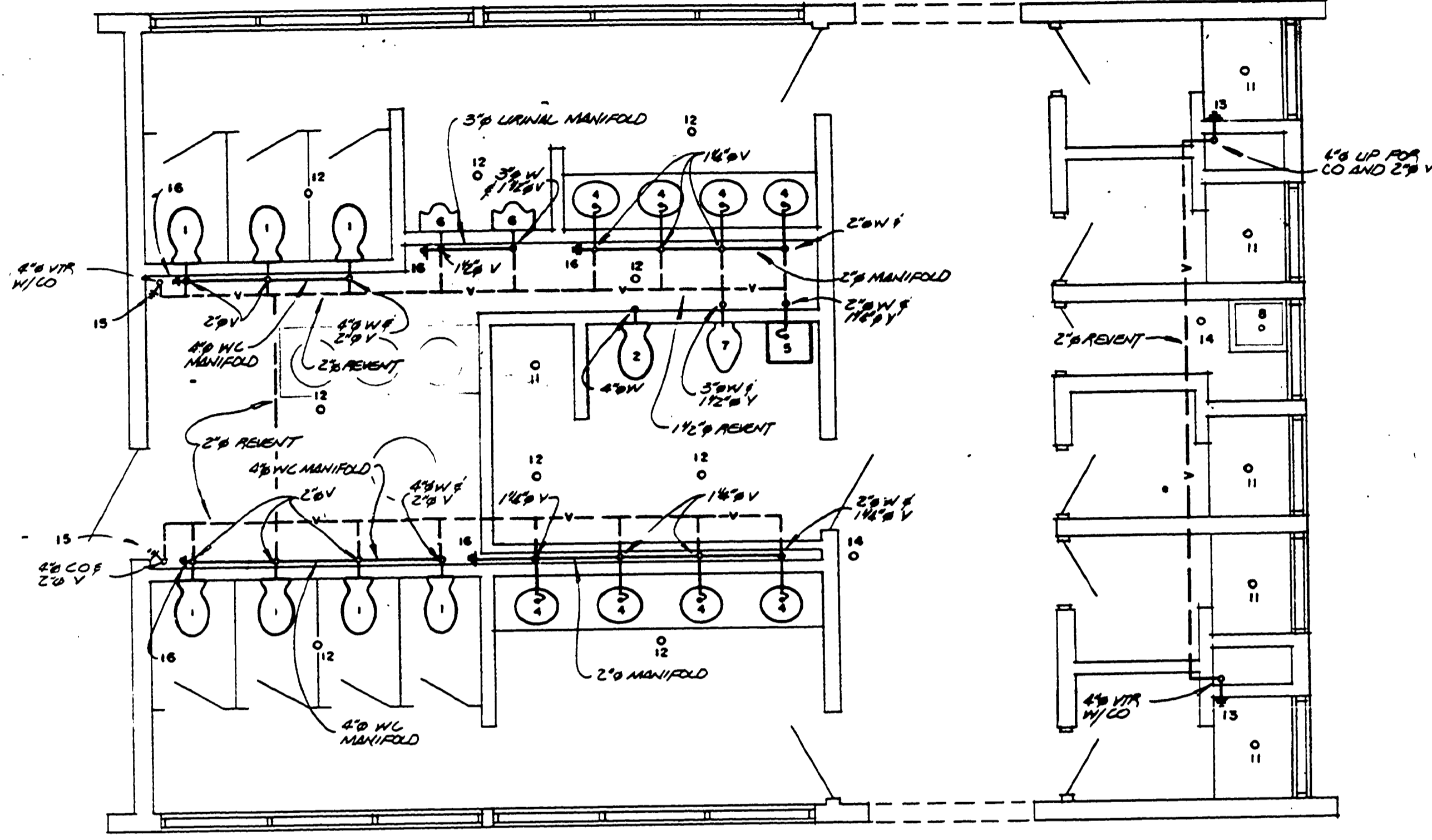
ABOVE SLAB WASTE PLUMBING PLAN SCALE 1/8" = 1'-0"
