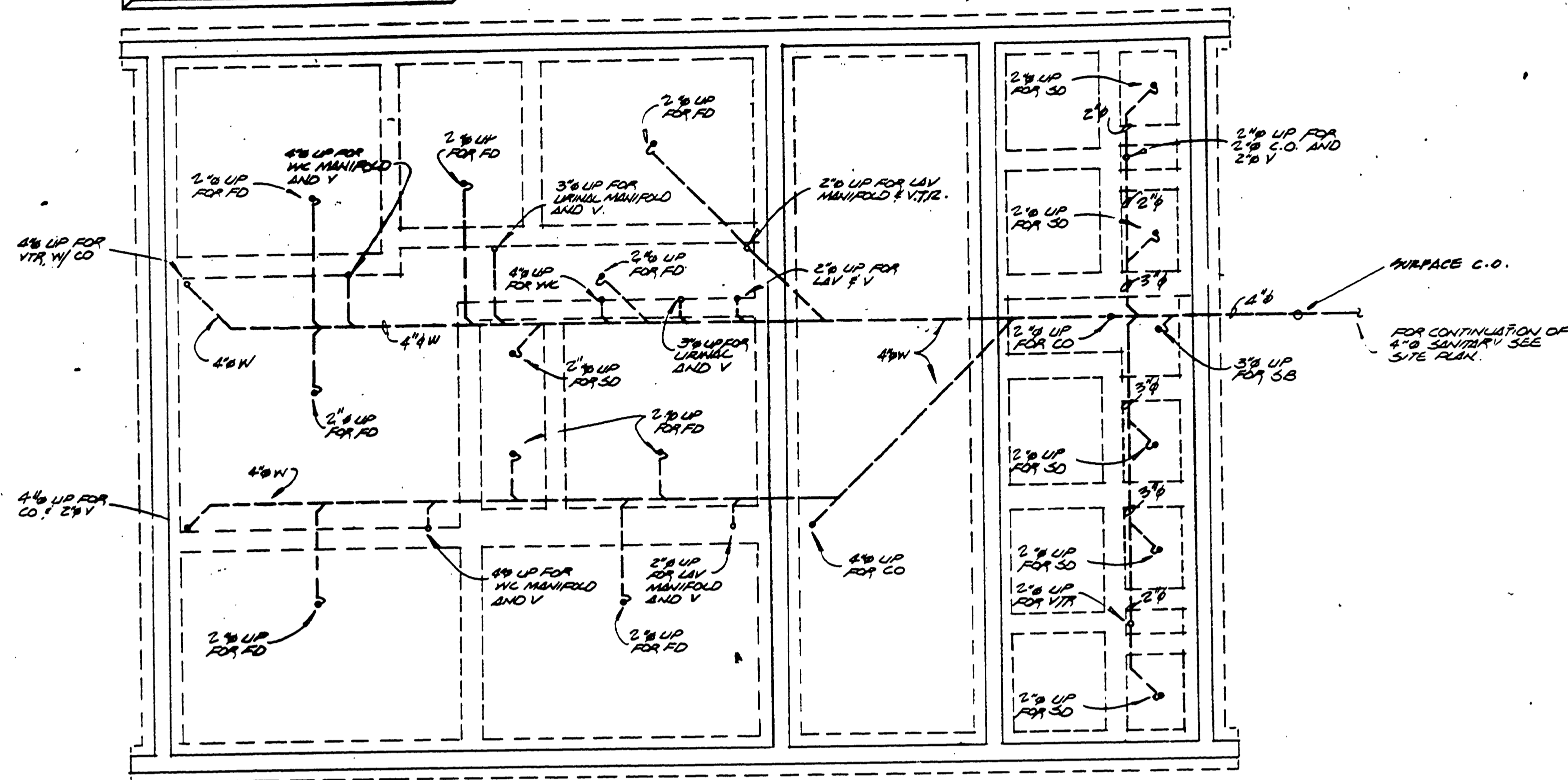
BELOW SLAB WASTE PLUMBING PLAN SCALE 1/8" = 1'-0"
