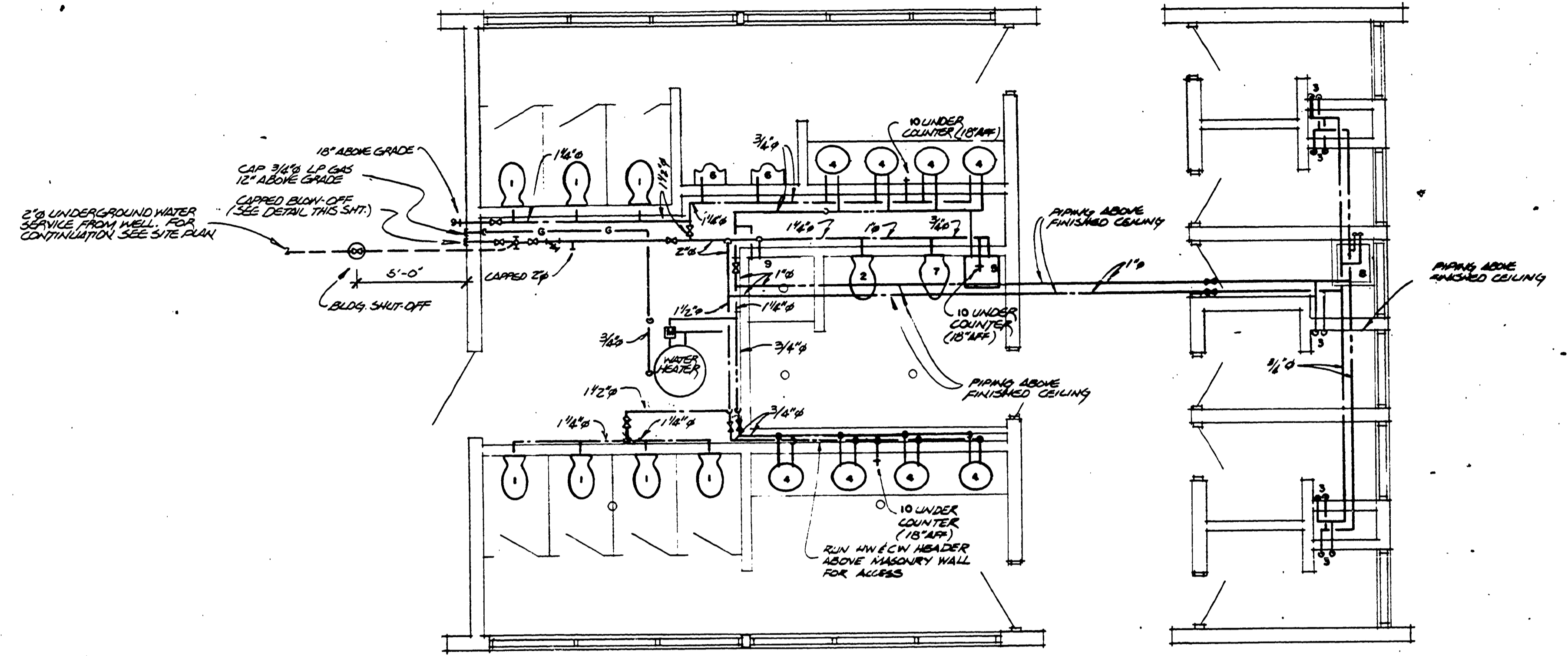
DOMESTIC WATER SUPPLY SYSTEM PIPING SCALE 1/4" = 1'-0"
