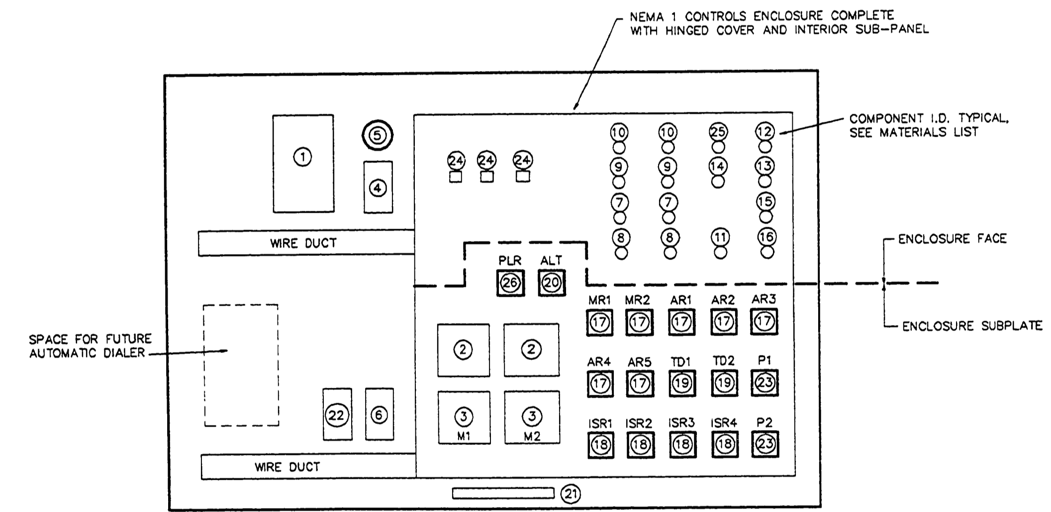
TYPICAL SUB-PANEL LAYOUT - SERVICE ENCLOSURE DETAIL NO SCALE
