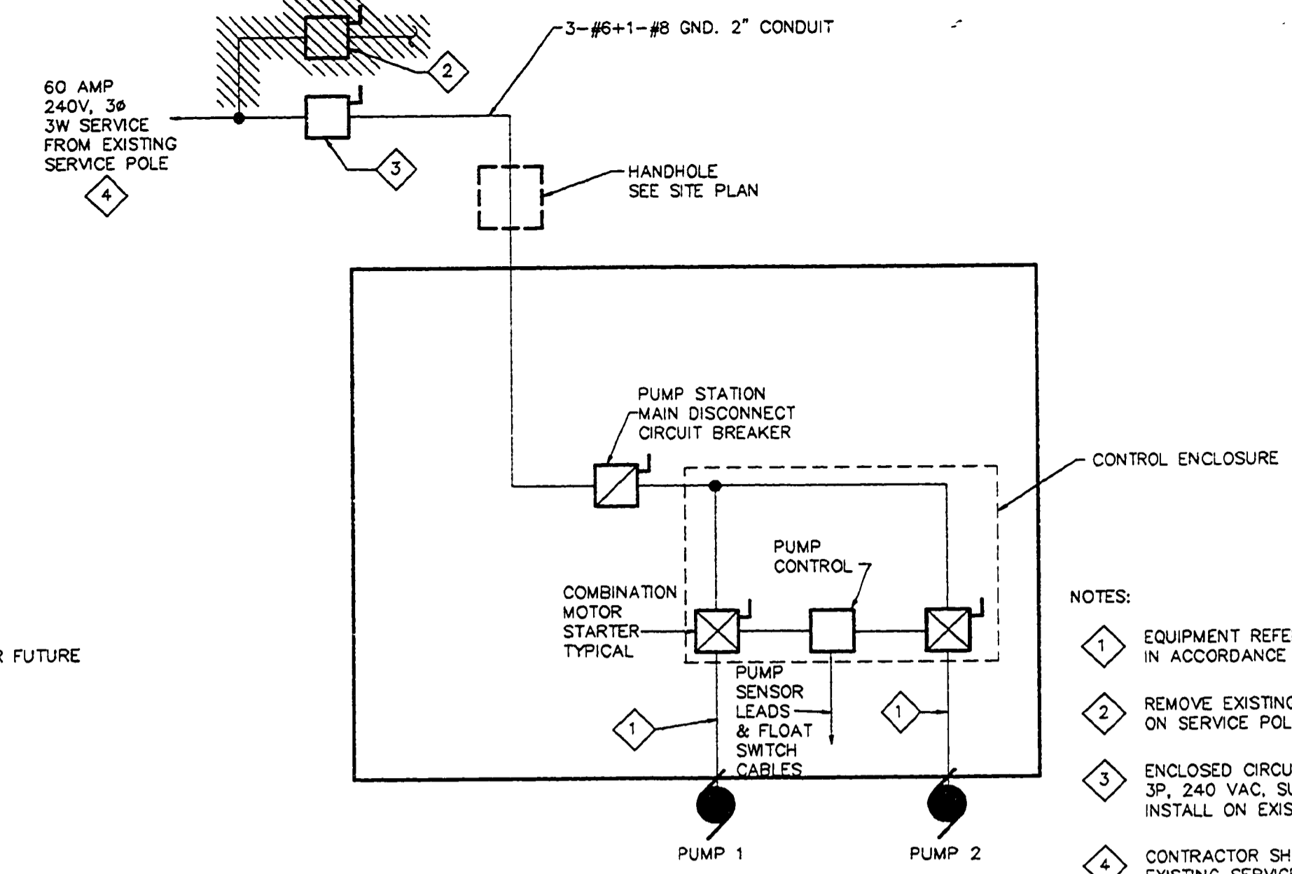
ONE-LINE DIAGRAM 240V 3Ø - 3W
