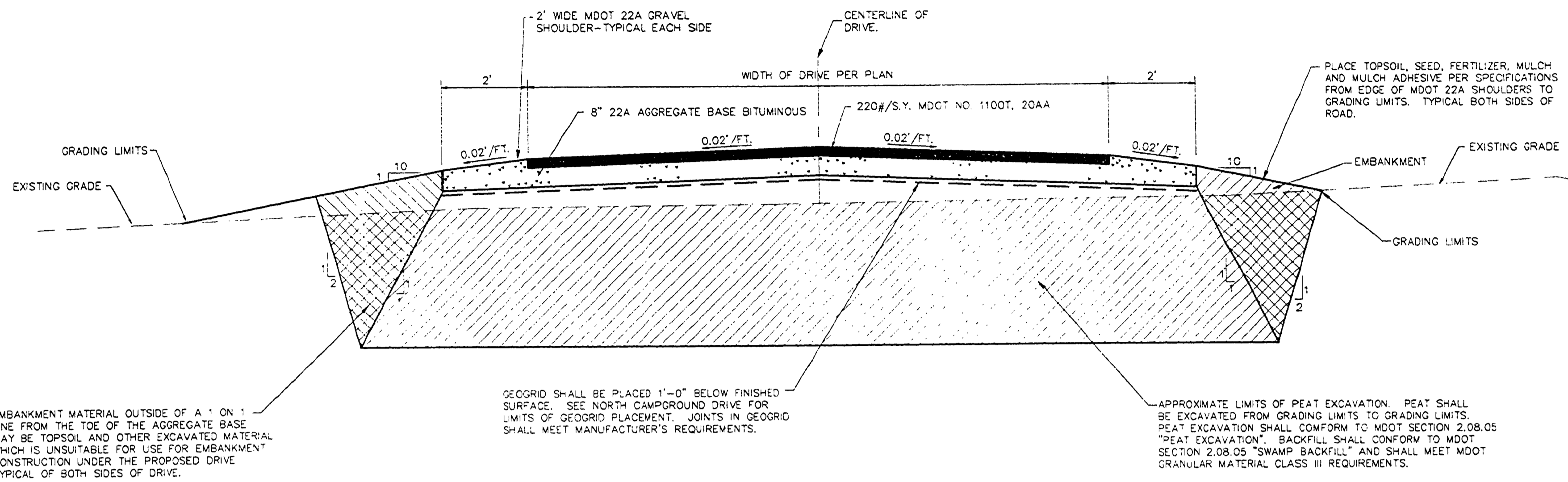
TYPICAL CROSS SECTION ENTRANCE DRIVE - PEAT EXCAVATION AREA NO SCALE
