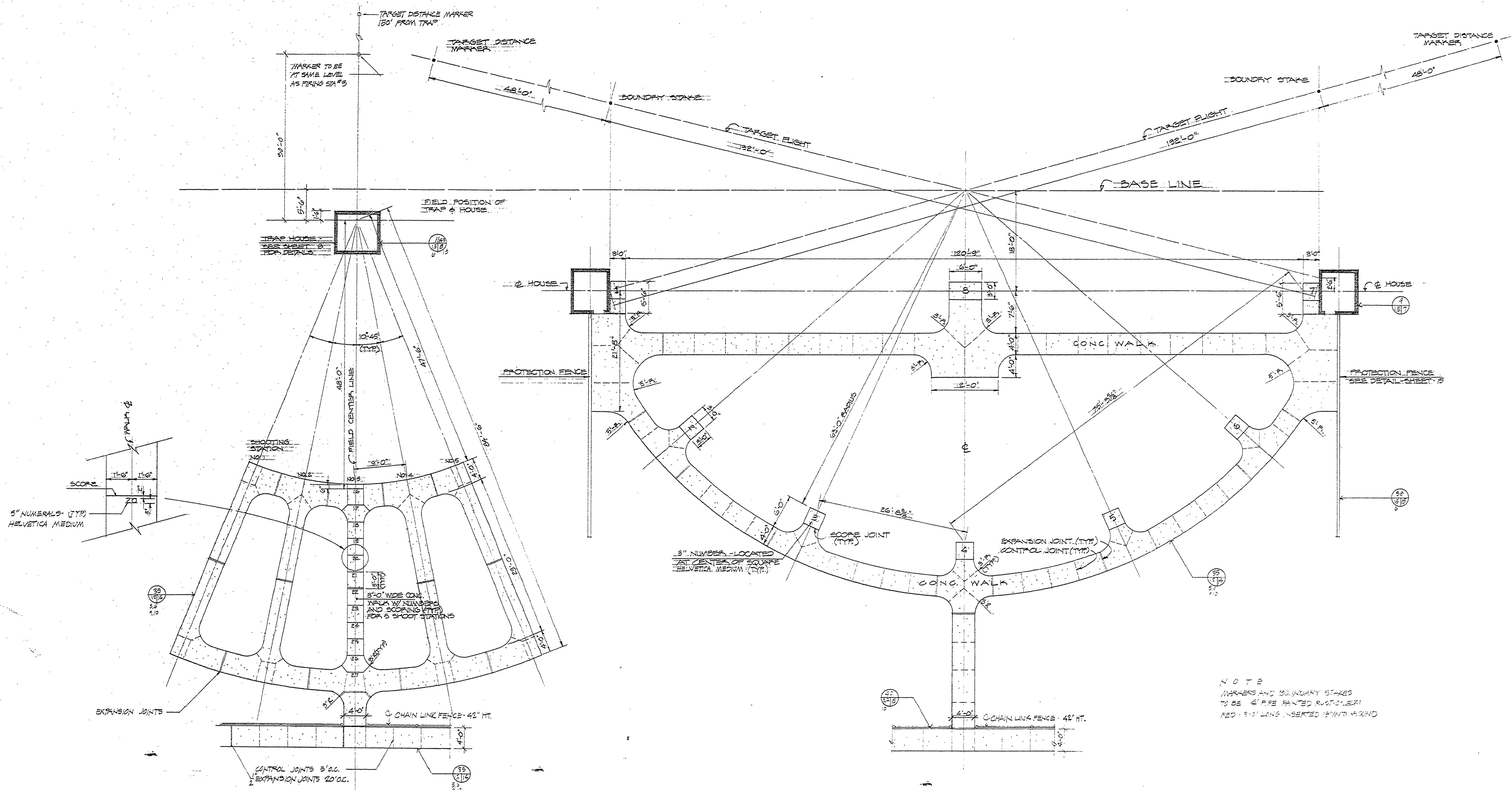
1 TRAP FIELD LAYOUT SCALE 1/8" = 1'-0"
