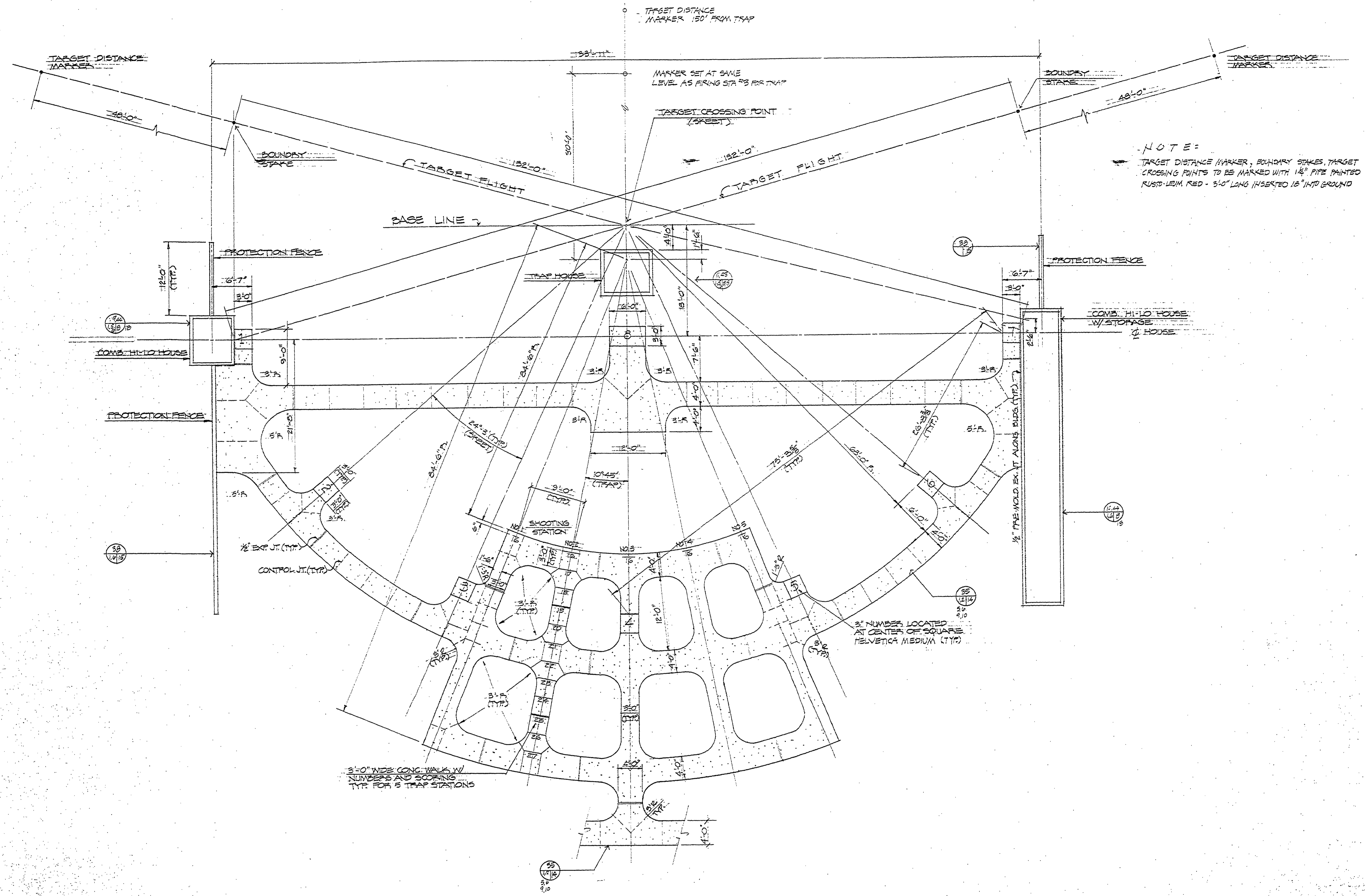
COMBINATION TRAP SKEET FIELD LAYOUT SCALE 1/8" = 1'-0"
