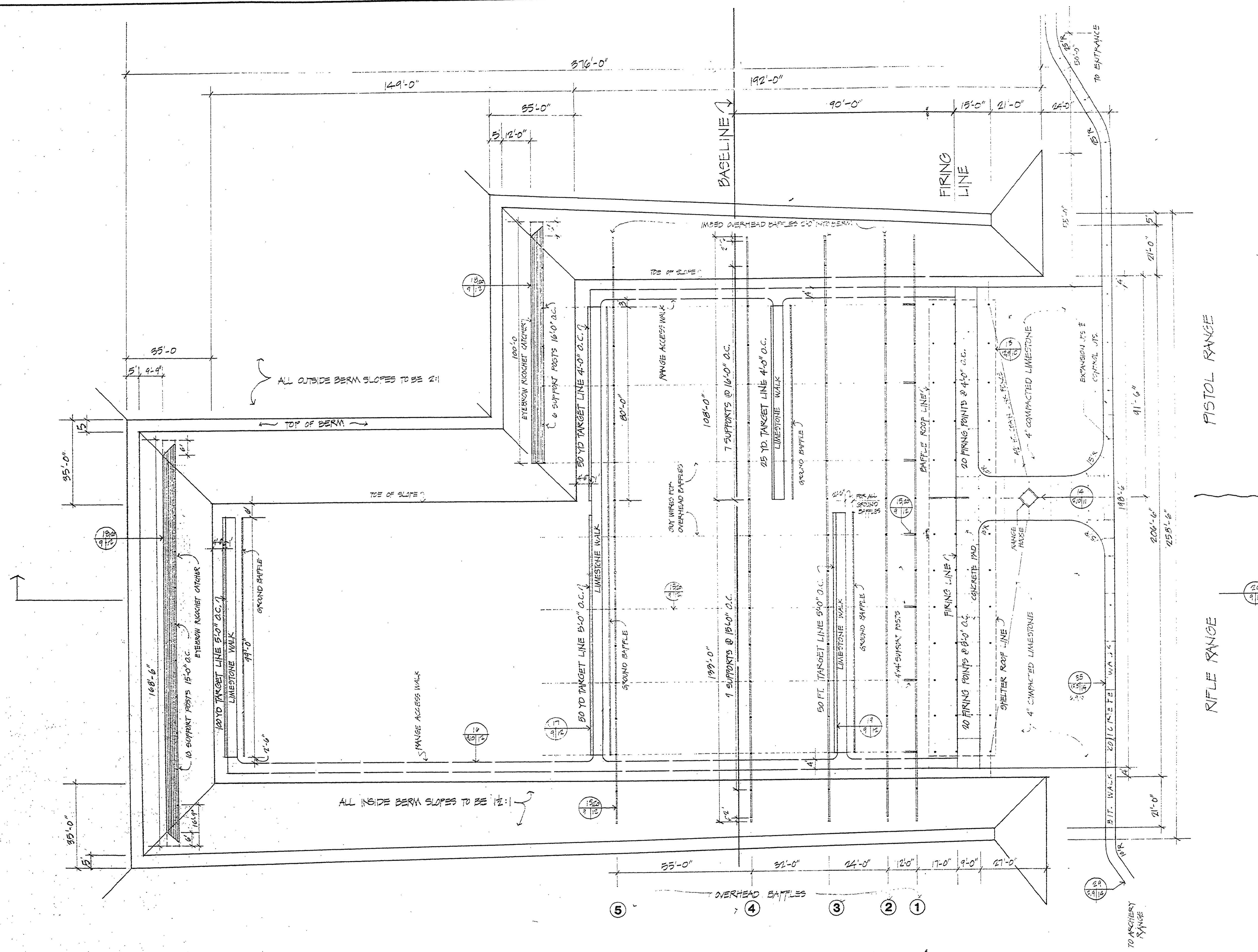
12 13 RIFLE/PISTOL RANGE LAYOUT SCALE 1"=20'-0"
