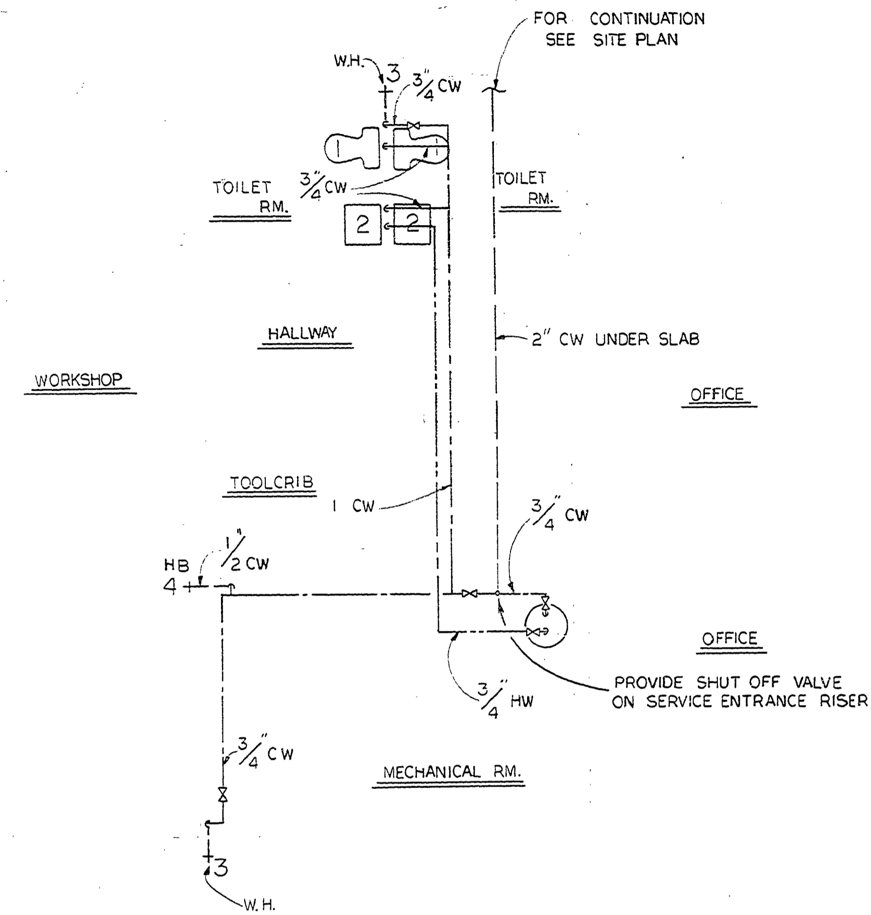
WATER SUPPLY PLAN SCALE 1/4" = 1'-0"
