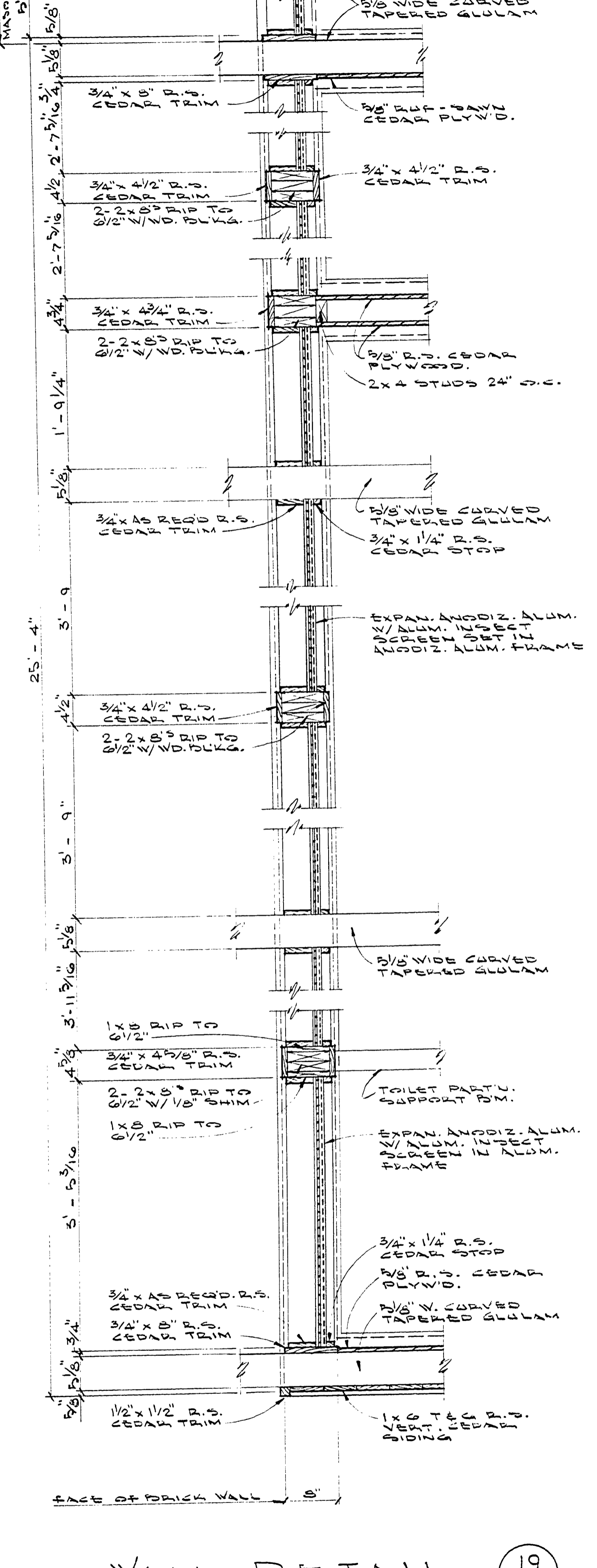
WALL DETAIL 19/46
