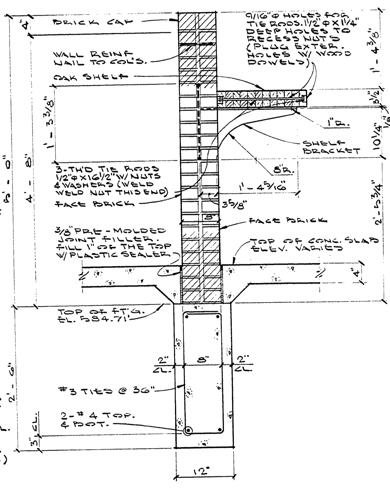
WALL DETAIL 17/36
