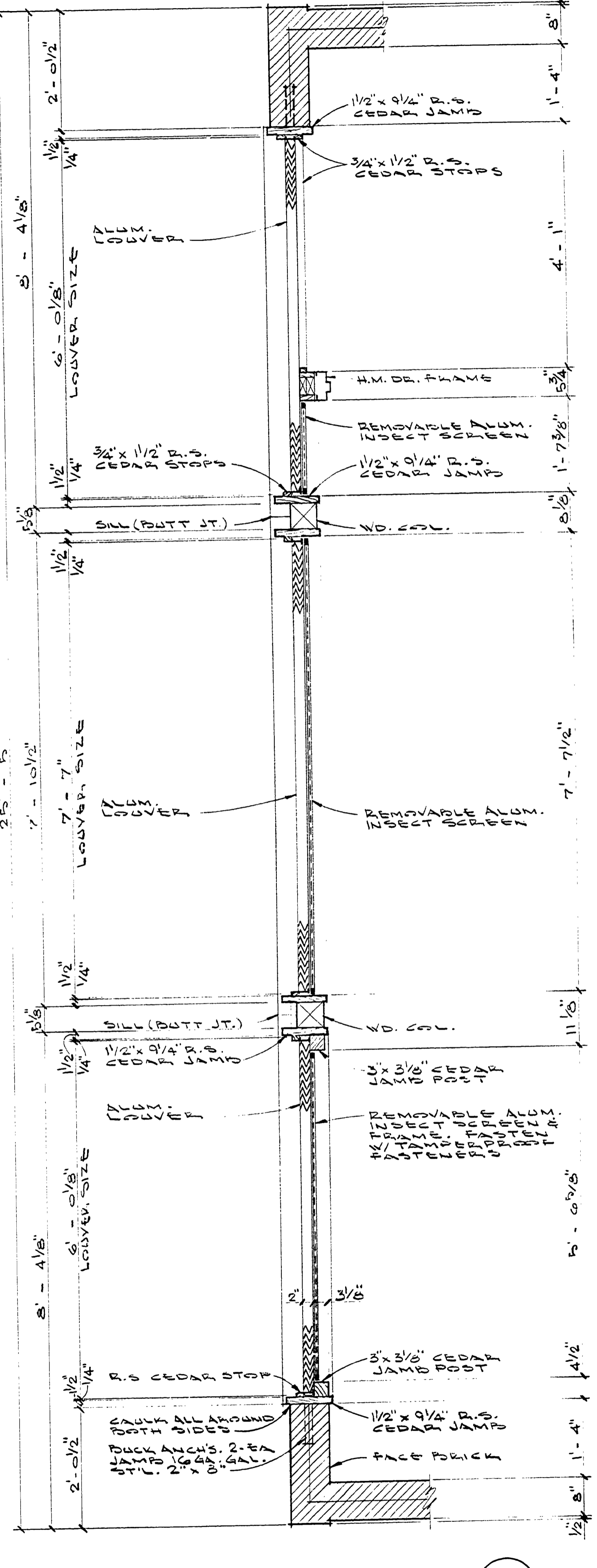
WALL DETAIL 18/46
