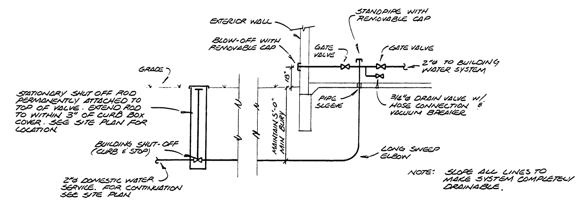
WATER SERVICE ENTRANCE NO SCALE
