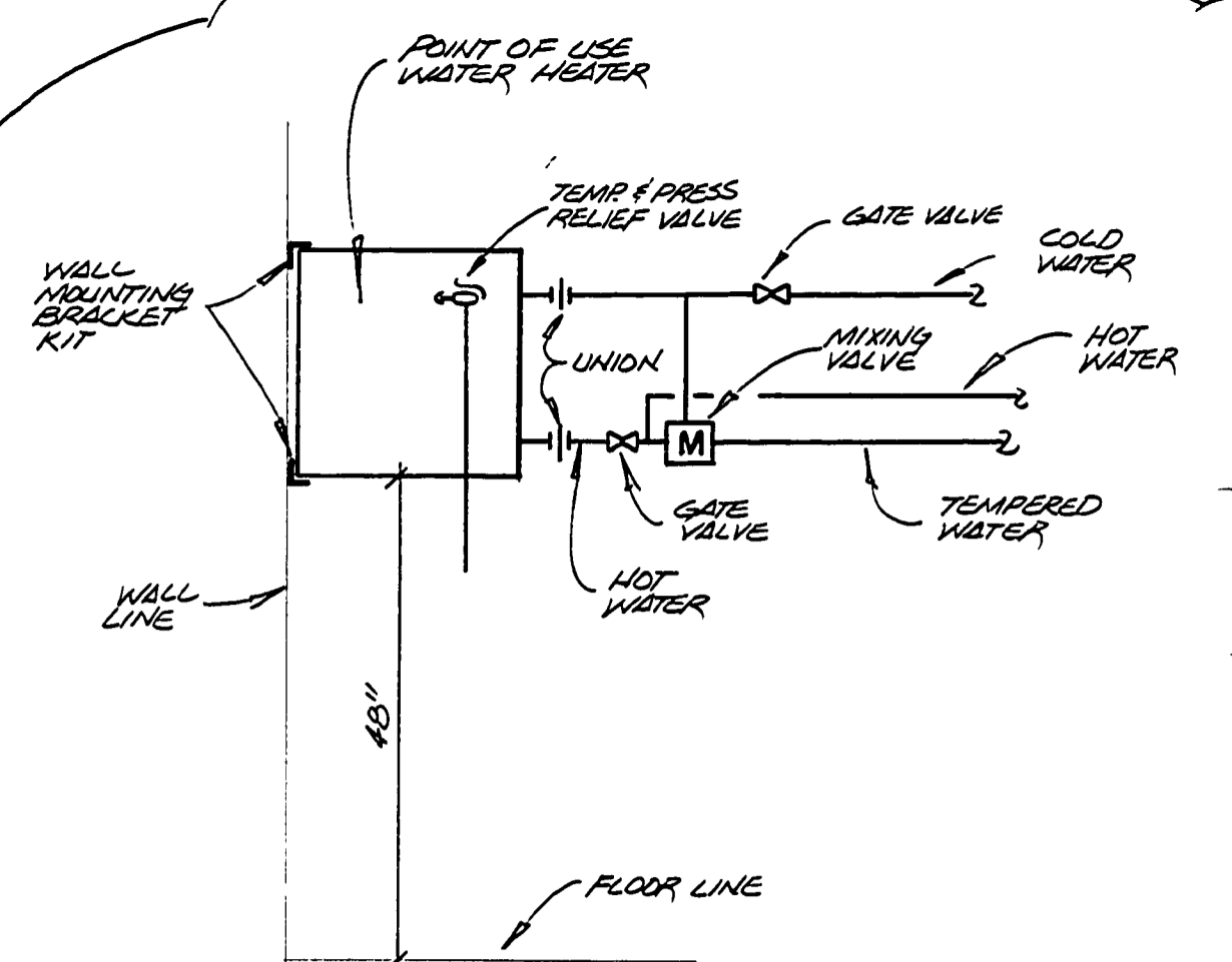
ELECTRIC WATER HEATER DETAIL NOT TO SCALE
