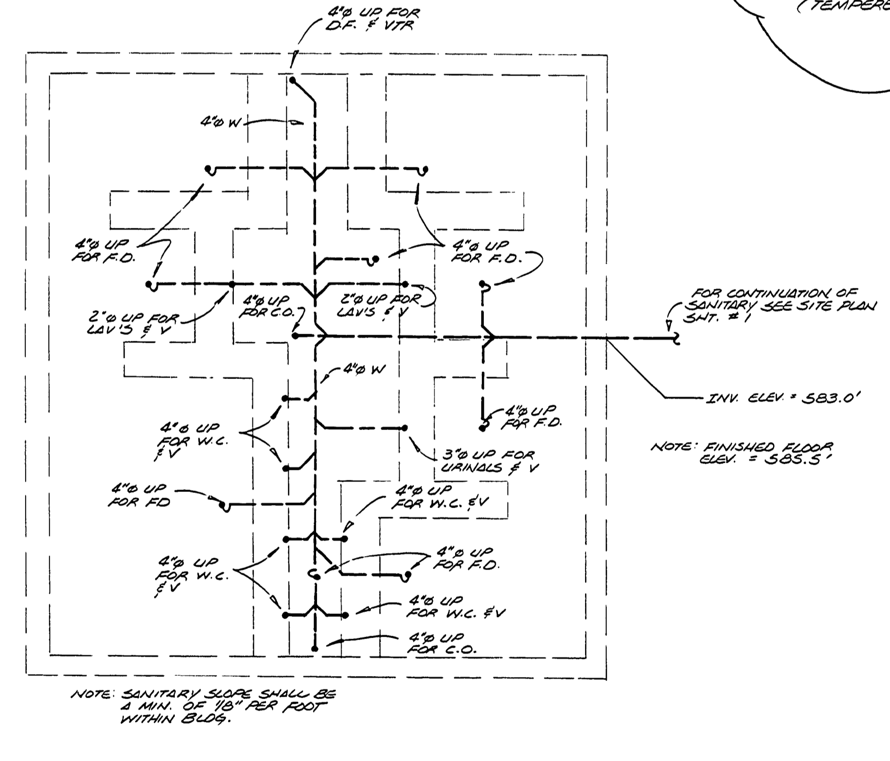
BELOW SLAB WASTE PLUMBING SCALE 1/4" = 1'-0"
