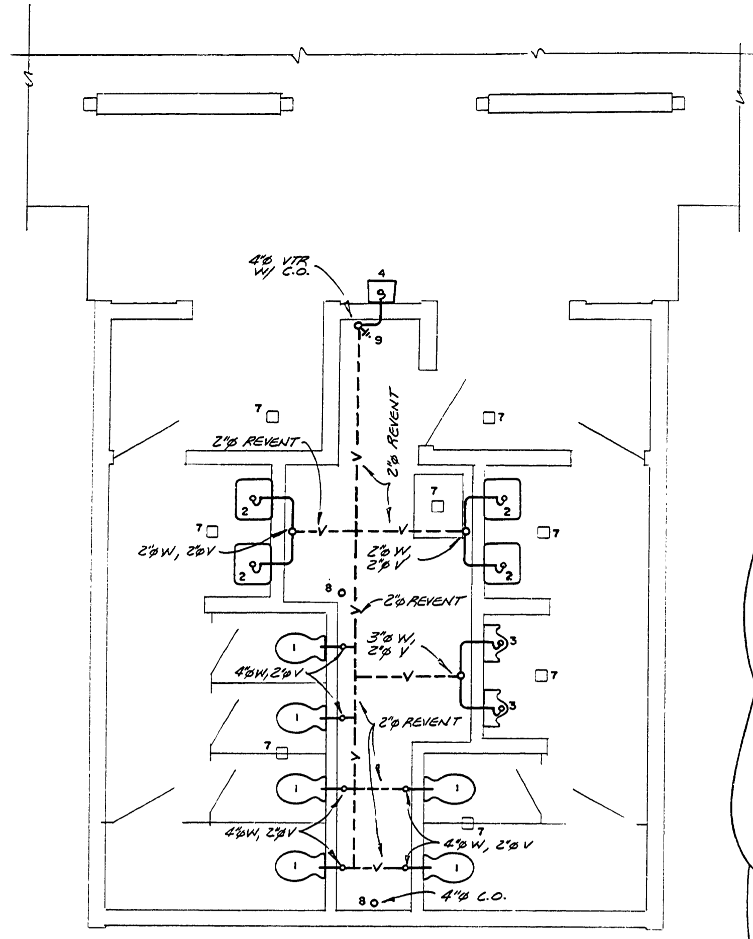
ABOVE SLAB WASTE PLUMBING SCALE 1/4" = 1'-0"
