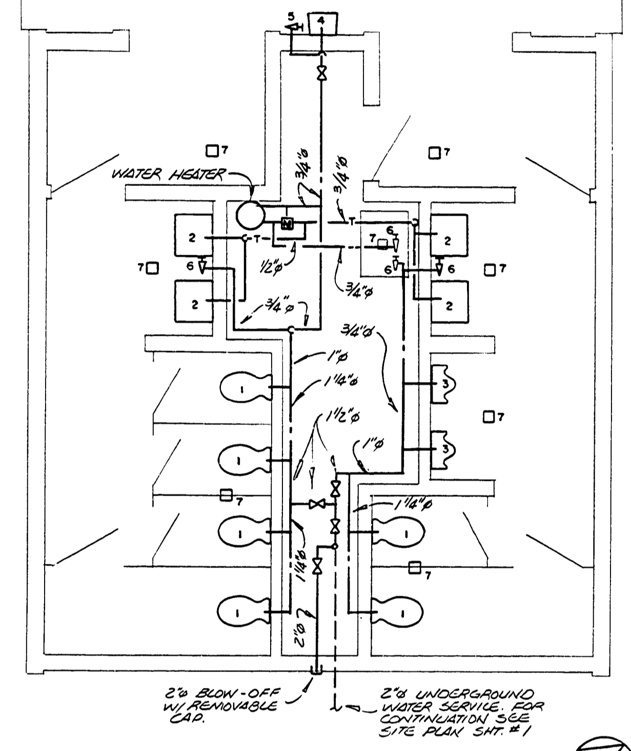
SUPPLY PLUMBING FLOOR PLAN SCALE 1/4" = 1'-0"
